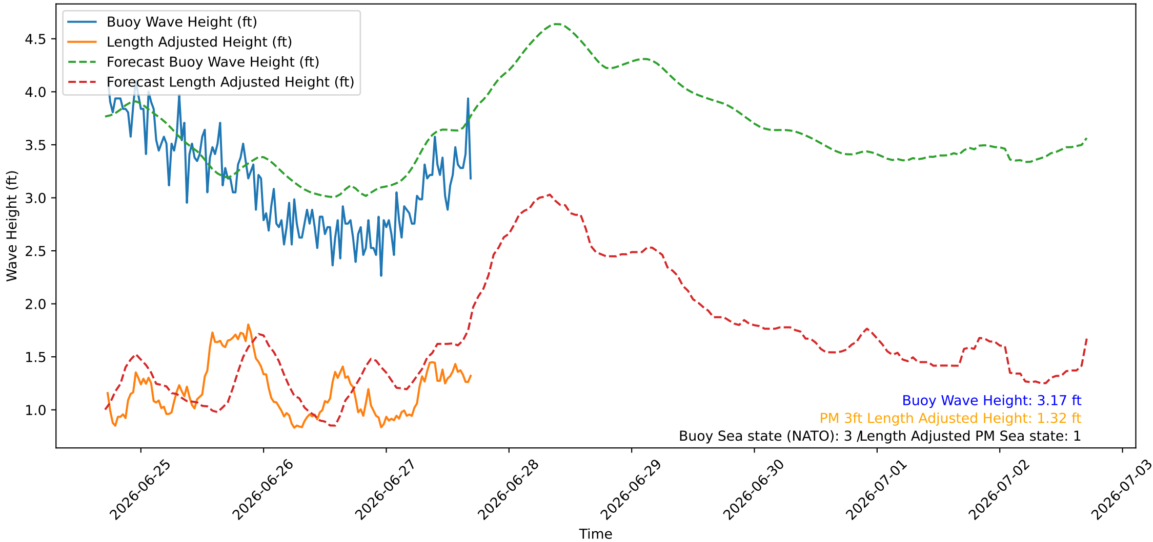
Wave Heights over Time for Green Beach at 2026-06-27 17:21:09
