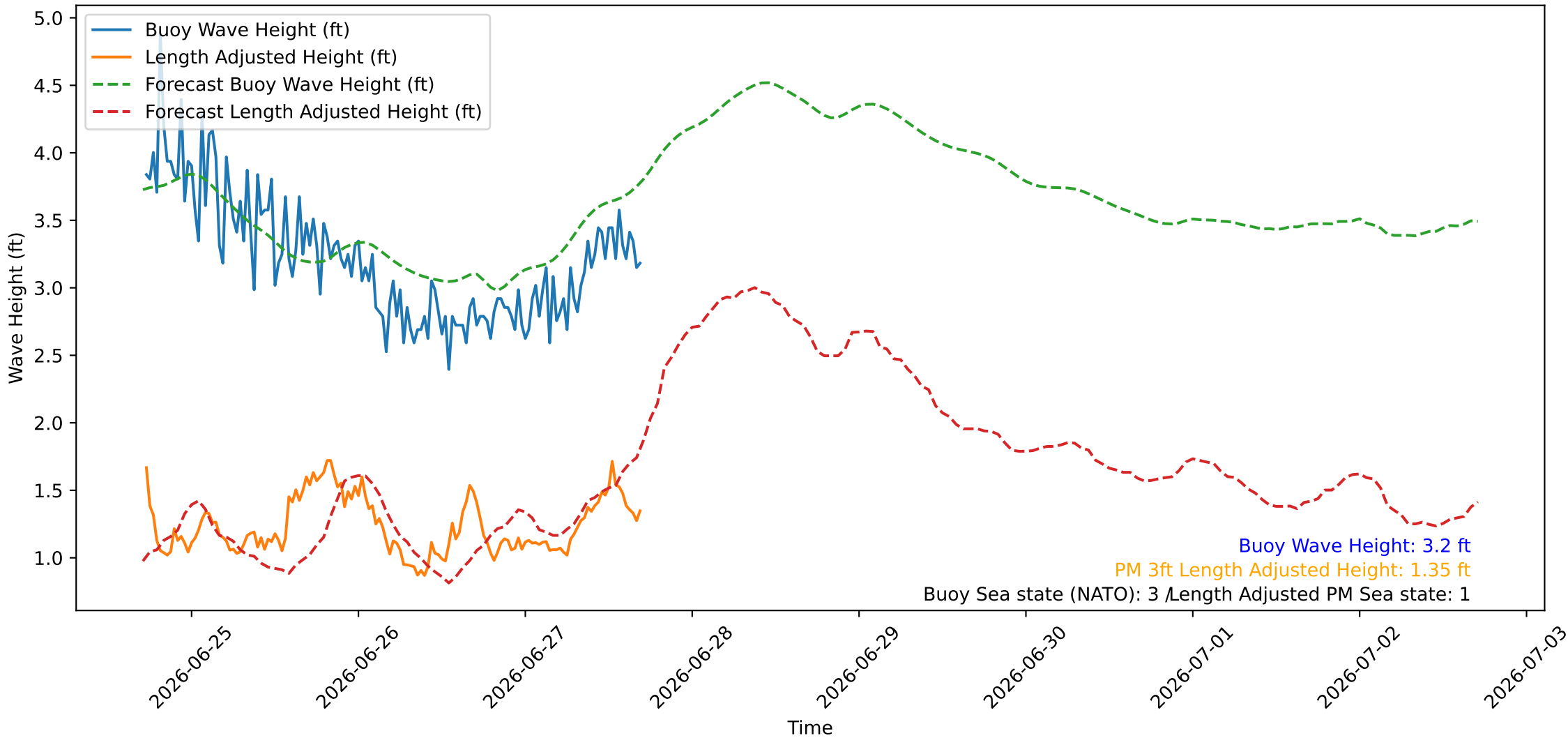
Wave Heights over Time for Oceanside Harbor at 2026-06-27 17:20:26
