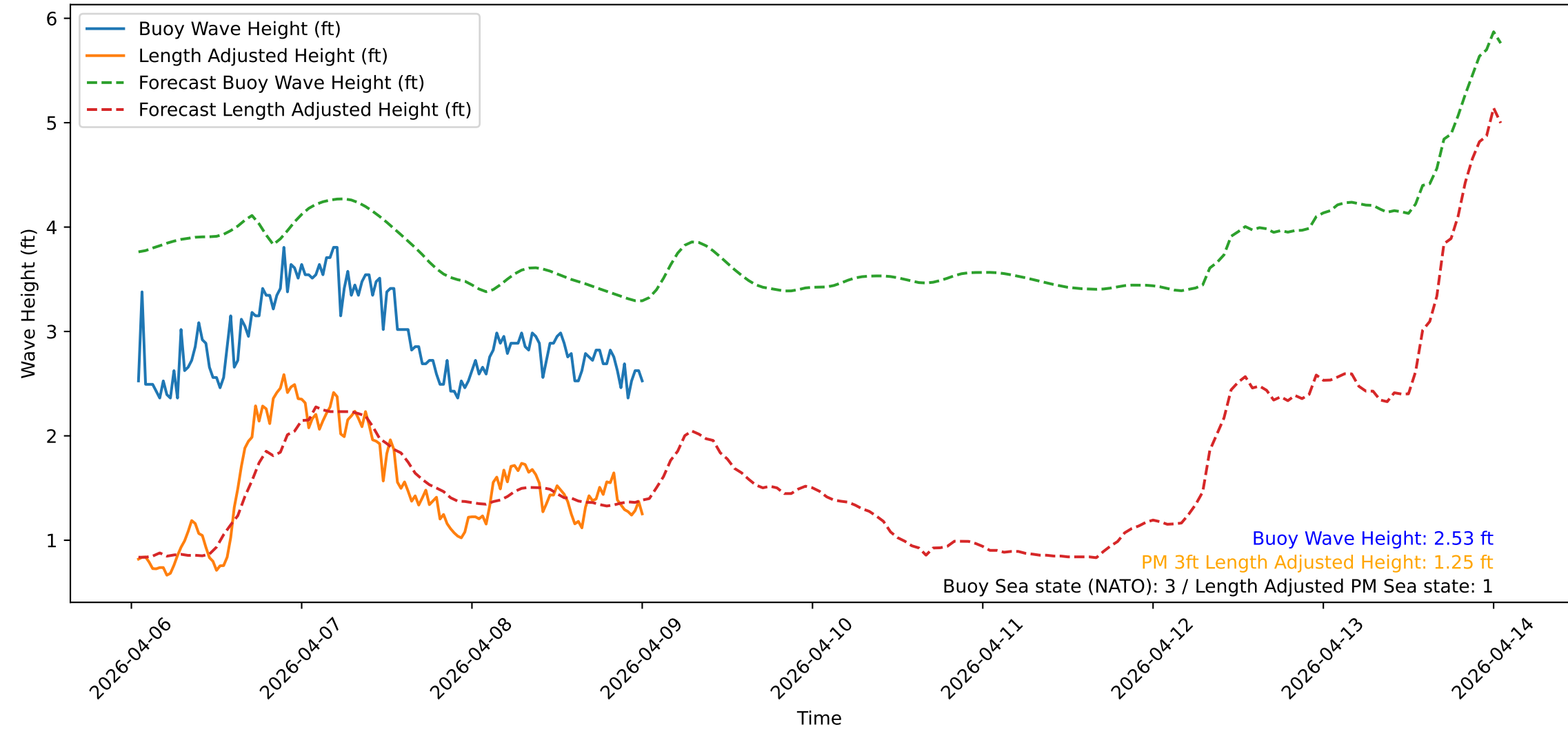
Wave Heights over Time for Green Beach at 2026-04-09 00:51:08
