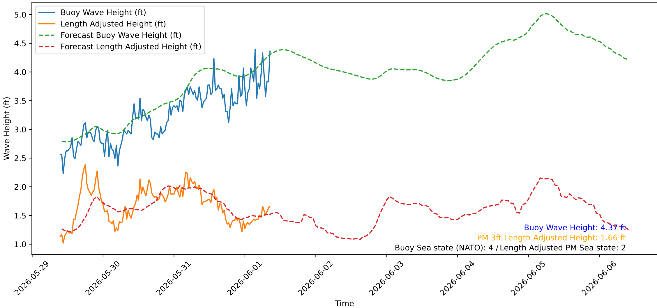
Wave Heights over Time for Oceanside Harbor at 2026-06-01 09:30:26
