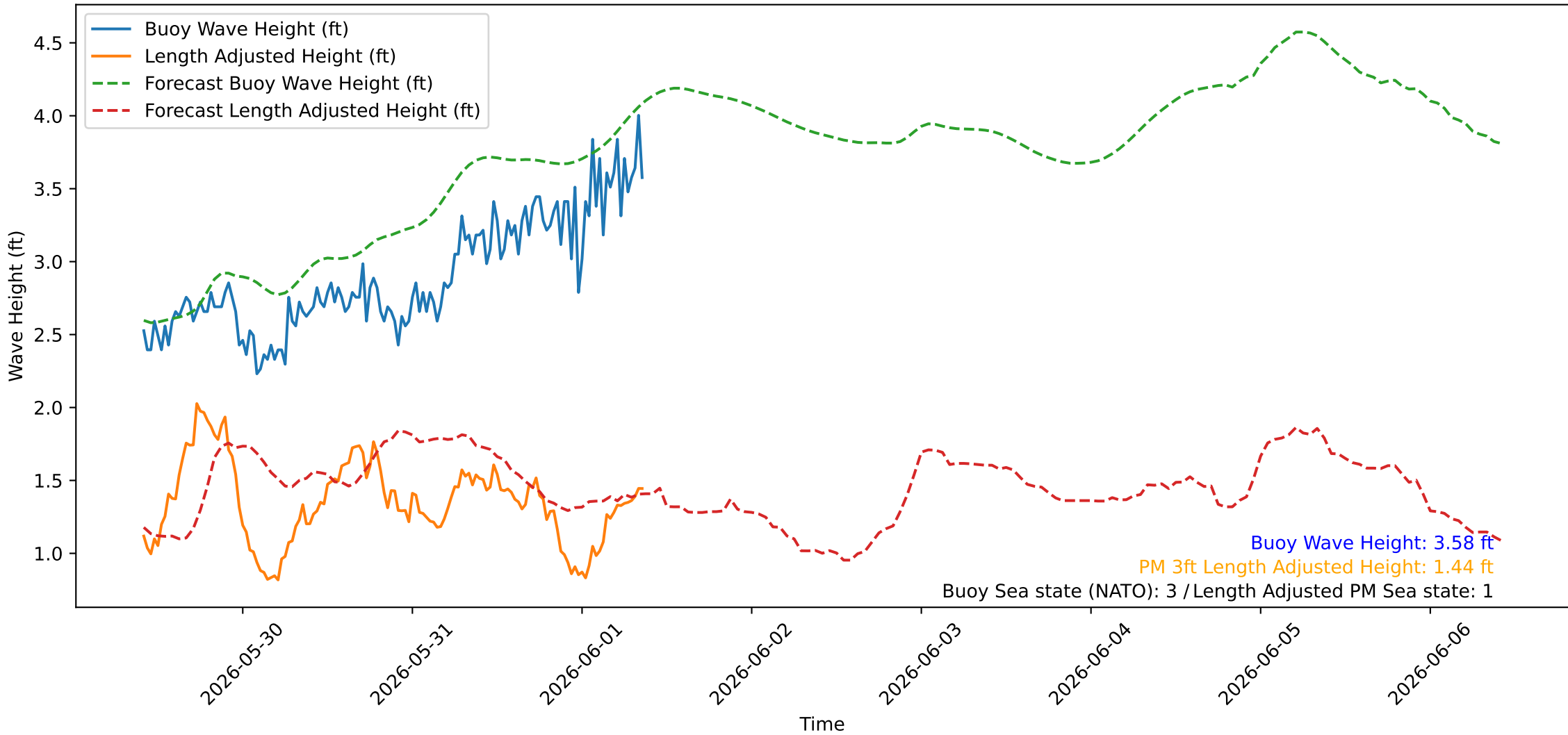
Wave Heights over Time for Red Beach at 2026-06-01 09:30:45
