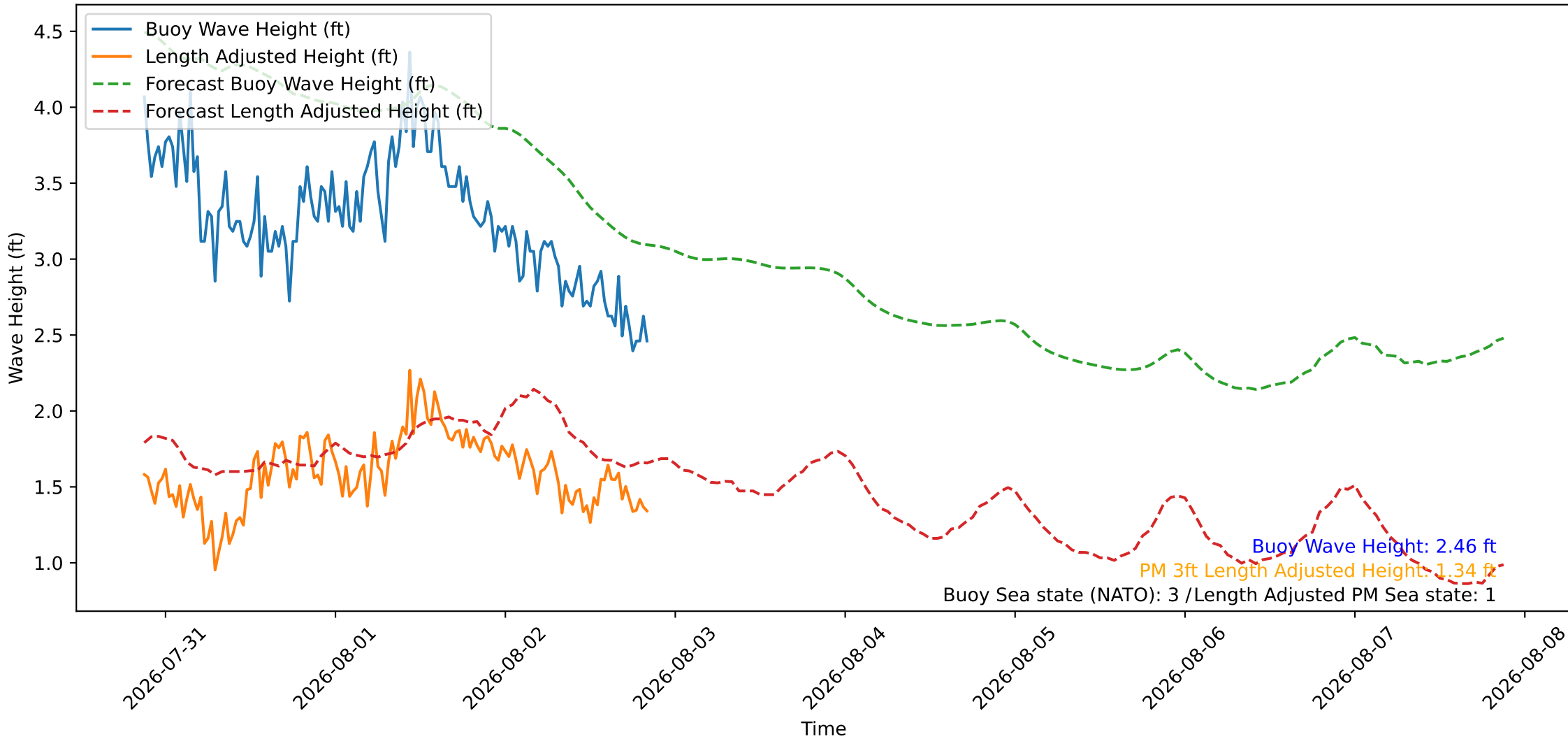
Wave Heights over Time for Oceanside Harbor at 2026-08-02 21:00:26
