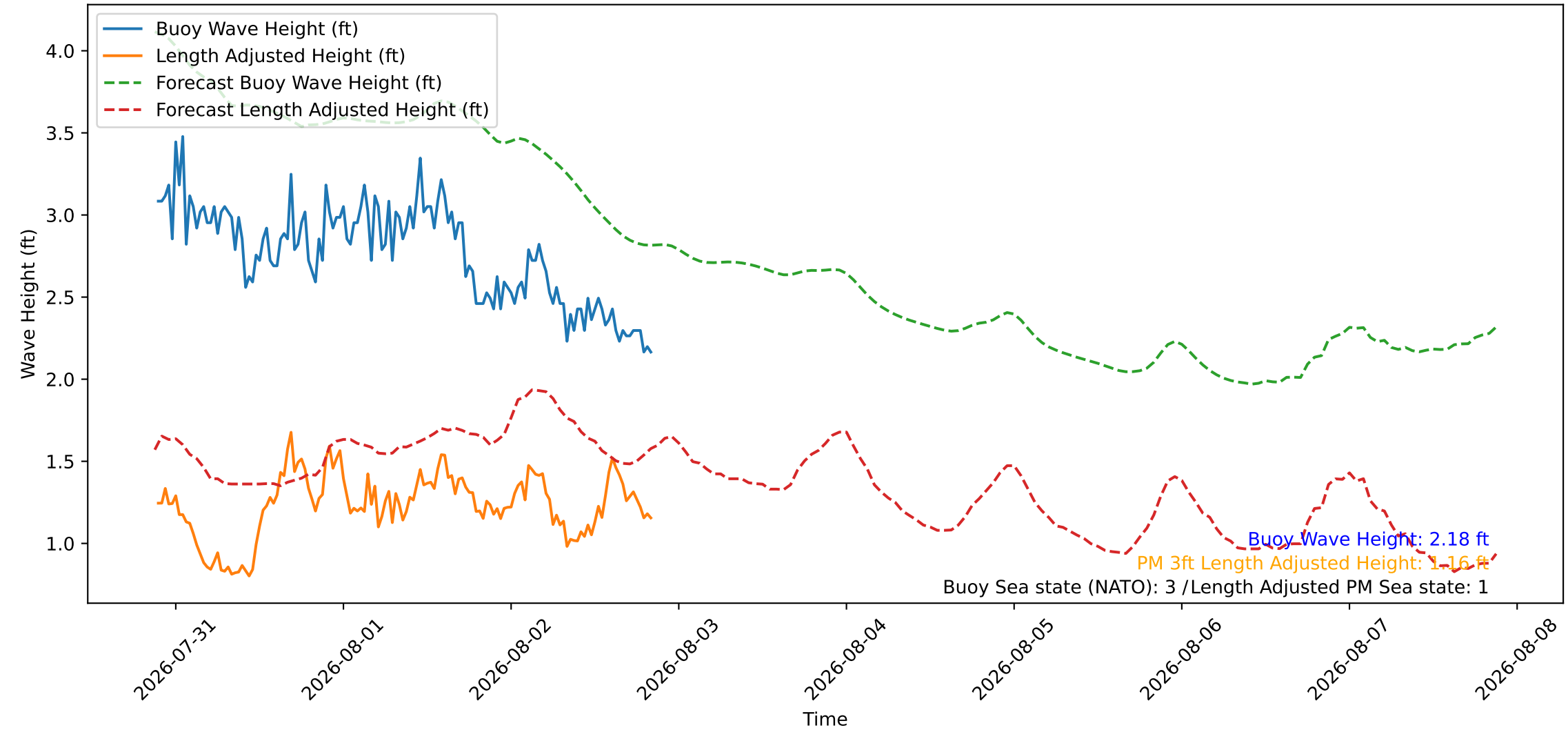
Wave Heights over Time for Red Beach at 2026-08-02 21:00:45
