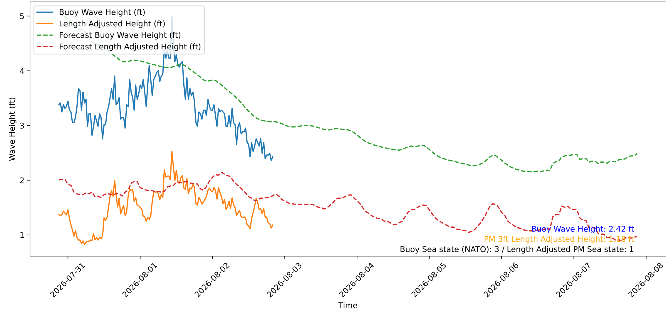
Wave Heights over Time for Green Beach at 2026-08-02 21:01:08
