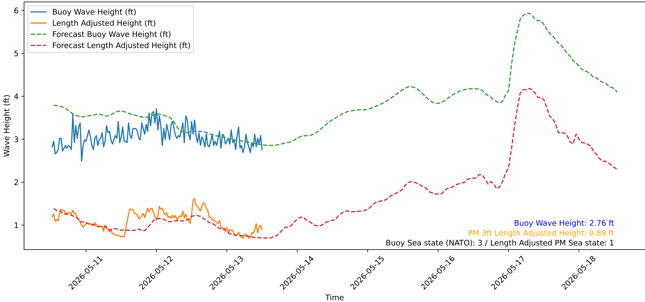
Wave Heights over Time for Oceanside Harbor at 2026-05-13 12:40:32
