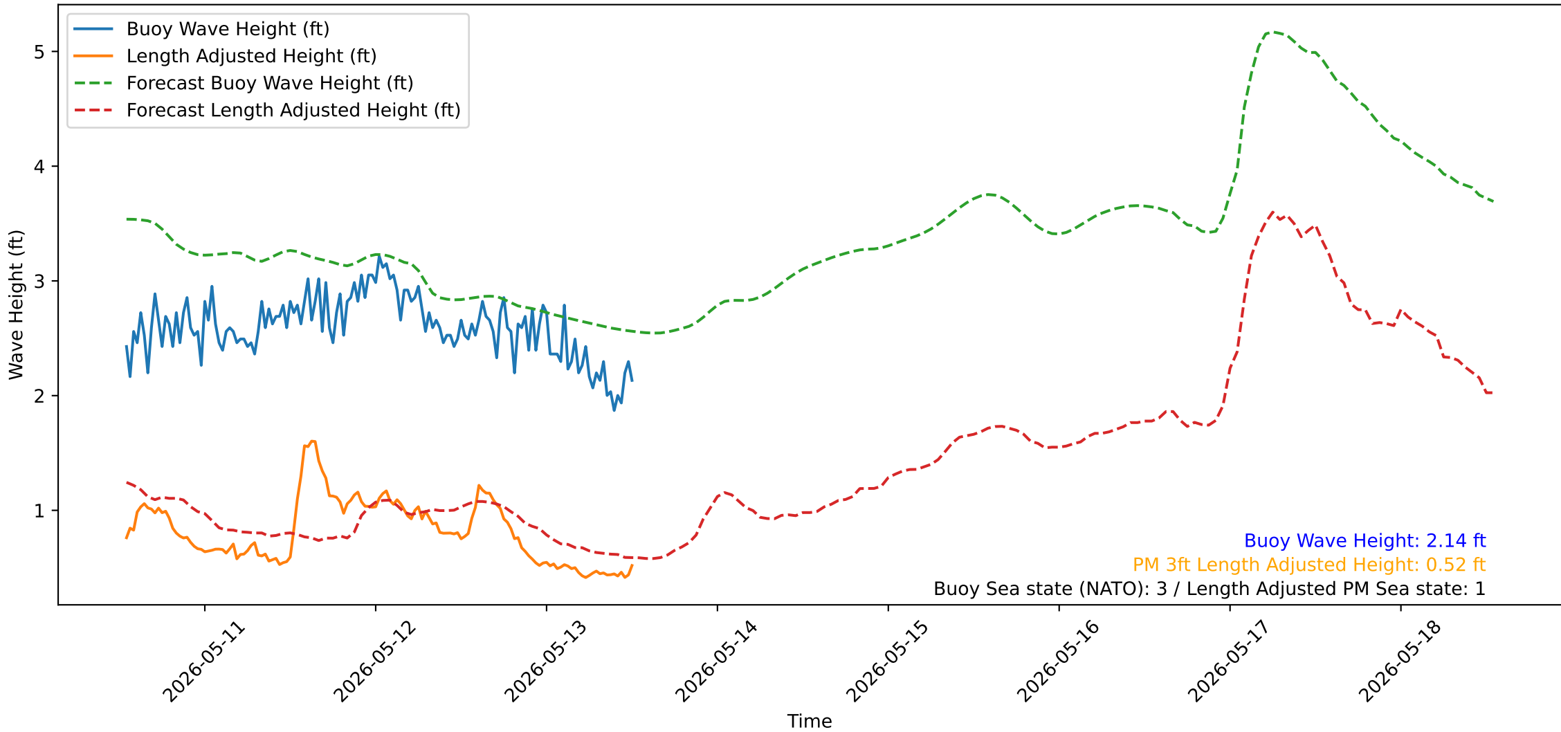
Wave Heights over Time for Red Beach at 2026-05-13 12:40:51
