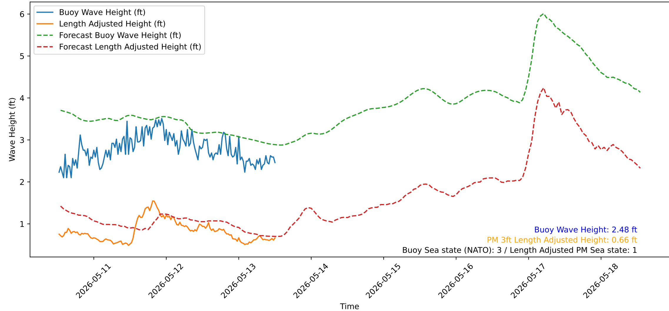
Wave Heights over Time for Green Beach at 2026-05-13 12:41:14
