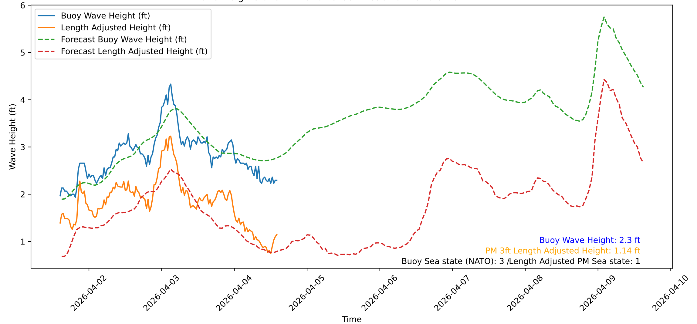
Wave Heights over Time for Green Beach at 2026-04-04 14:41:12
