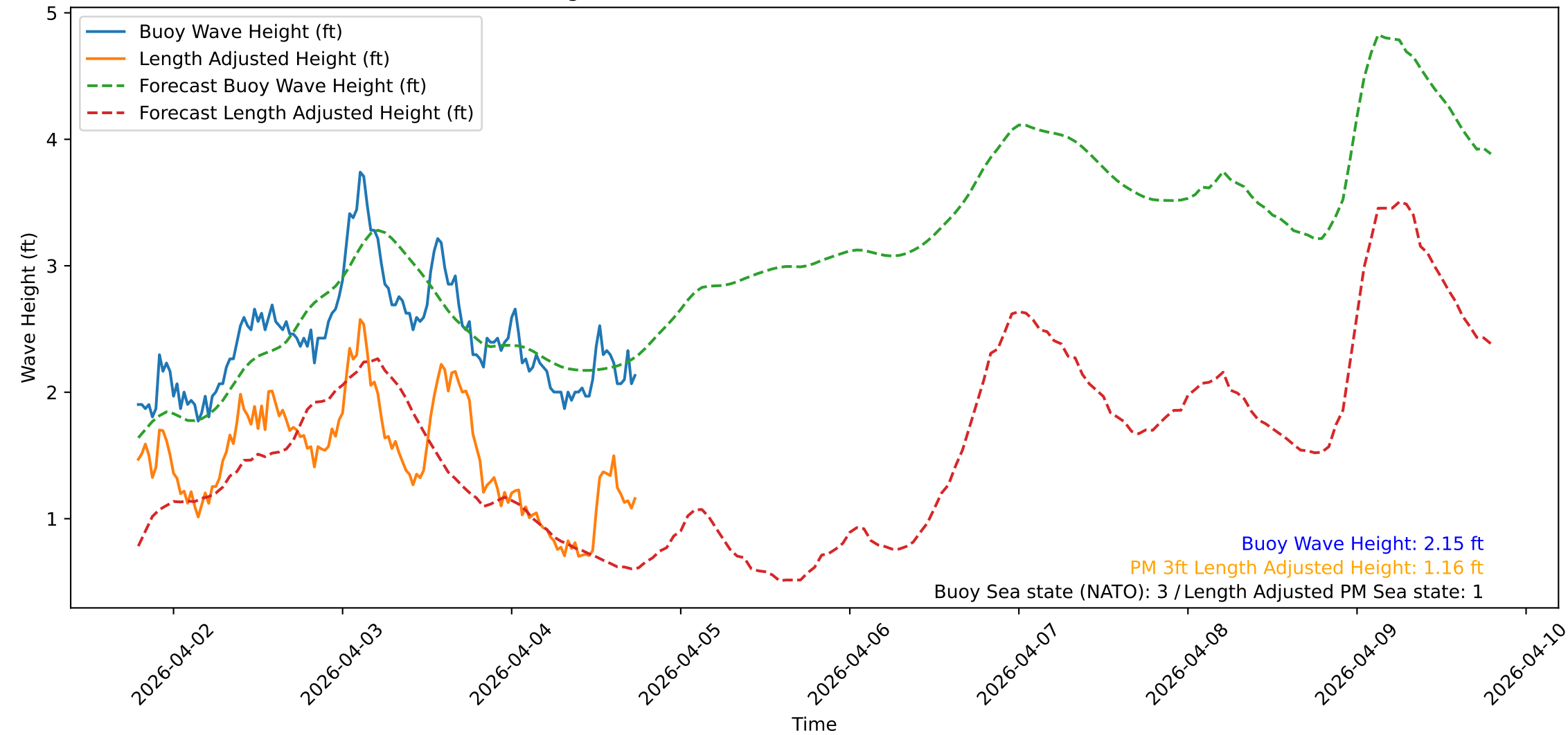
Wave Heights over Time for Red Beach at 2026-04-04 18:40:51
