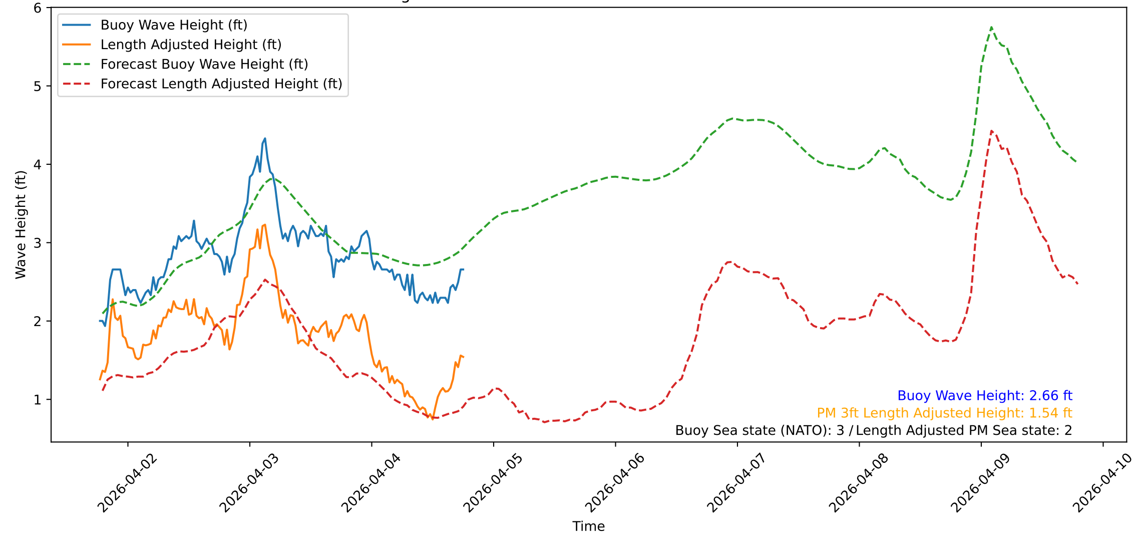
Wave Heights over Time for Green Beach at 2026-04-04 18:41:16
