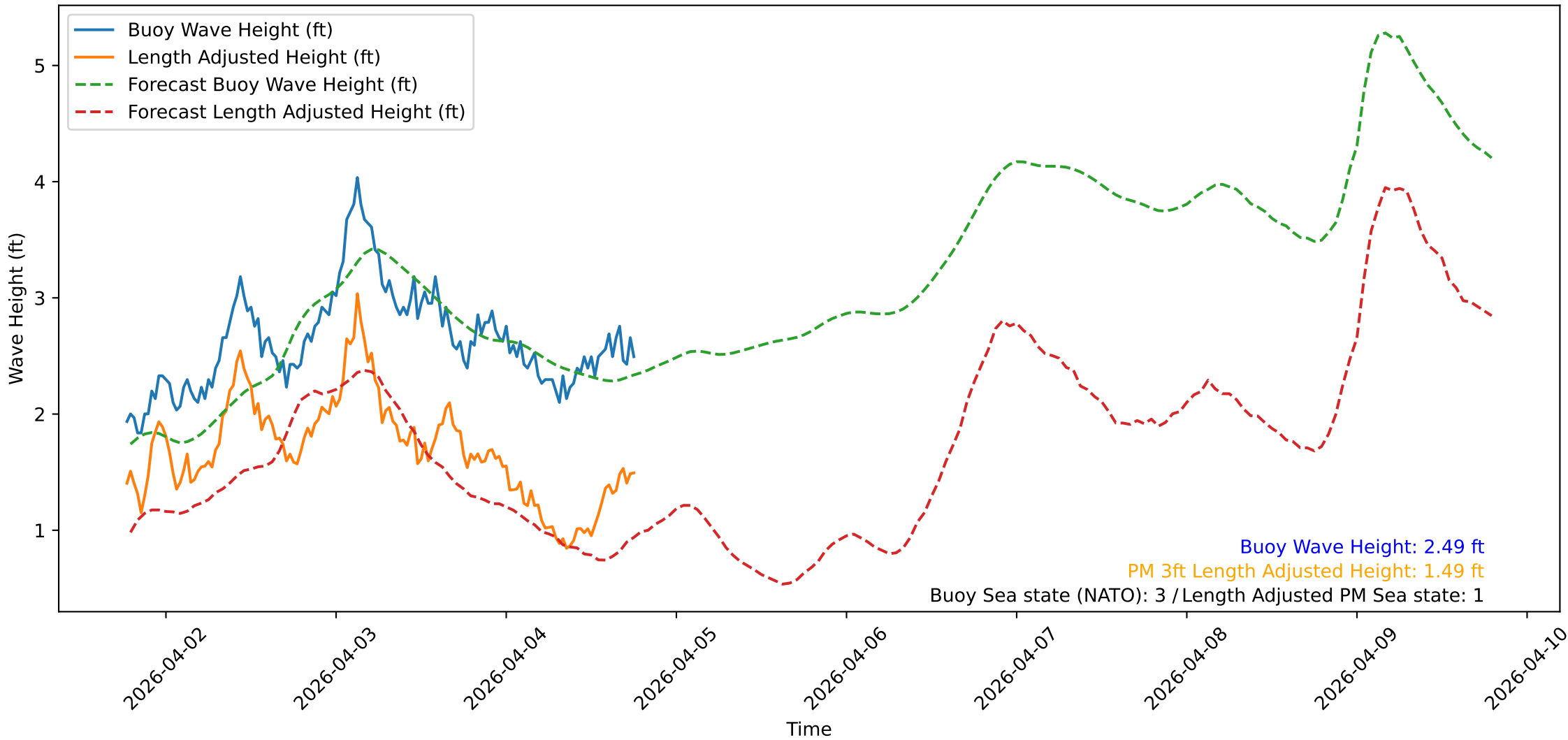
Wave Heights over Time for Oceanside Harbor at 2026-04-04 18:40:34
