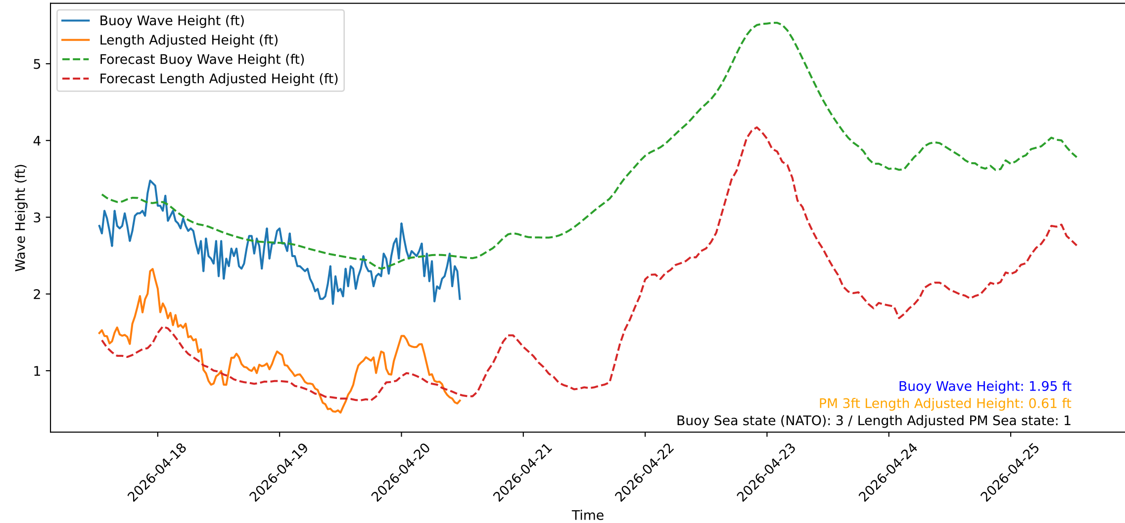
Wave Heights over Time for Green Beach at 2026-04-20 12:31:14
