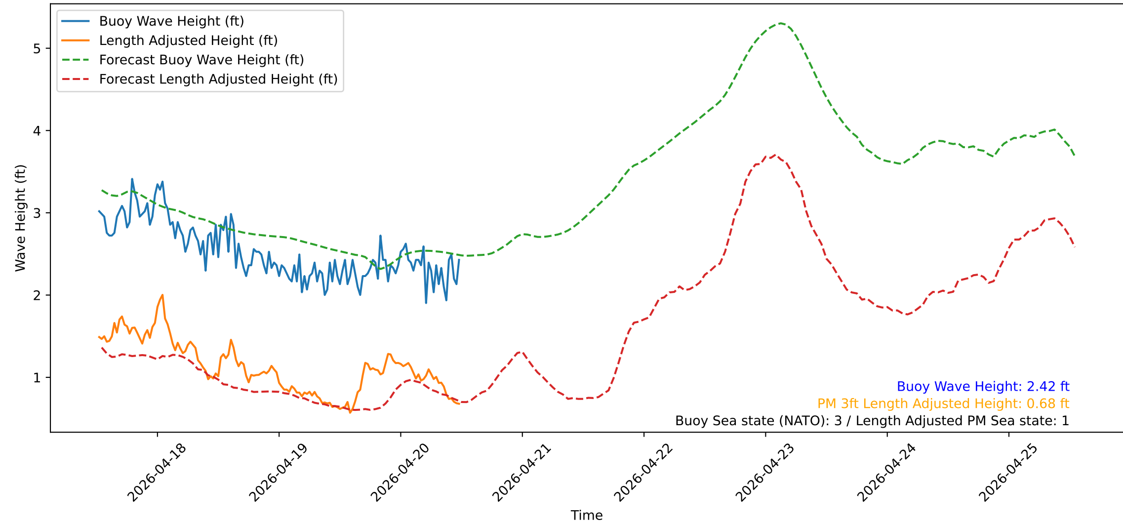
Wave Heights over Time for Oceanside Harbor at 2026-04-20 12:30:32
