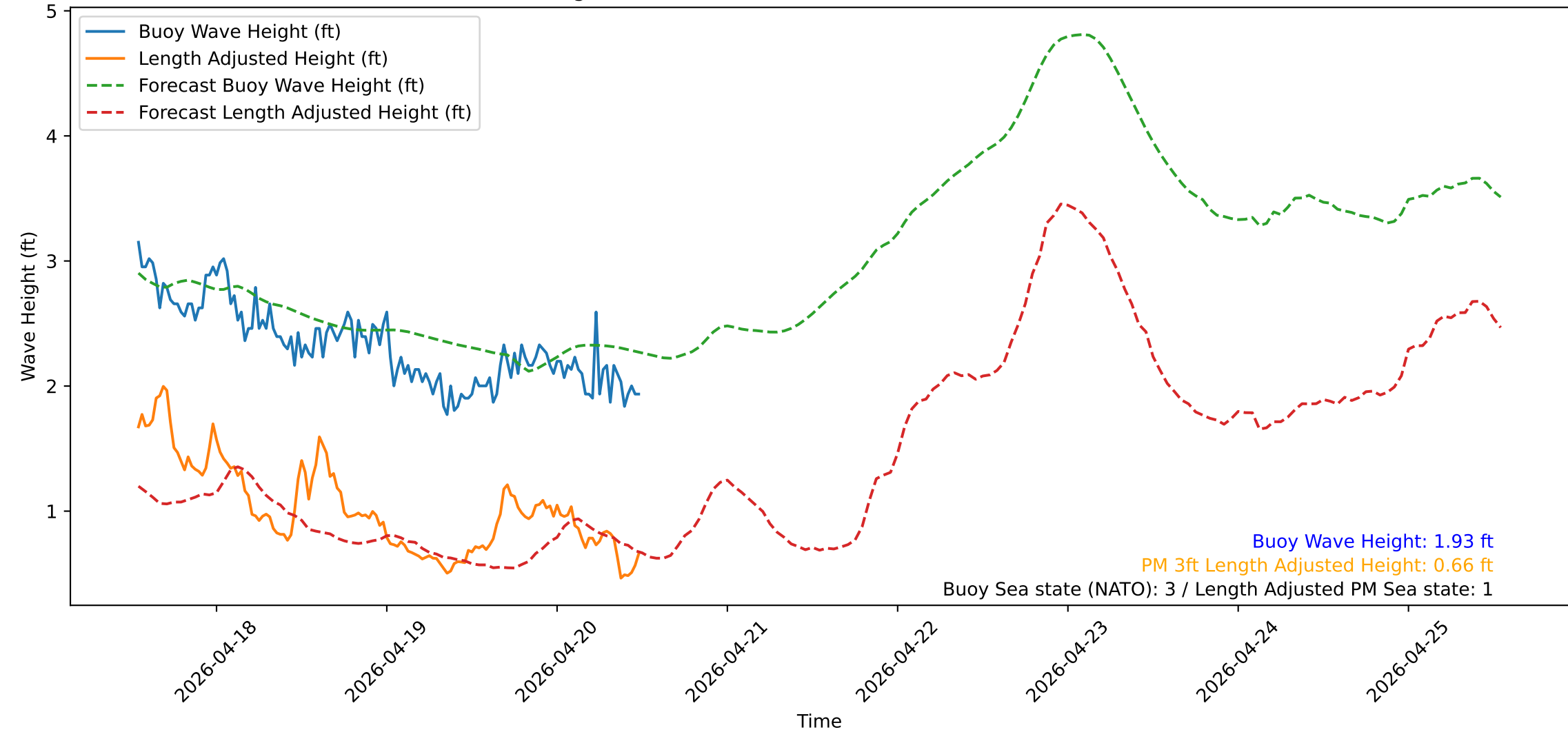
Wave Heights over Time for Red Beach at 2026-04-20 12:30:51
