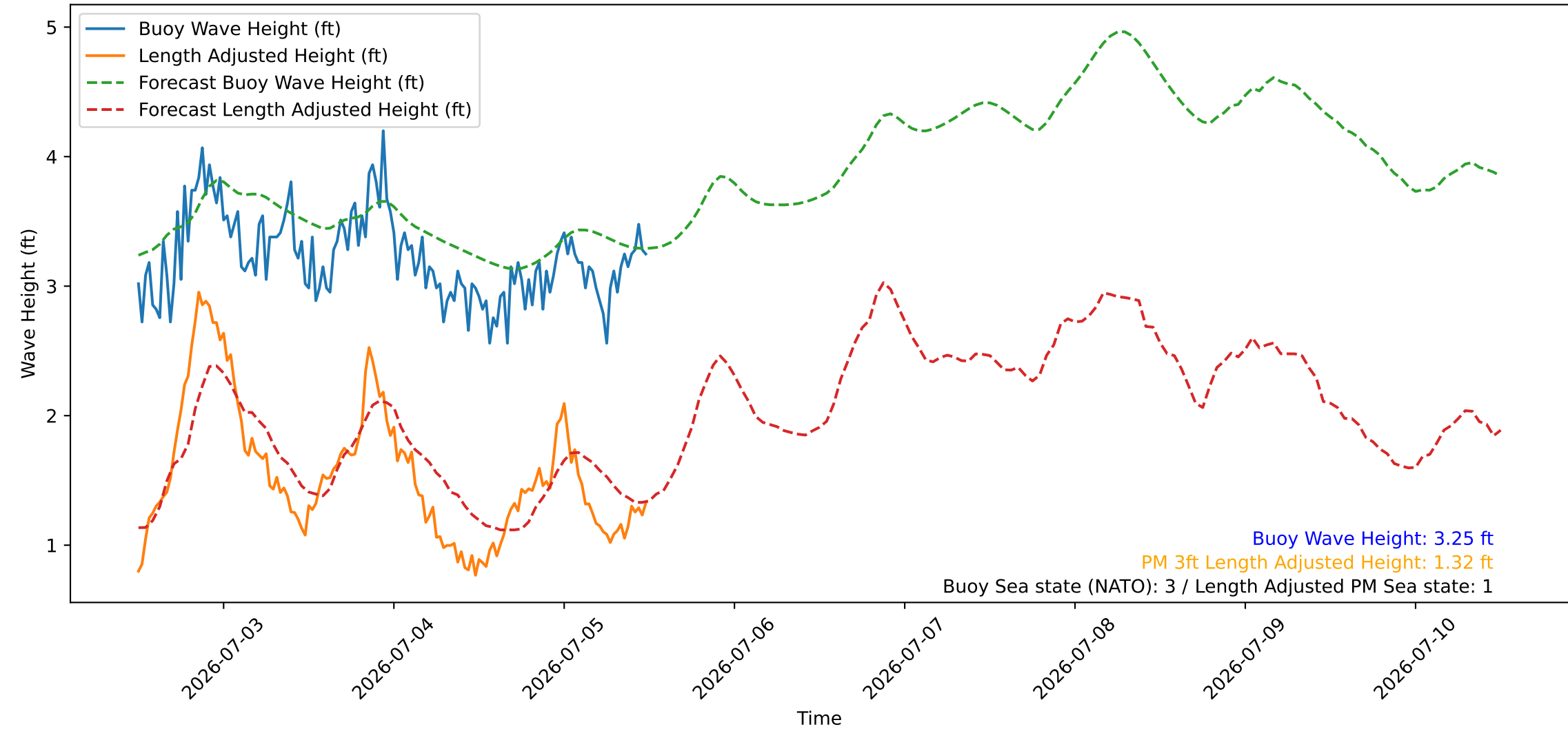
Wave Heights over Time for Green Beach at 2026-07-05 12:11:08
