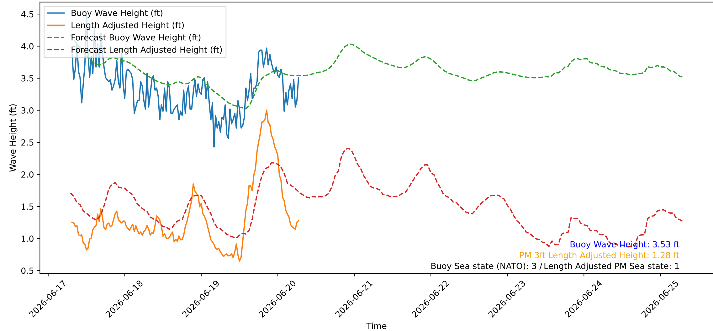
Wave Heights over Time for Green Beach at 2026-06-20 07:21:09
