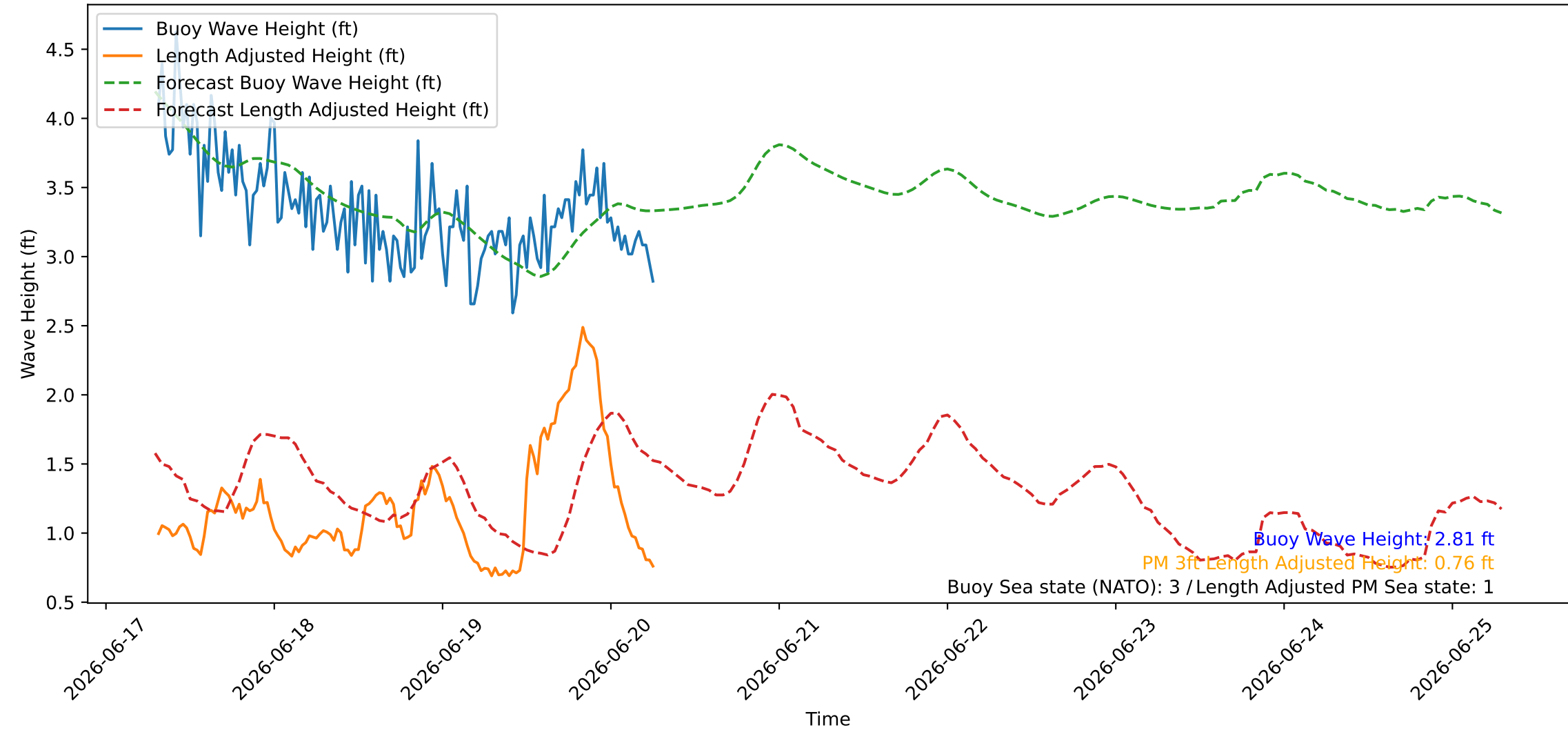
Wave Heights over Time for Red Beach at 2026-06-20 07:20:47
