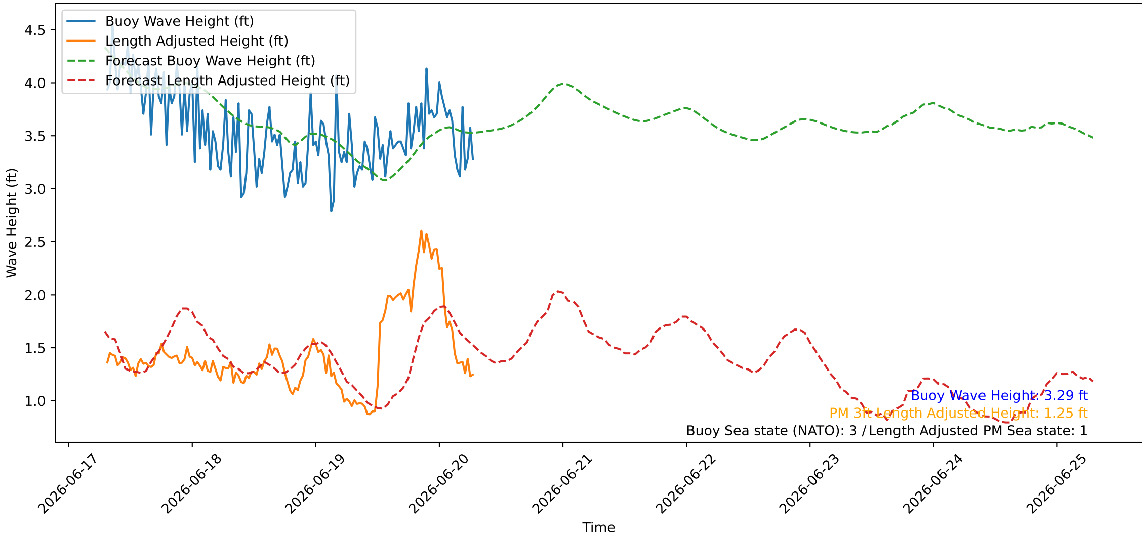
Wave Heights over Time for Oceanside Harbor at 2026-06-20 07:20:26
