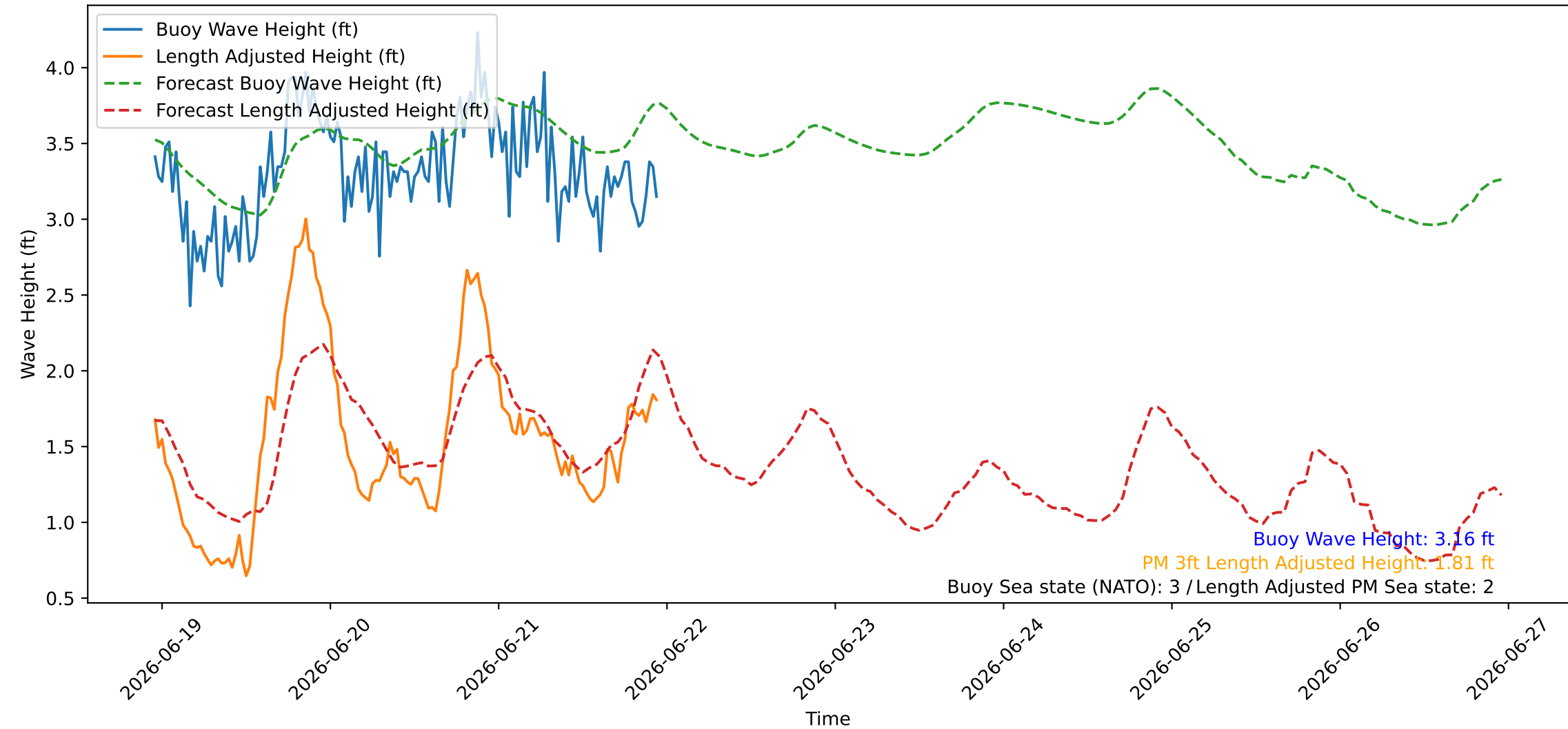
Wave Heights over Time for Green Beach at 2026-06-21 23:11:08
