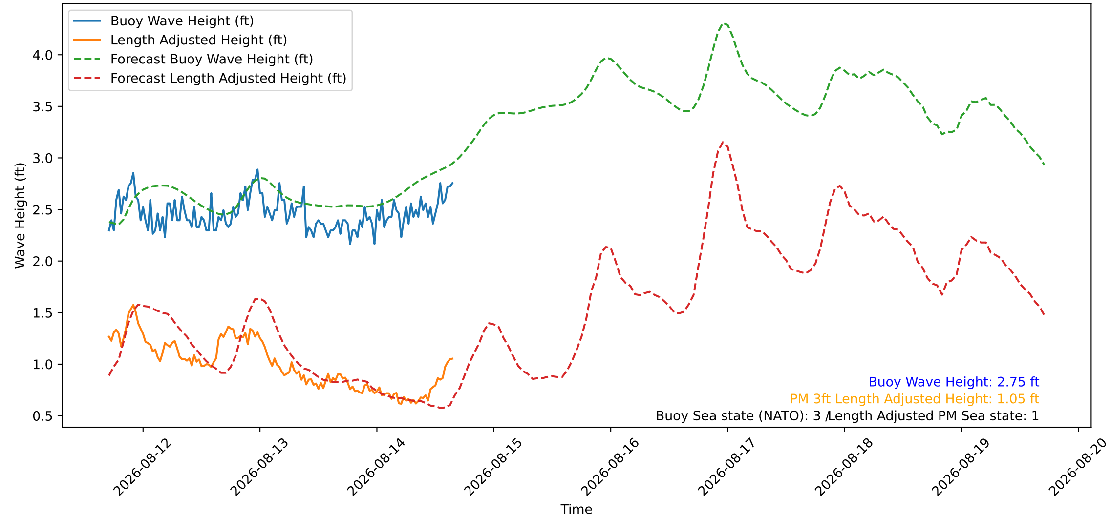
Wave Heights over Time for Red Beach at 2026-08-14 16:40:46
