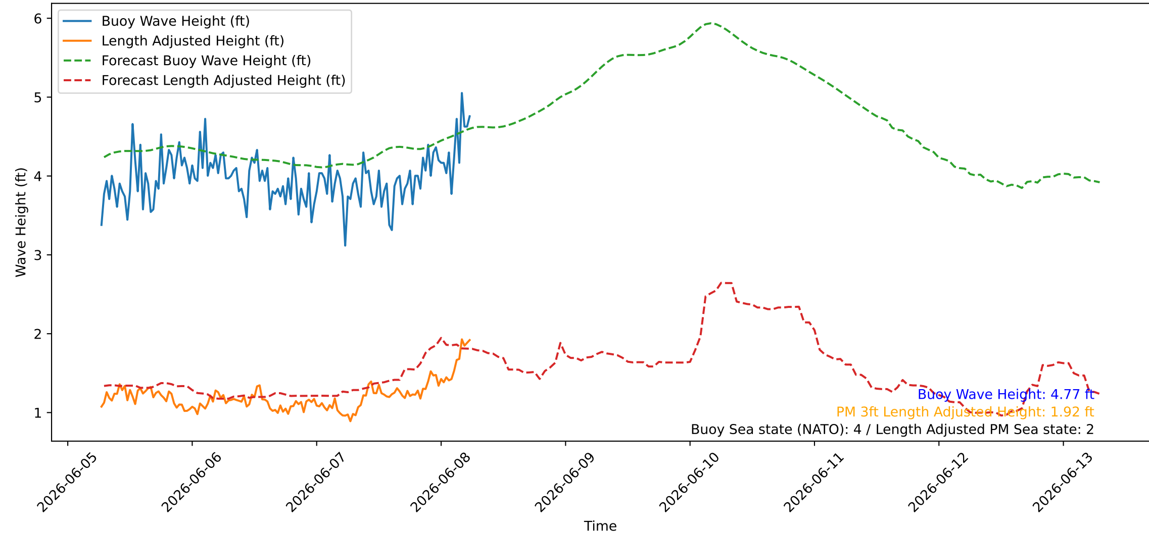
Wave Heights over Time for Green Beach at 2026-06-08 06:31:08
