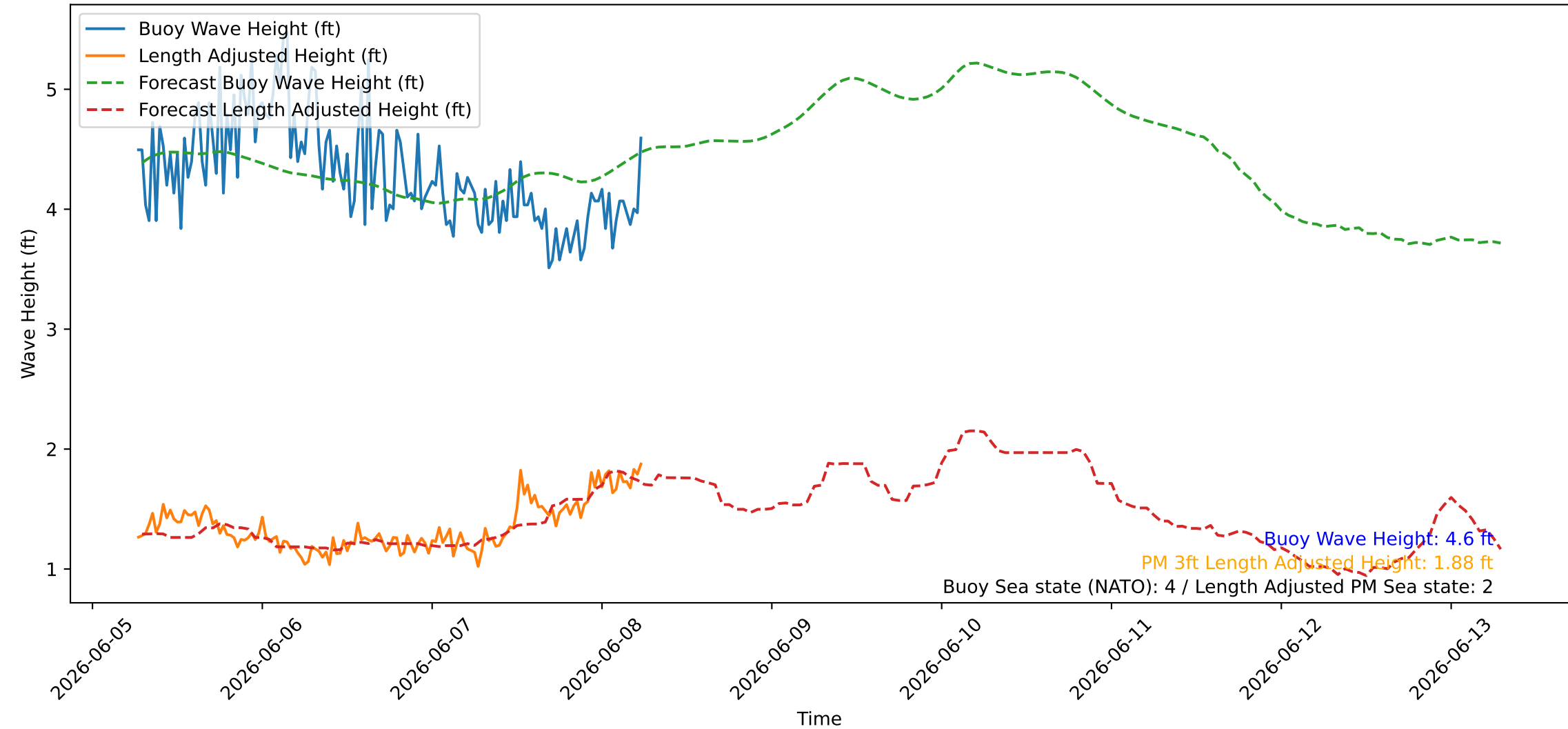
Wave Heights over Time for Oceanside Harbor at 2026-06-08 06:30:26
