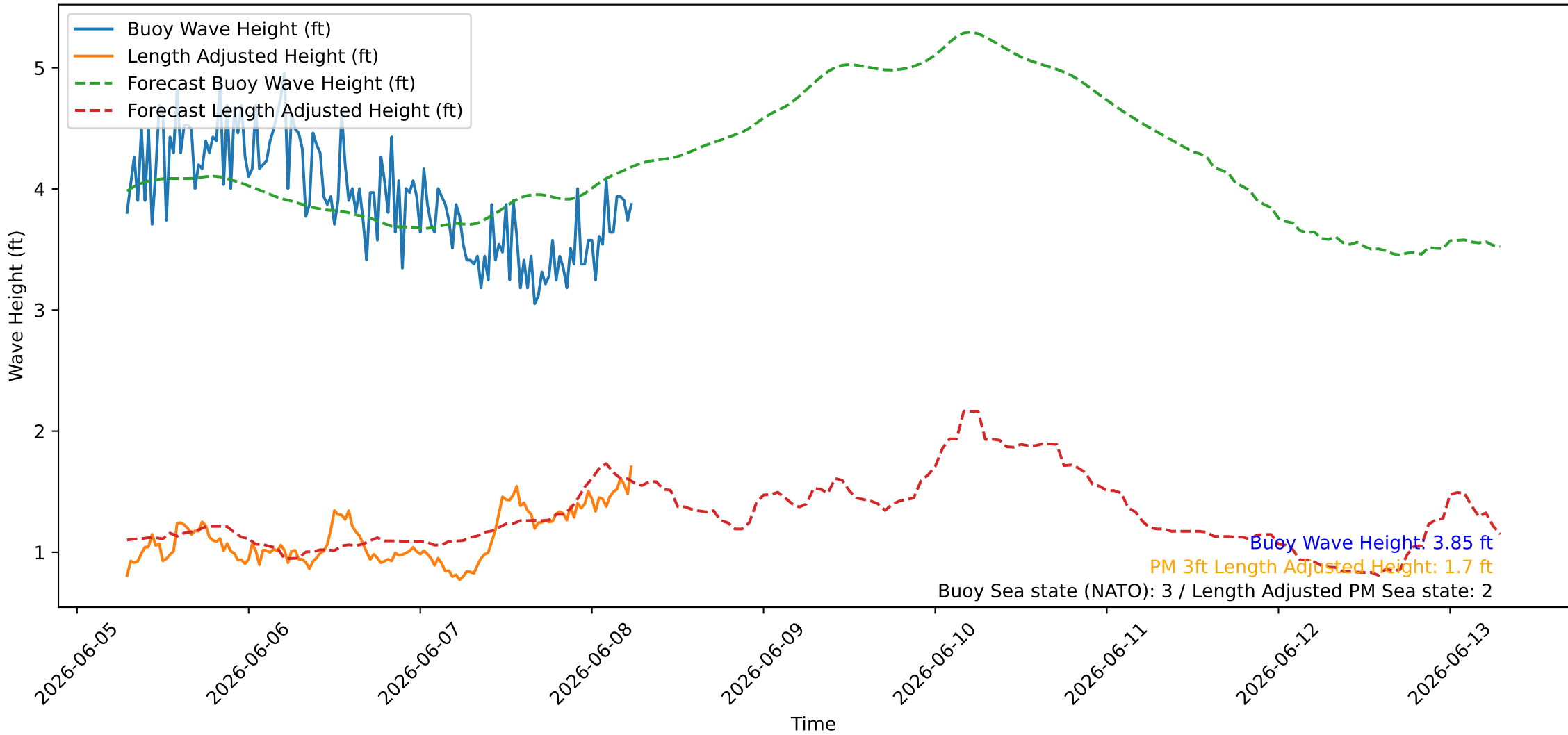
Wave Heights over Time for Red Beach at 2026-06-08 06:30:45
