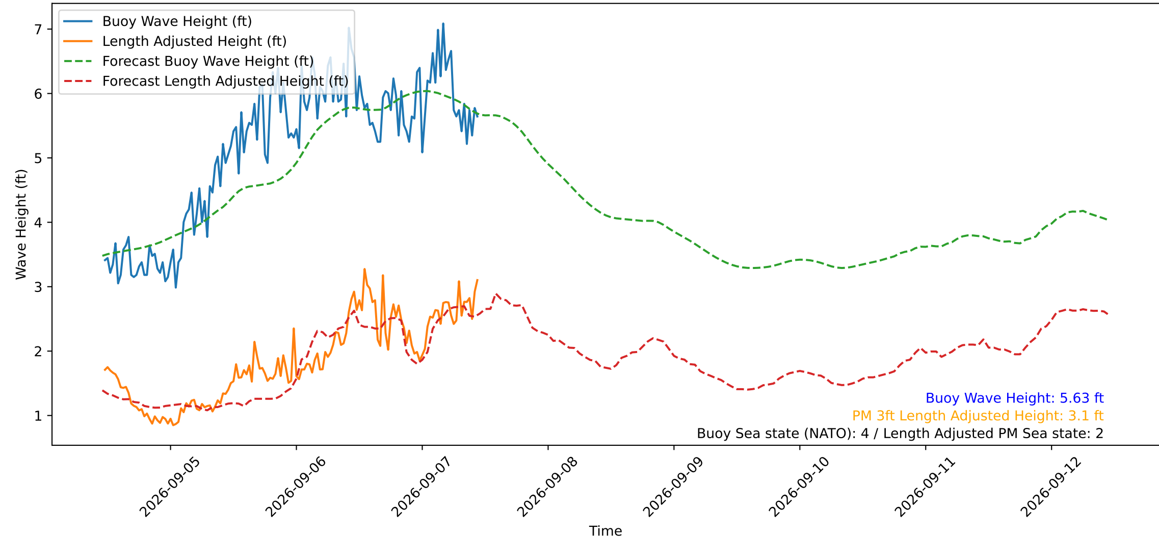
Wave Heights over Time for Oceanside Harbor at 2026-09-07 11:20:30
