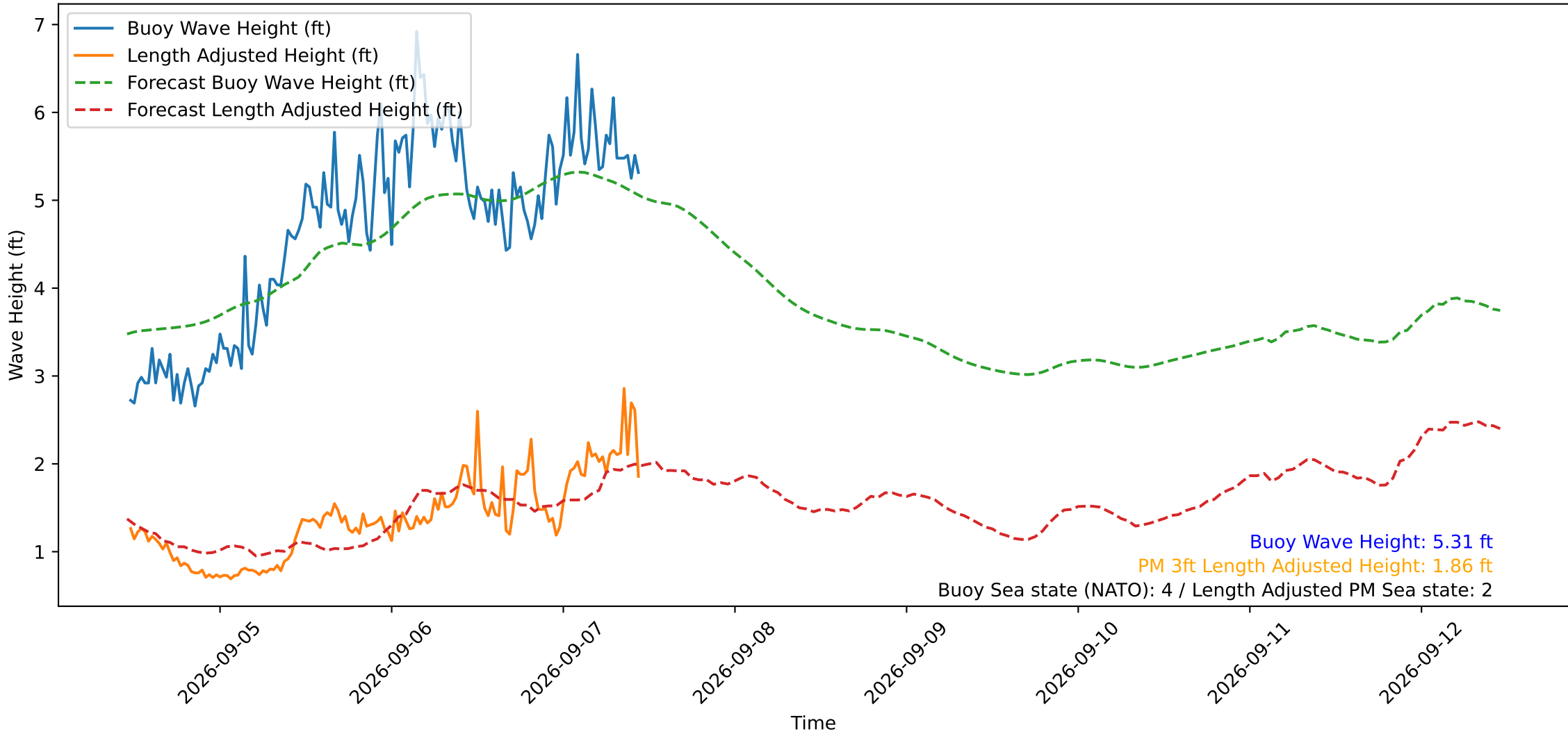
Wave Heights over Time for Red Beach at 2026-09-07 11:20:51
