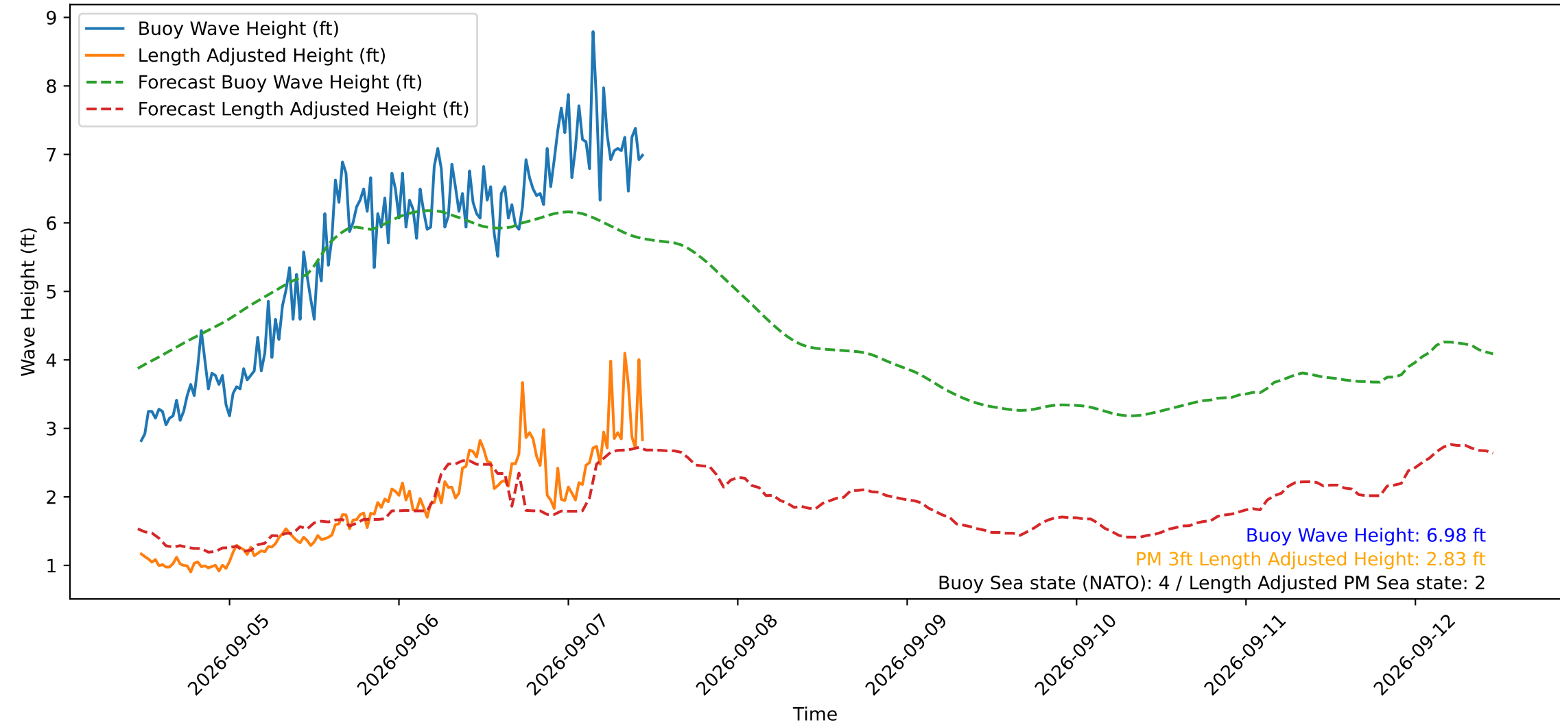
Wave Heights over Time for Green Beach at 2026-09-07 11:21:15
