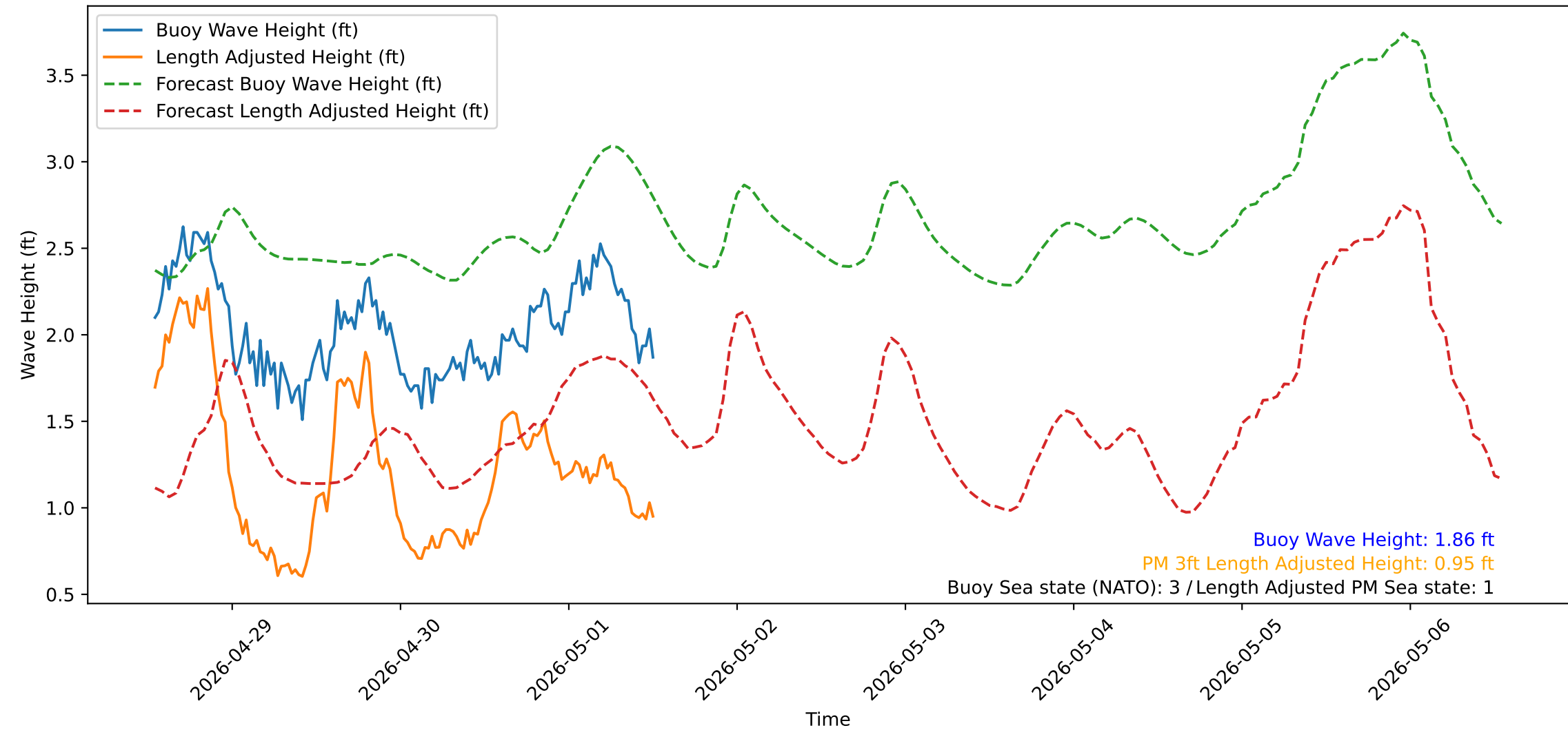
Wave Heights over Time for Red Beach at 2026-05-01 12:50:52
