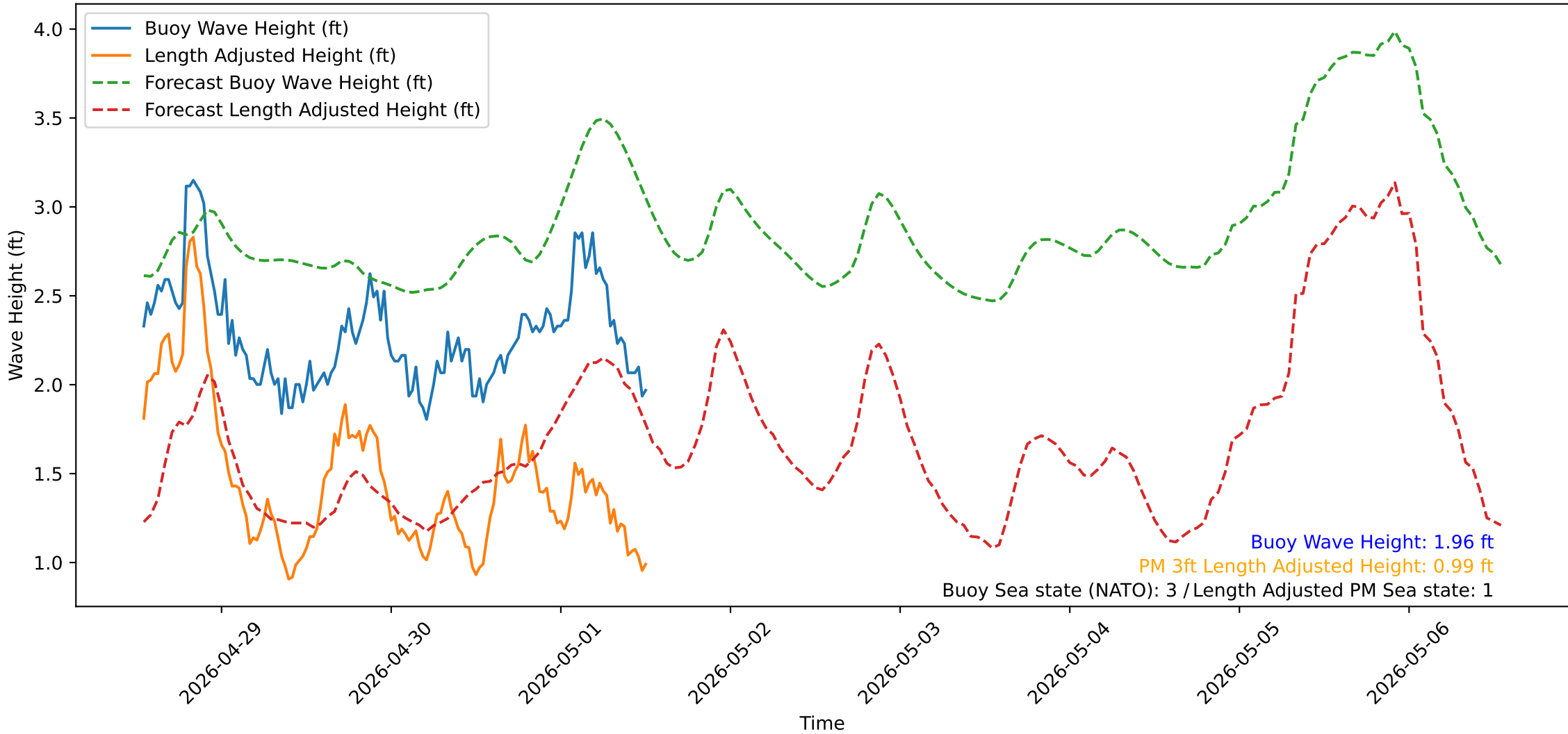
Wave Heights over Time for Green Beach at 2026-05-01 12:51:14
