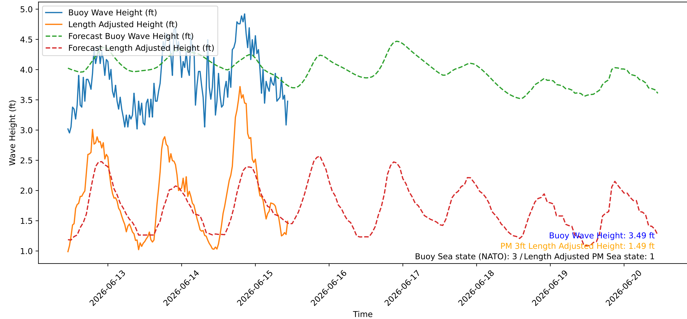
Wave Heights over Time for Green Beach at 2026-06-15 11:11:08
