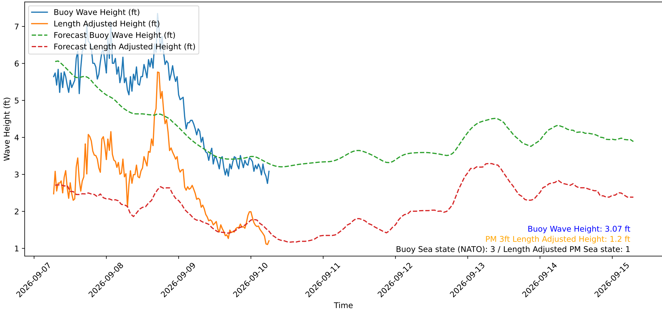
Wave Heights over Time for Oceanside Harbor at 2026-09-10 06:30:30
