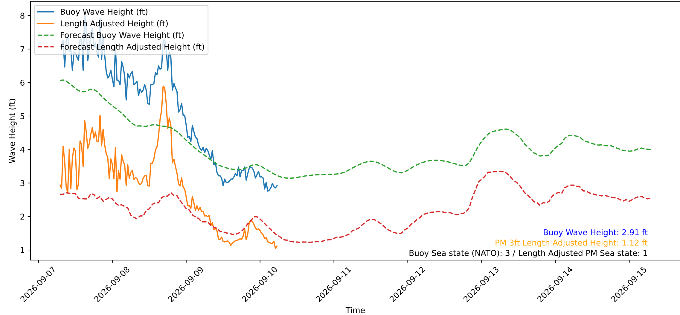
Wave Heights over Time for Green Beach at 2026-09-10 06:31:12
