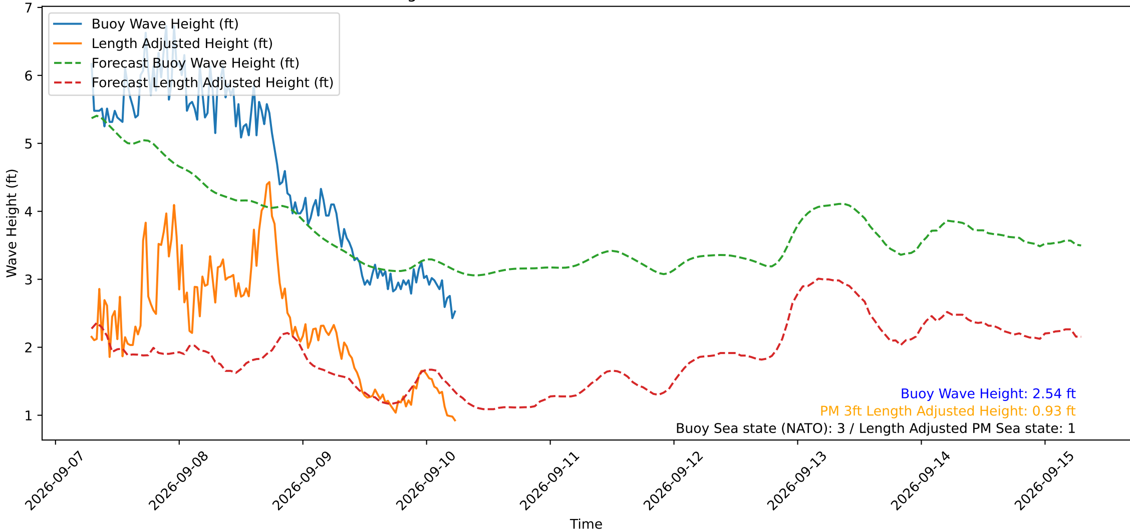
Wave Heights over Time for Red Beach at 2026-09-10 06:30:50
