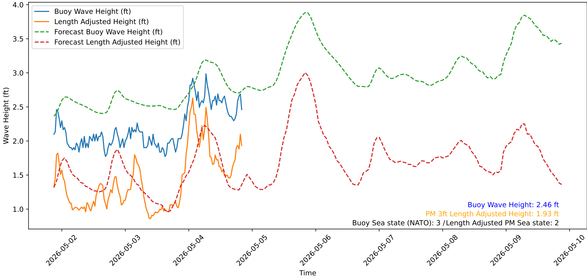
Wave Heights over Time for Green Beach at 2026-05-04 20:51:14
