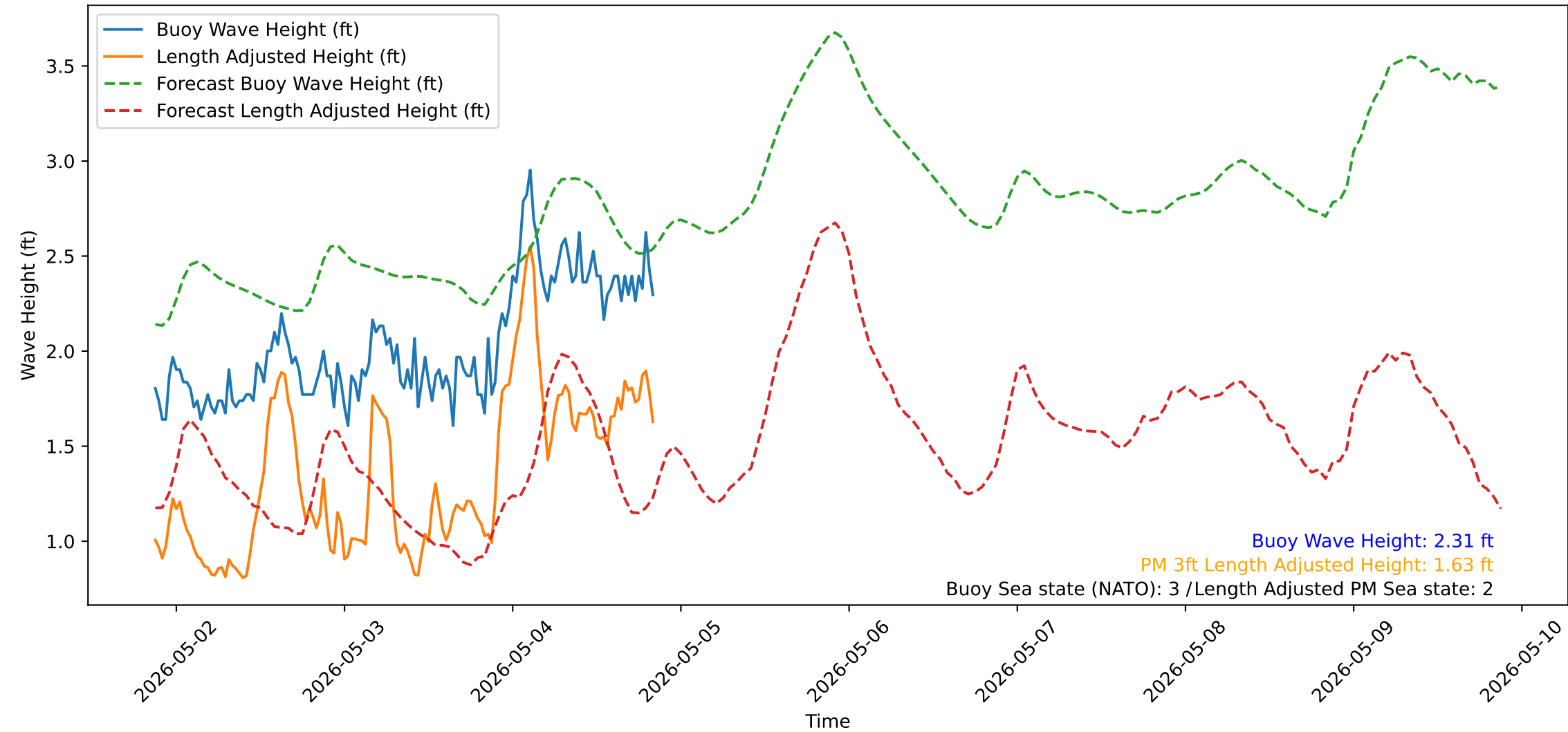
Wave Heights over Time for Red Beach at 2026-05-04 20:50:52
