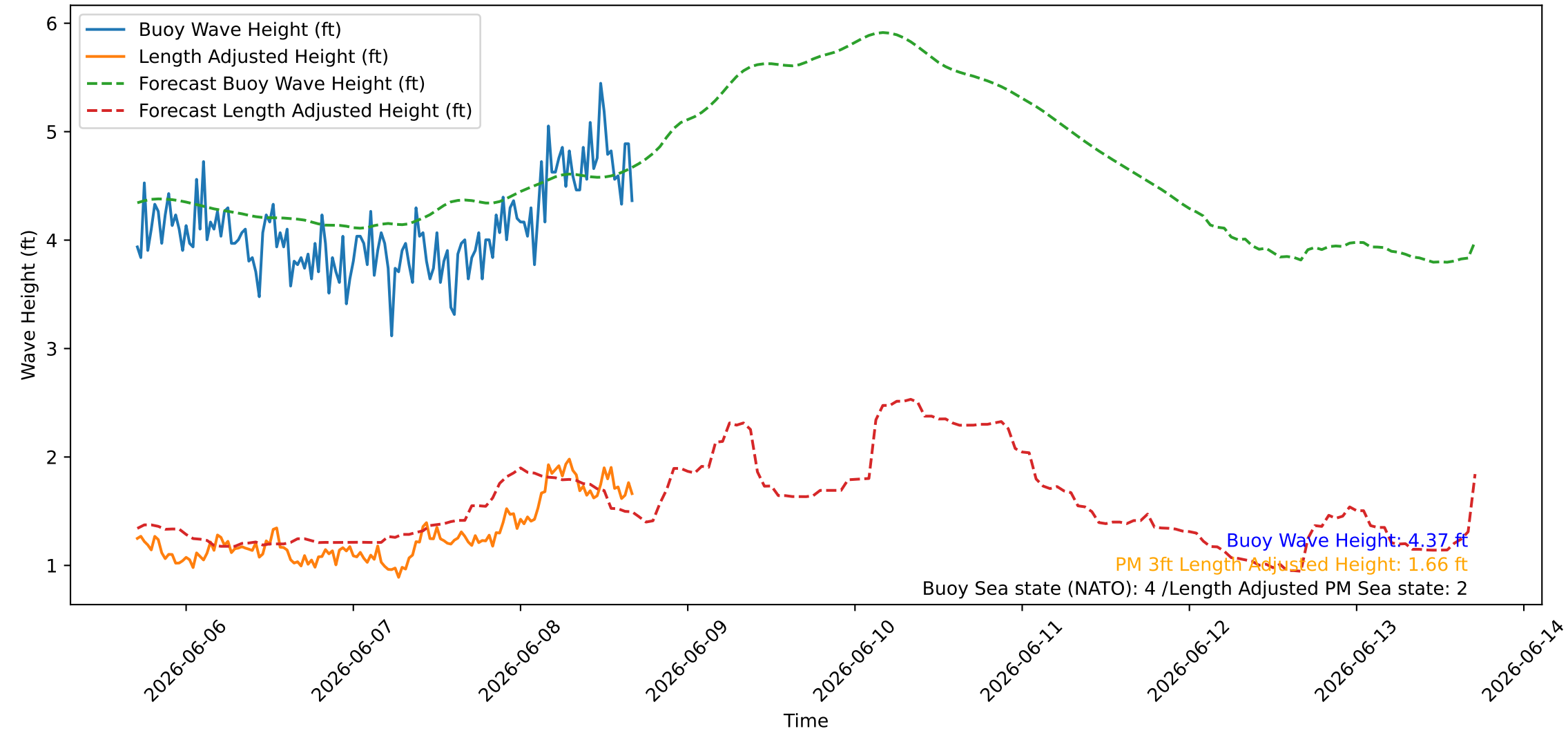
Wave Heights over Time for Green Beach at 2026-06-08 17:01:08
