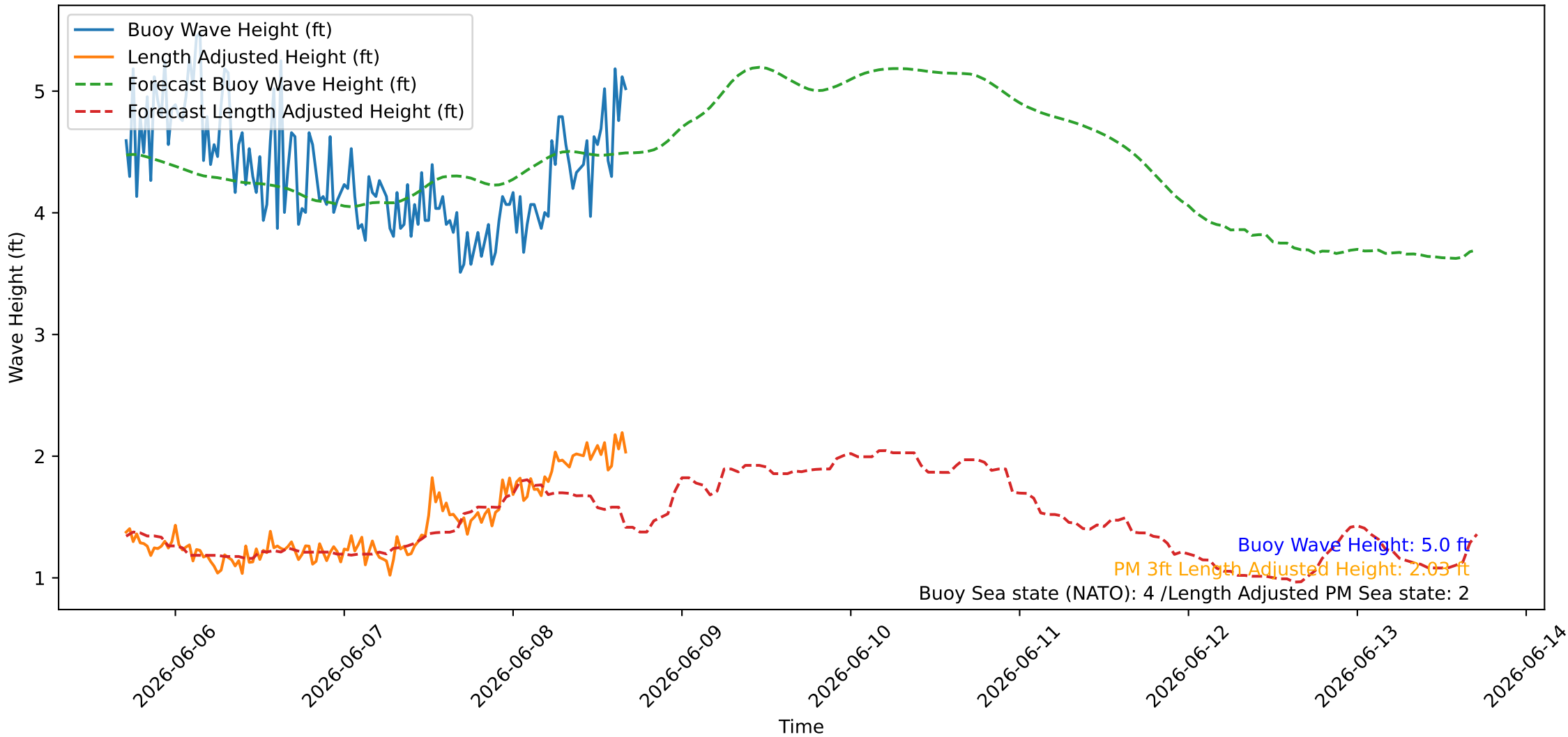
Wave Heights over Time for Oceanside Harbor at 2026-06-08 17:00:26
