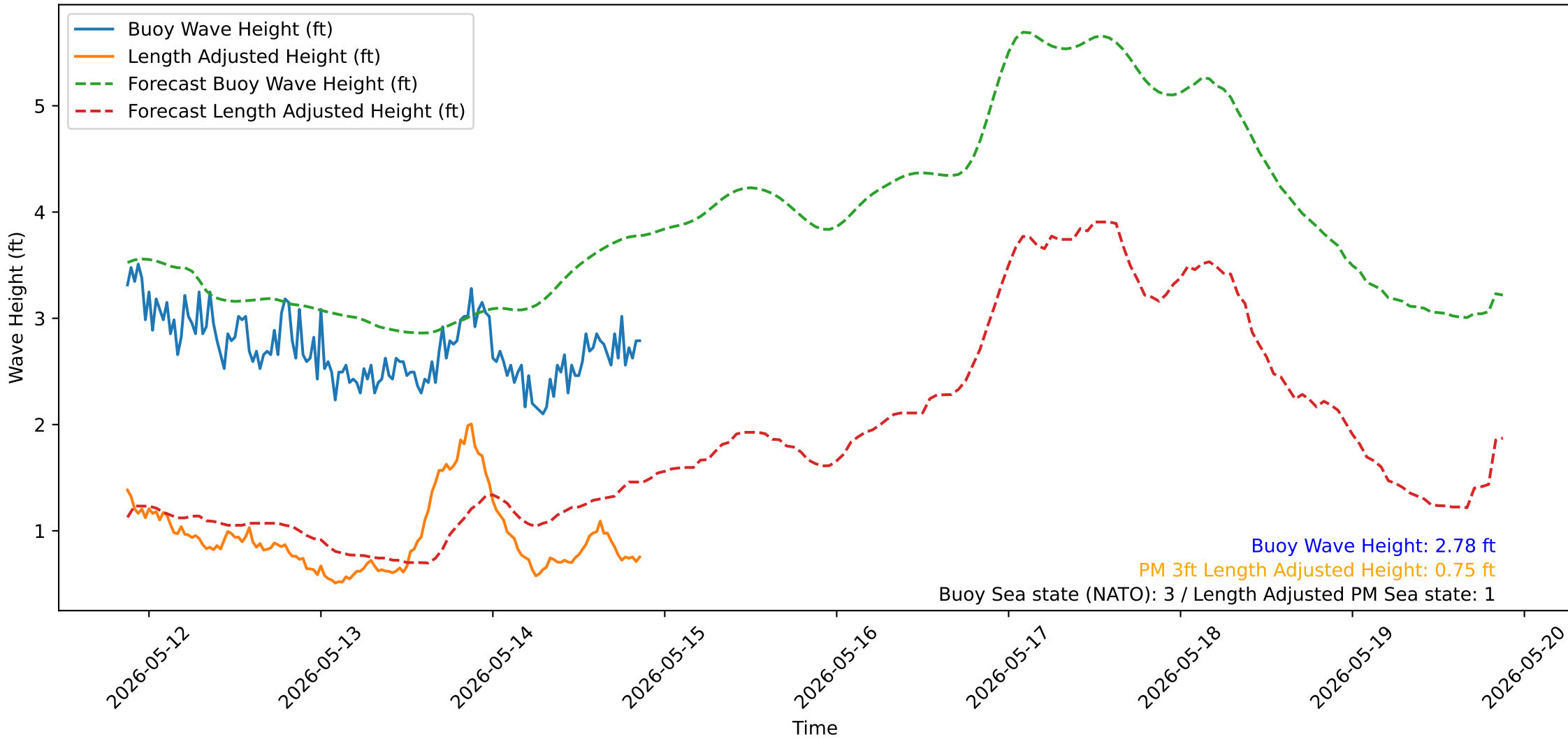
Wave Heights over Time for Green Beach at 2026-05-14 21:11:14
