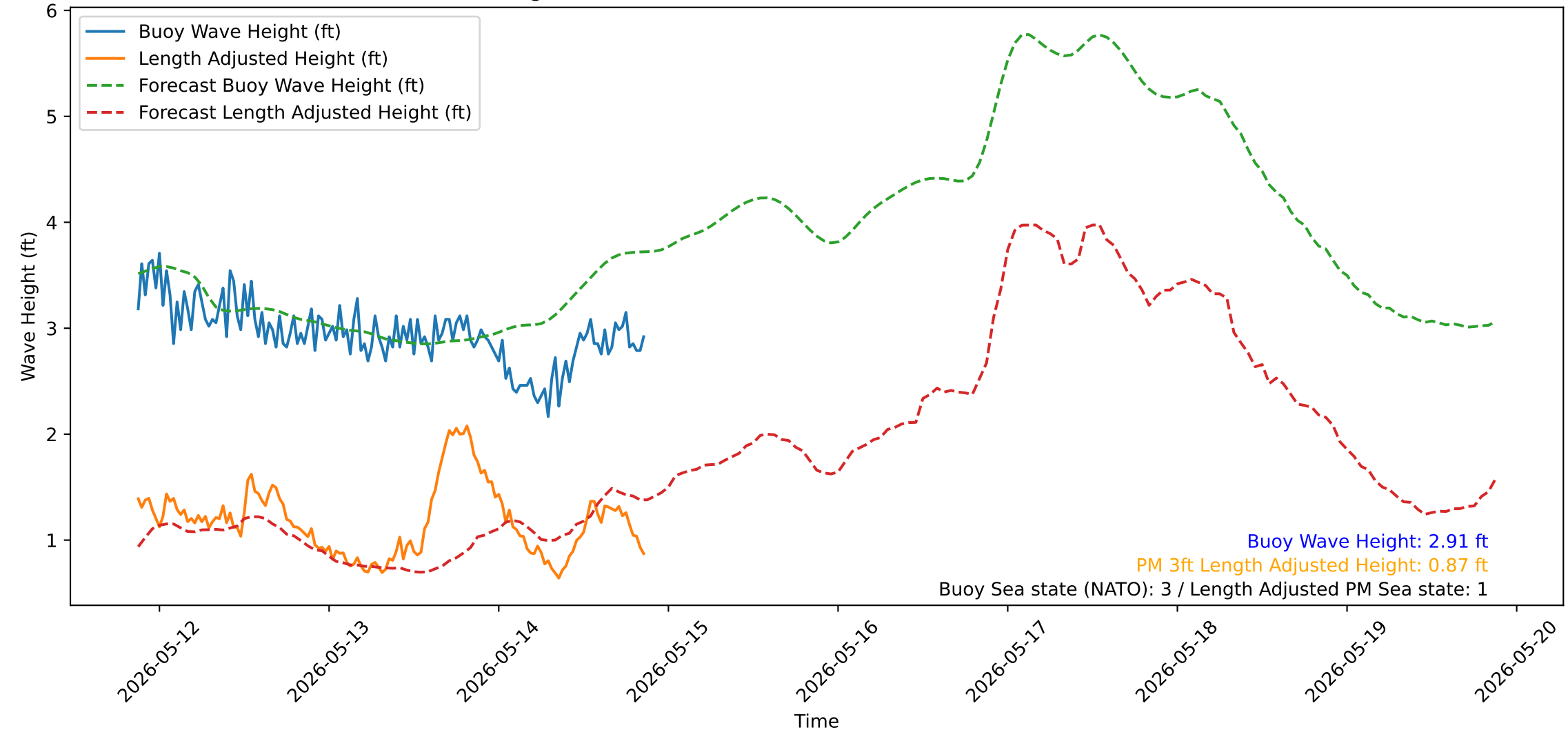
Wave Heights over Time for Oceanside Harbor at 2026-05-14 21:10:31
