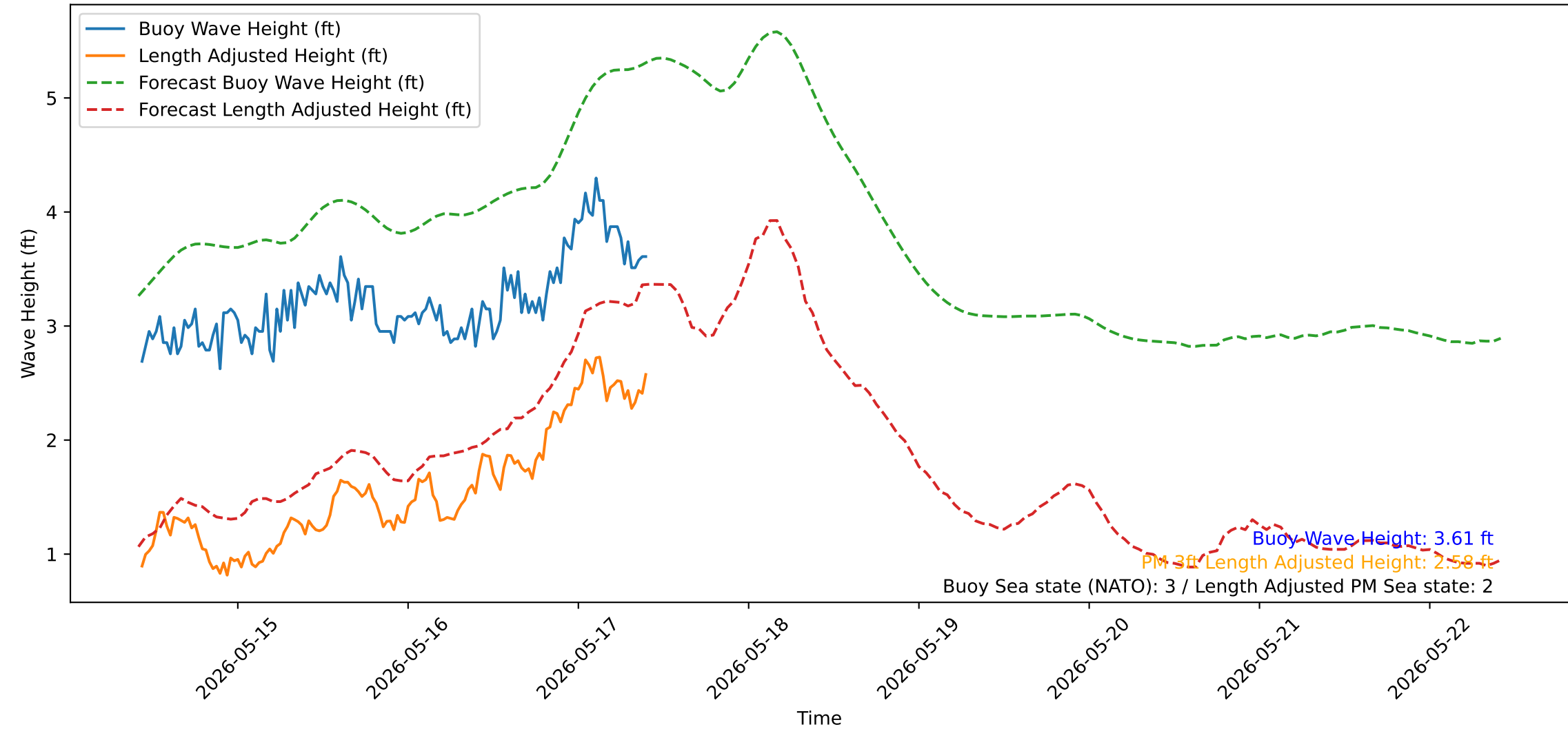
Wave Heights over Time for Oceanside Harbor at 2026-05-17 10:20:31
