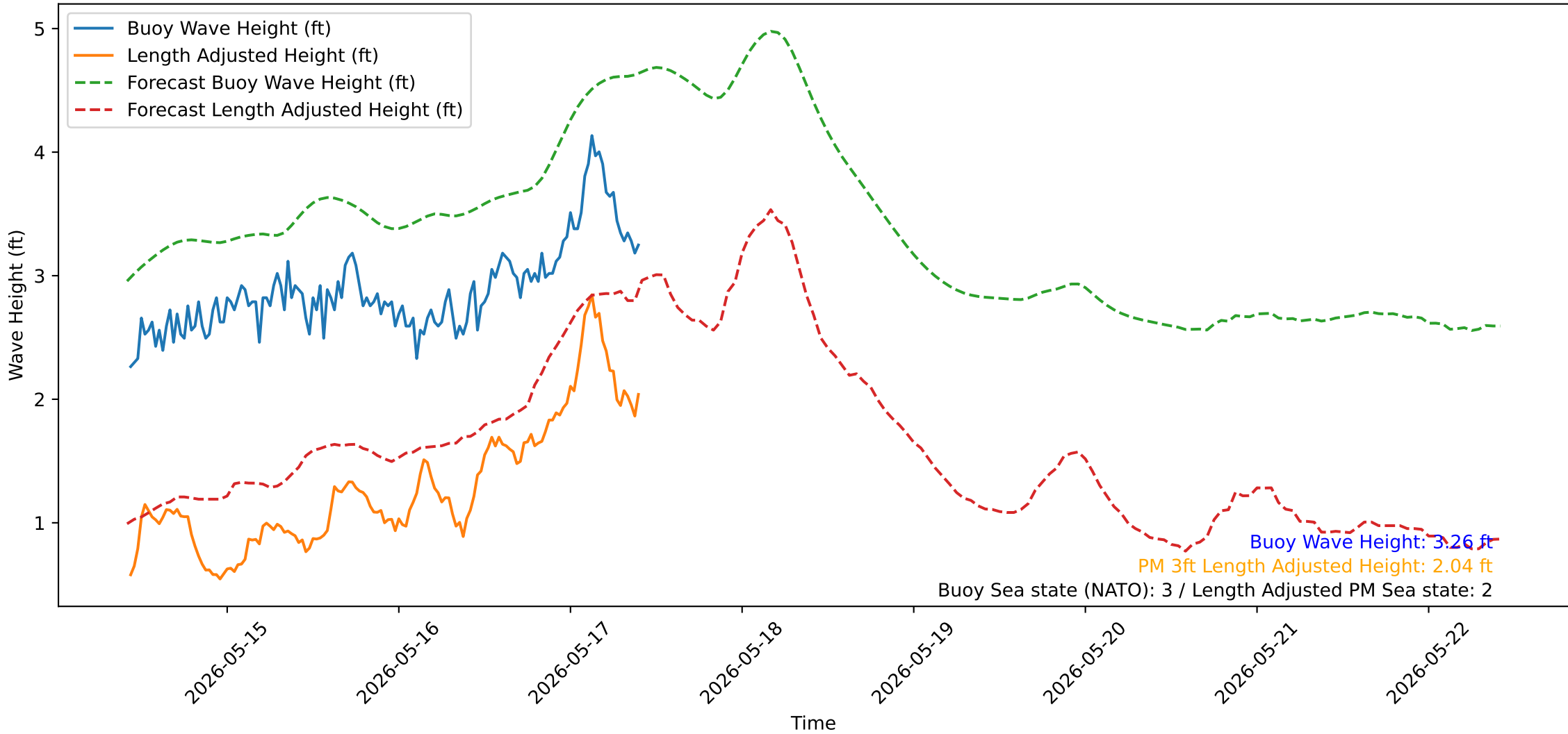
Wave Heights over Time for Red Beach at 2026-05-17 10:20:52
