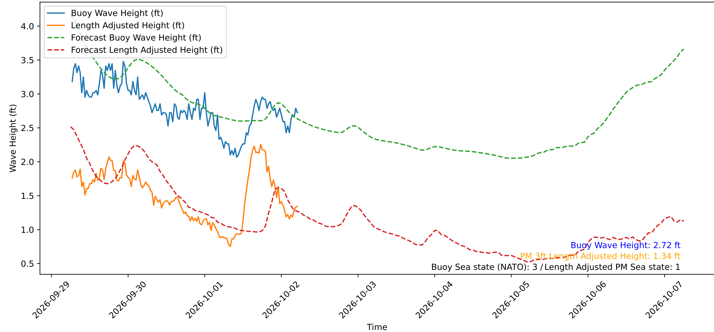
Wave Heights over Time for Red Beach at 2026-10-02 06:00:49
