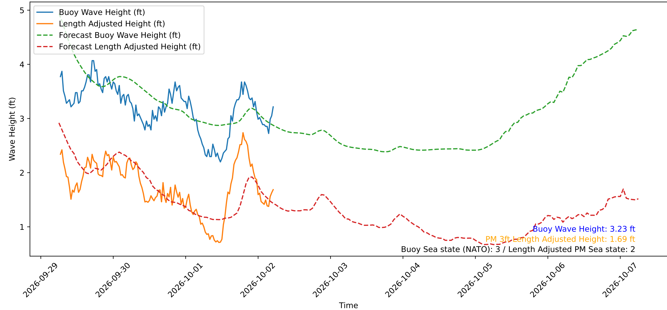
Wave Heights over Time for Green Beach at 2026-10-02 06:01:11
