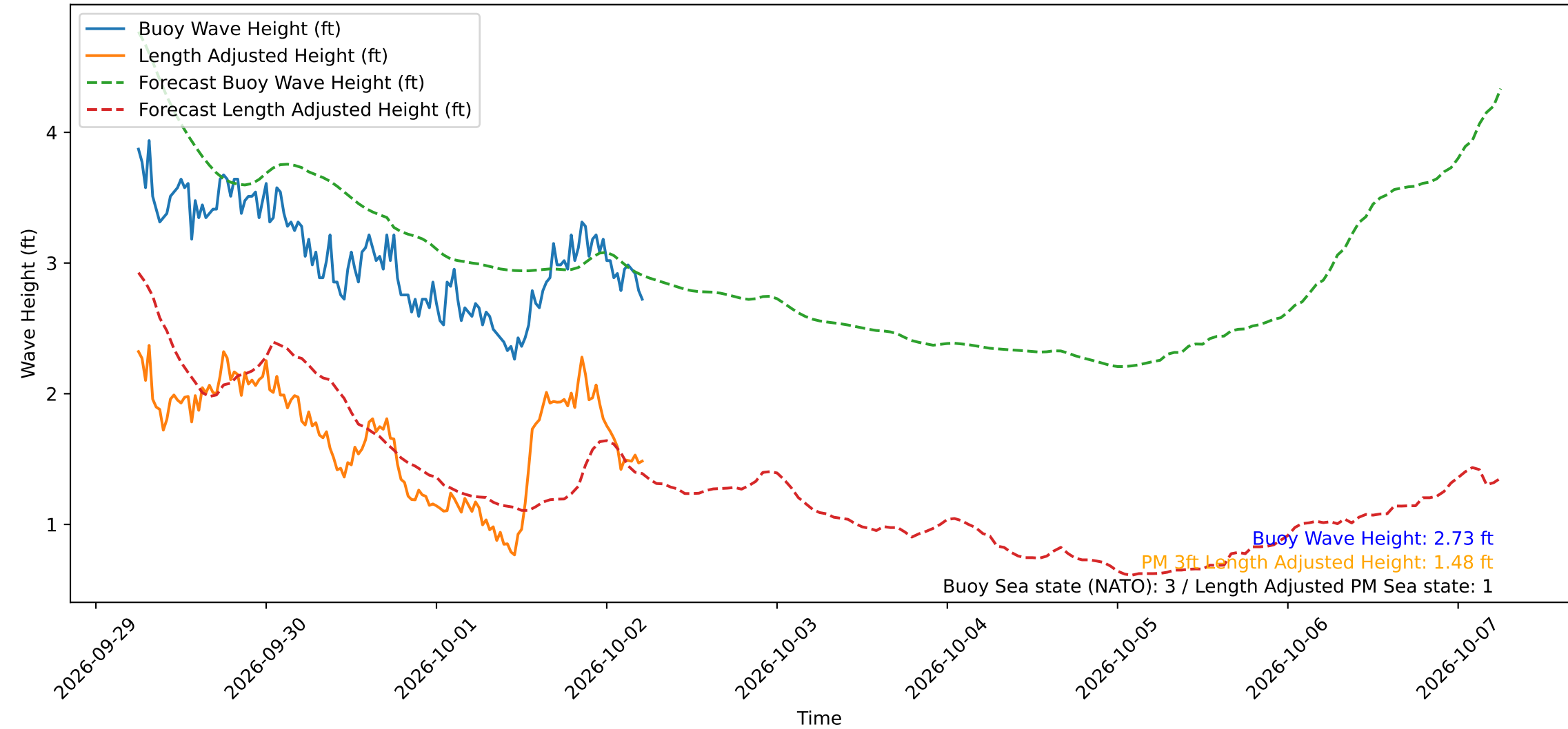
Wave Heights over Time for Oceanside Harbor at 2026-10-02 06:00:29
