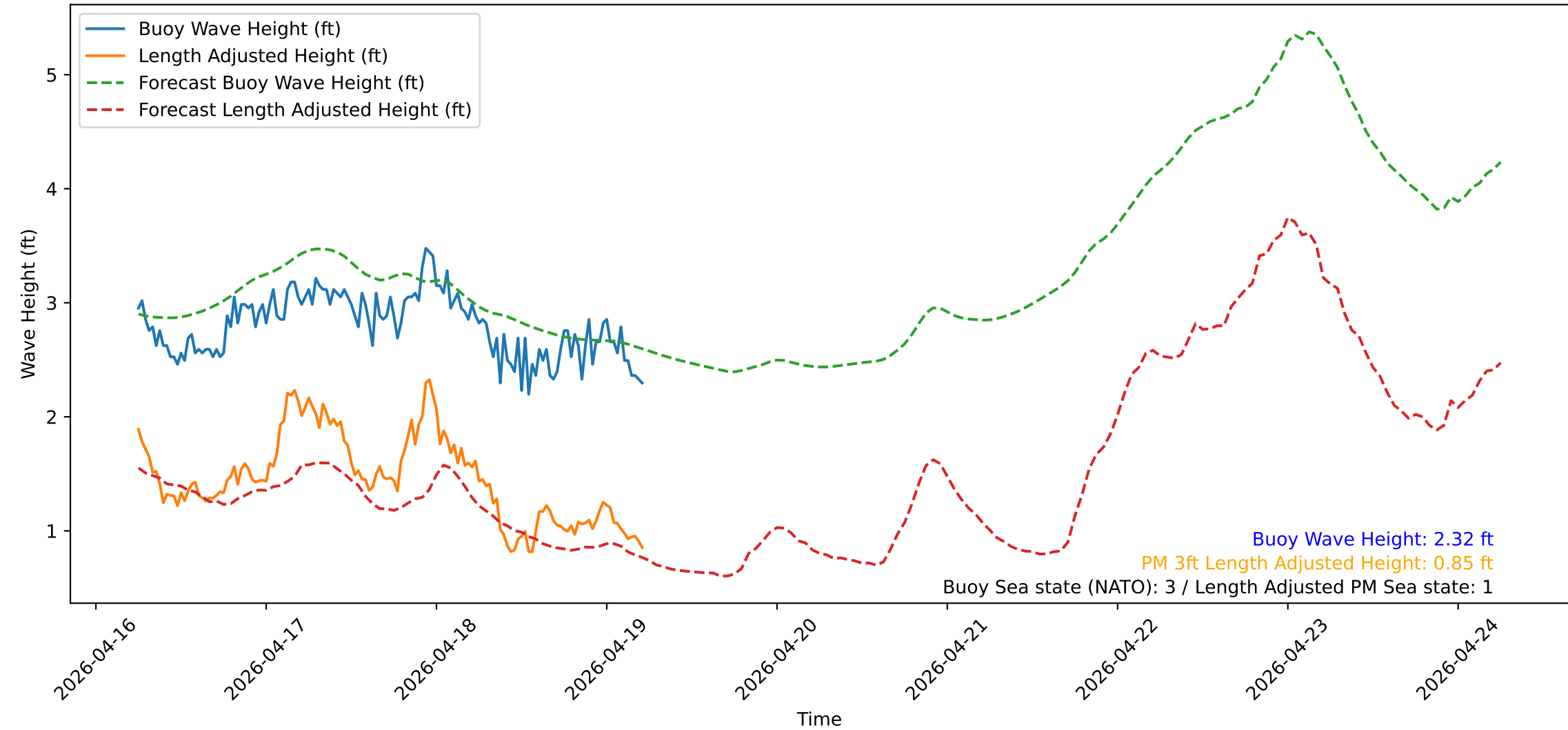
Wave Heights over Time for Green Beach at 2026-04-19 05:51:15
