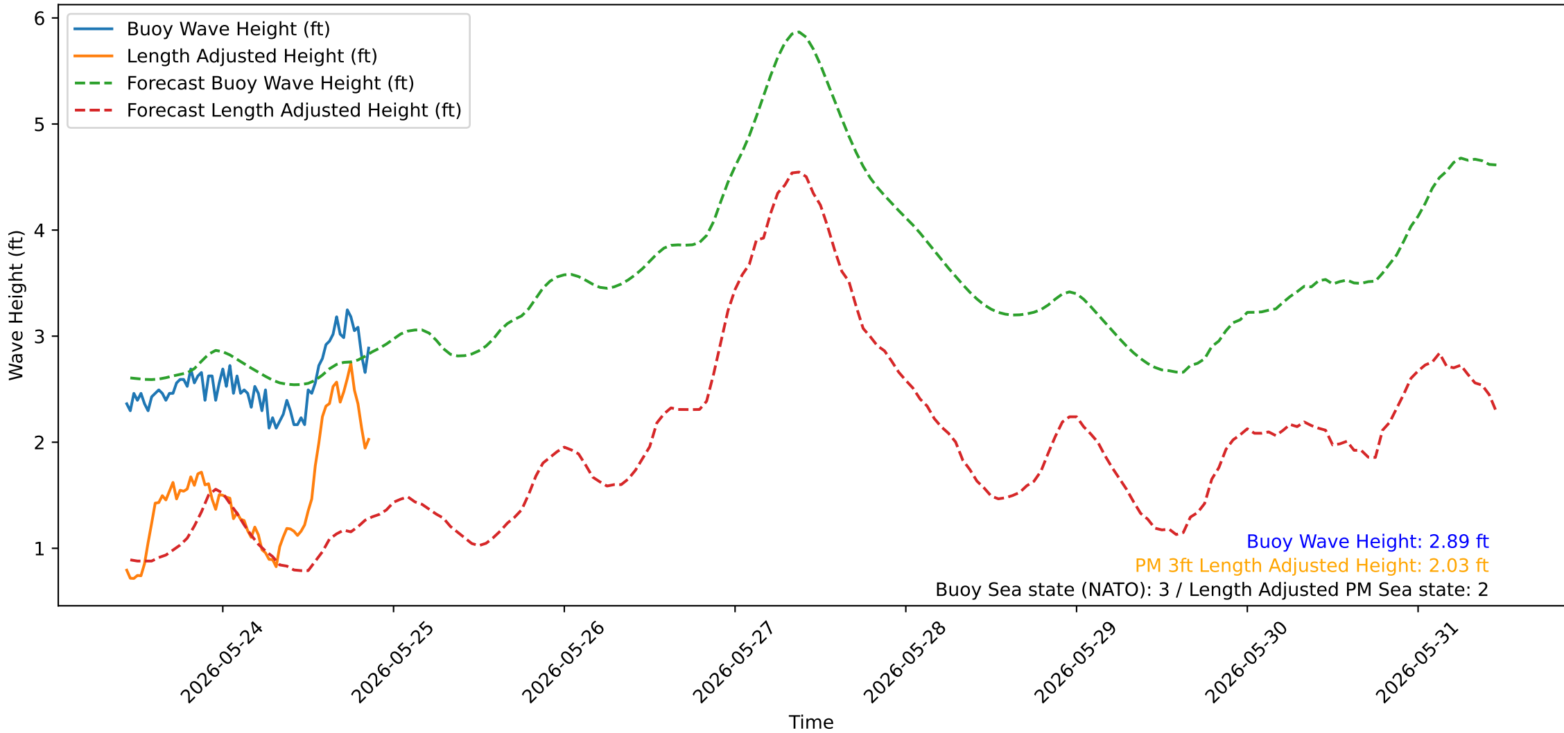
Wave Heights over Time for Oceanside Harbor at 2026-05-26 10:30:29
