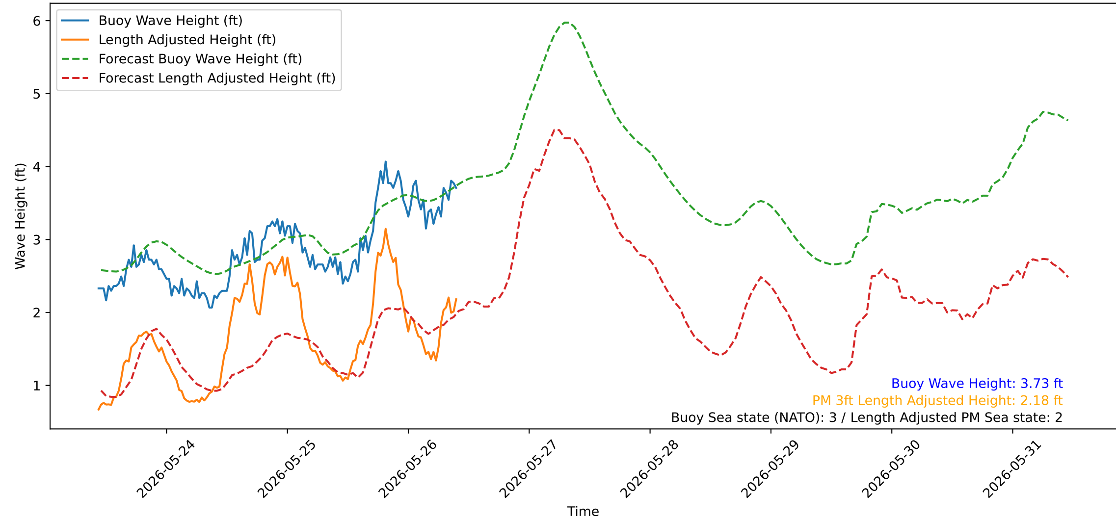
Wave Heights over Time for Green Beach at 2026-05-26 10:31:10
