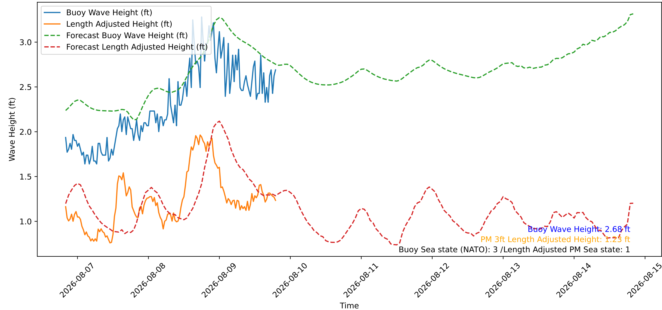
Wave Heights over Time for Oceanside Harbor at 2026-08-09 20:00:26
