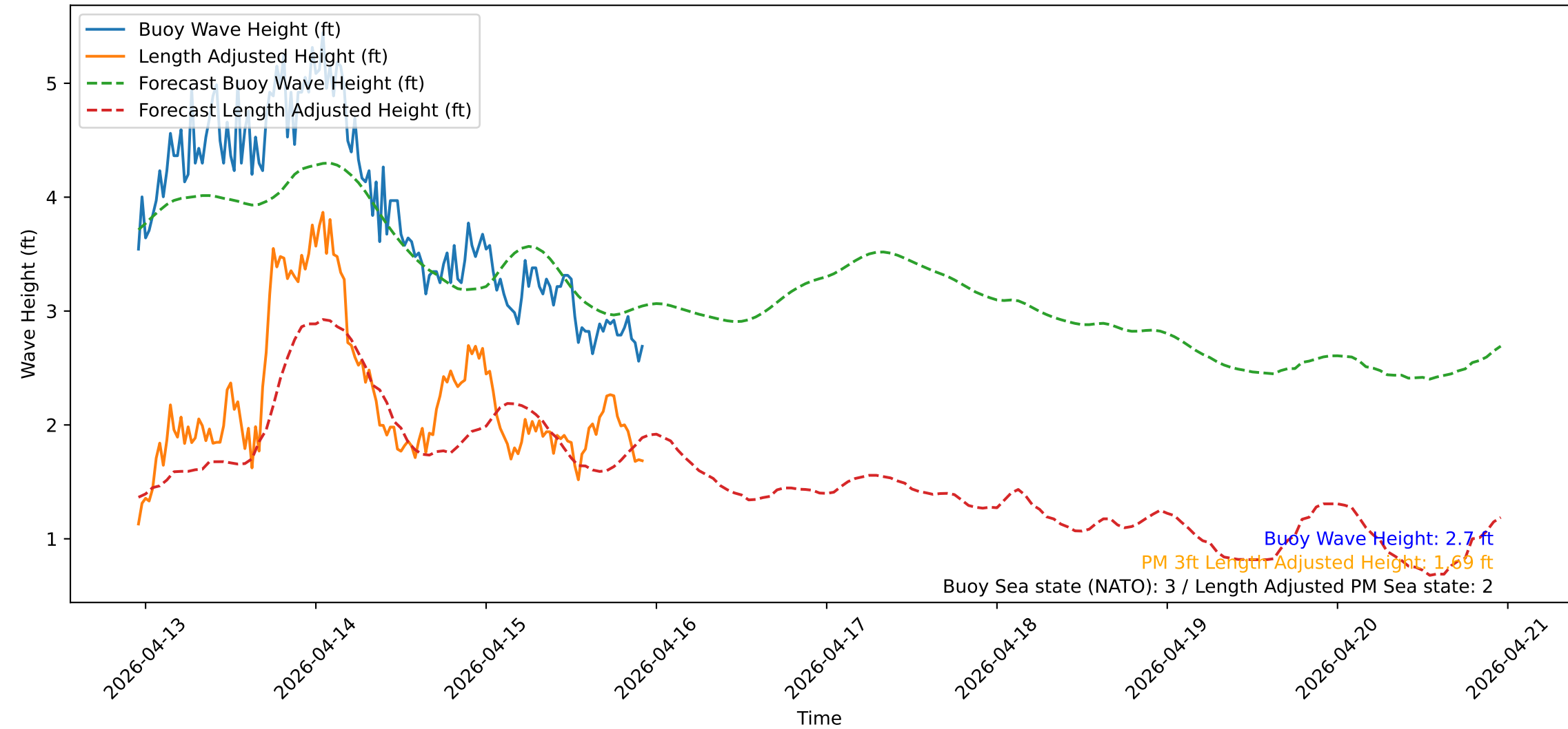
Wave Heights over Time for Oceanside Harbor at 2026-04-15 23:10:32
