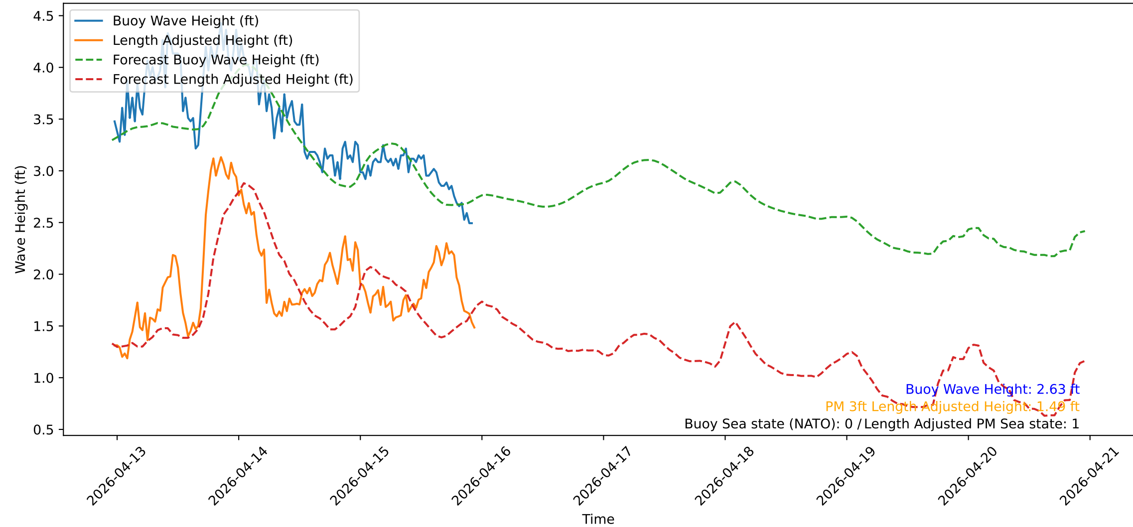
Wave Heights over Time for Red Beach at 2026-04-15 23:10:51
