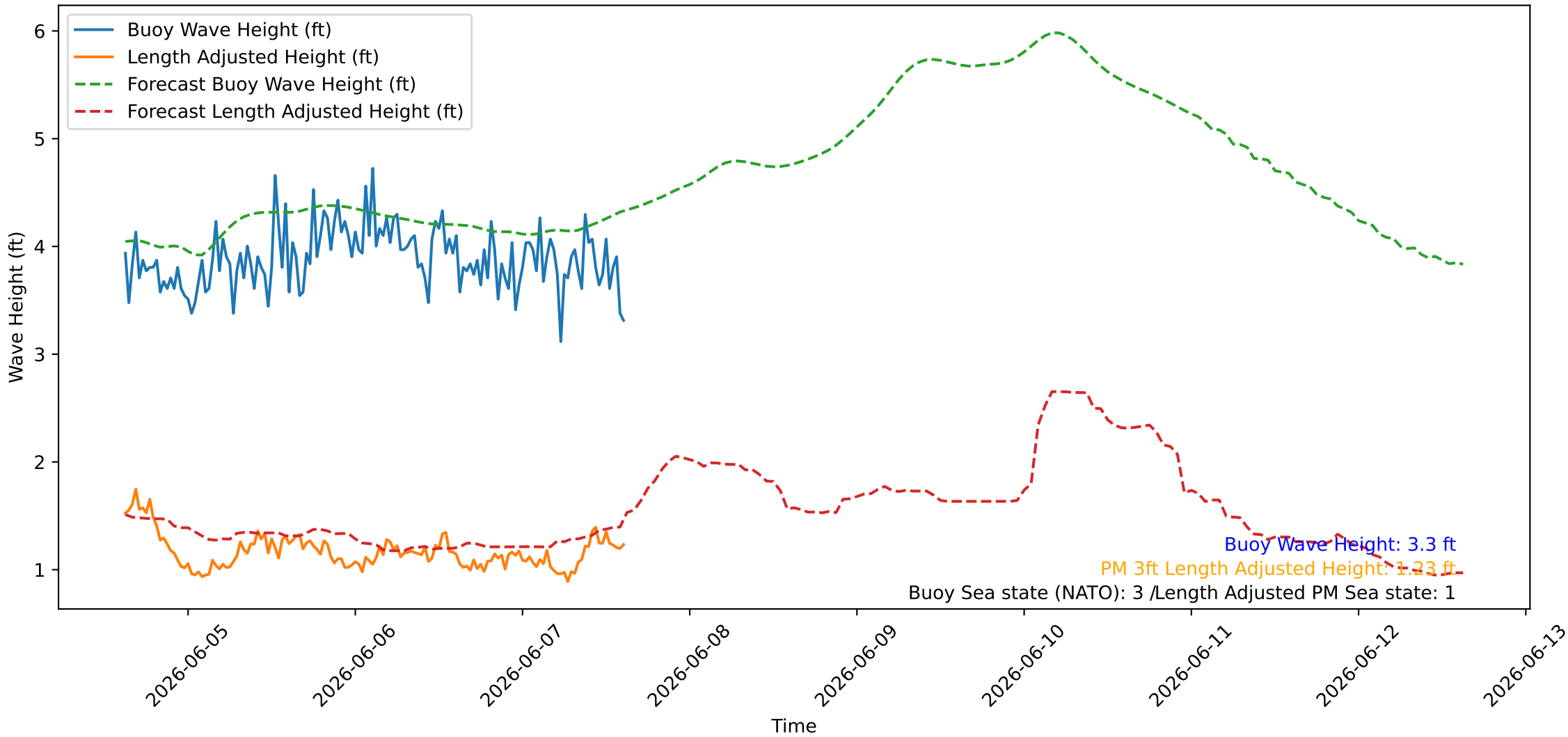
Wave Heights over Time for Green Beach at 2026-06-07 15:11:08
