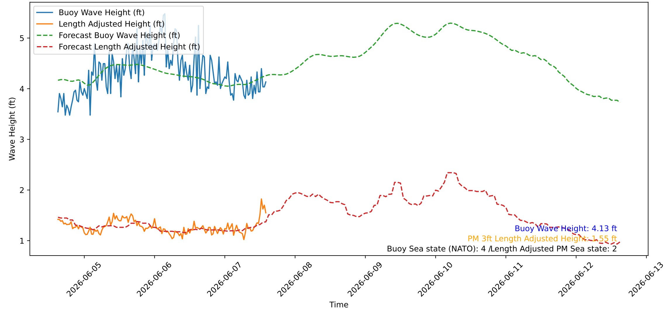
Wave Heights over Time for Oceanside Harbor at 2026-06-07 15:10:26
