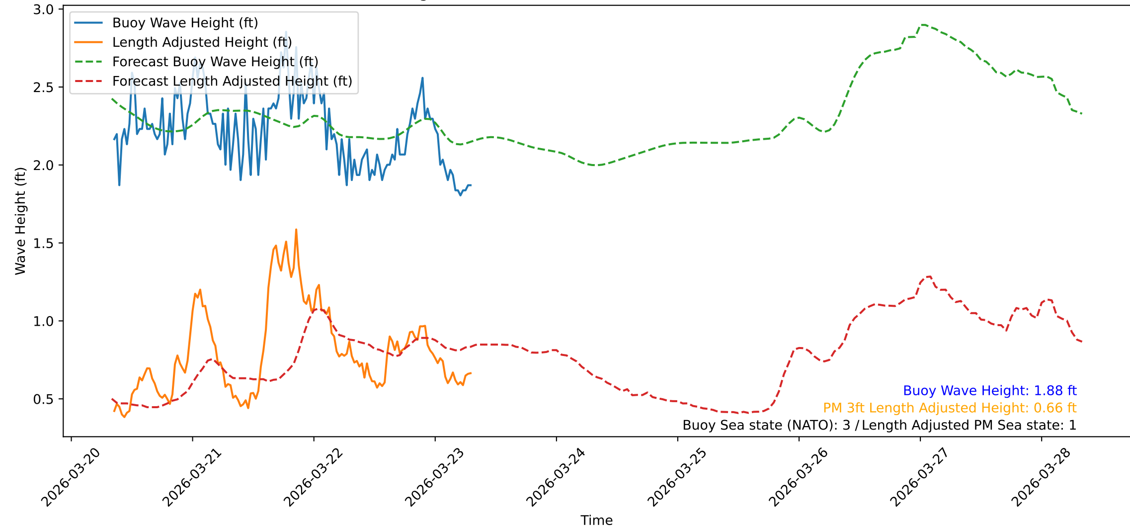
Wave Heights over Time for Red Beach at 2026-03-23 08:00:47
