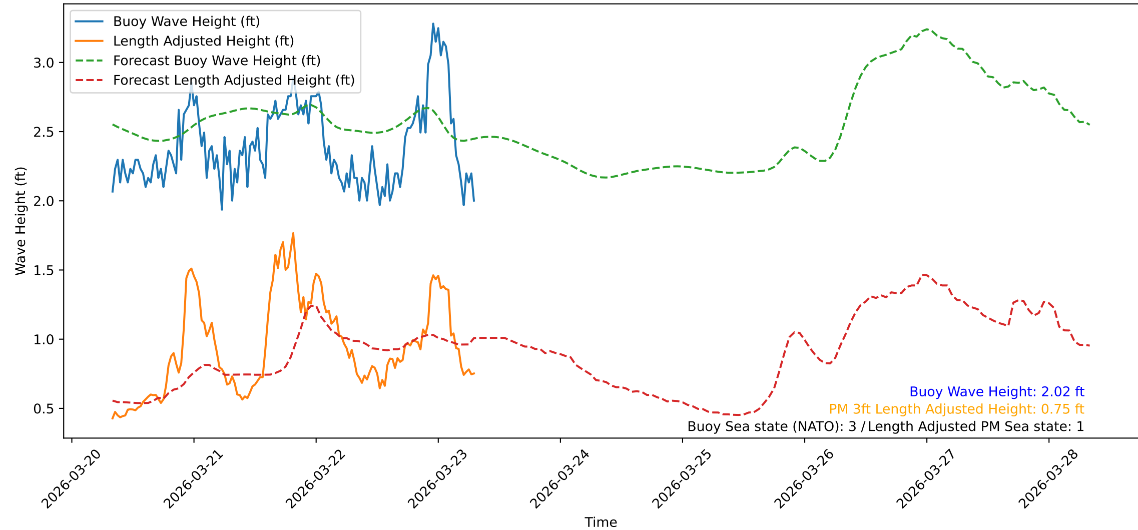
Wave Heights over Time for Green Beach at 2026-03-23 08:01:10
