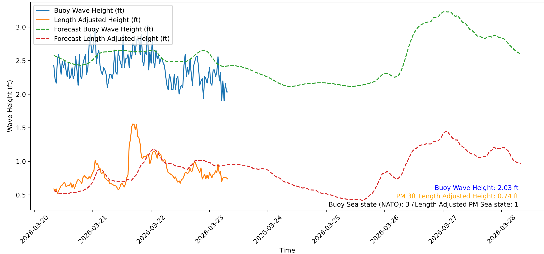
Wave Heights over Time for Oceanside Harbor at 2026-03-23 08:00:32
