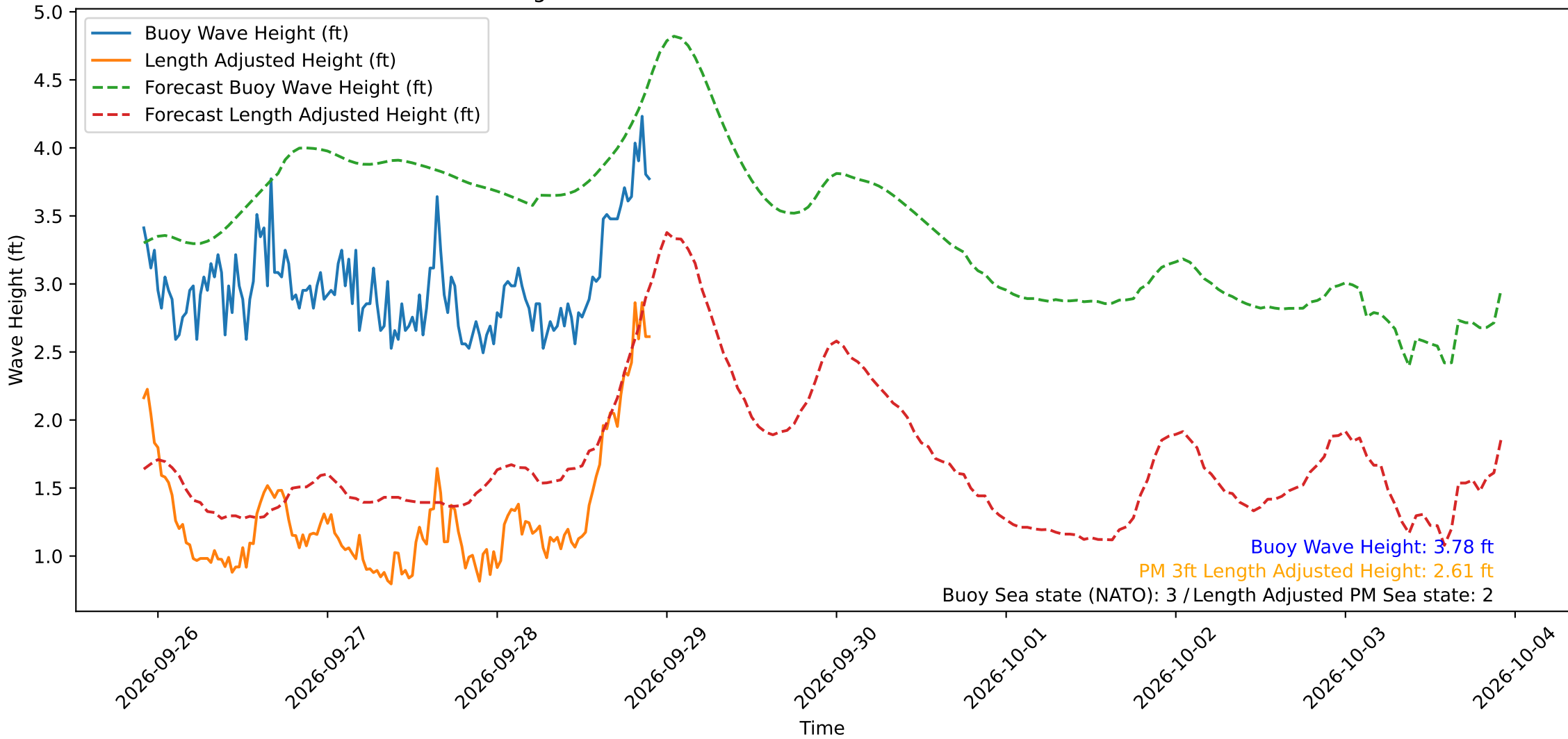
Wave Heights over Time for Oceanside Harbor at 2026-09-28 22:00:29
