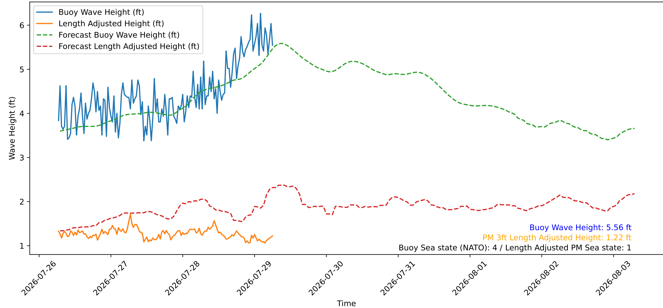
Wave Heights over Time for Green Beach at 2026-07-29 06:41:09
