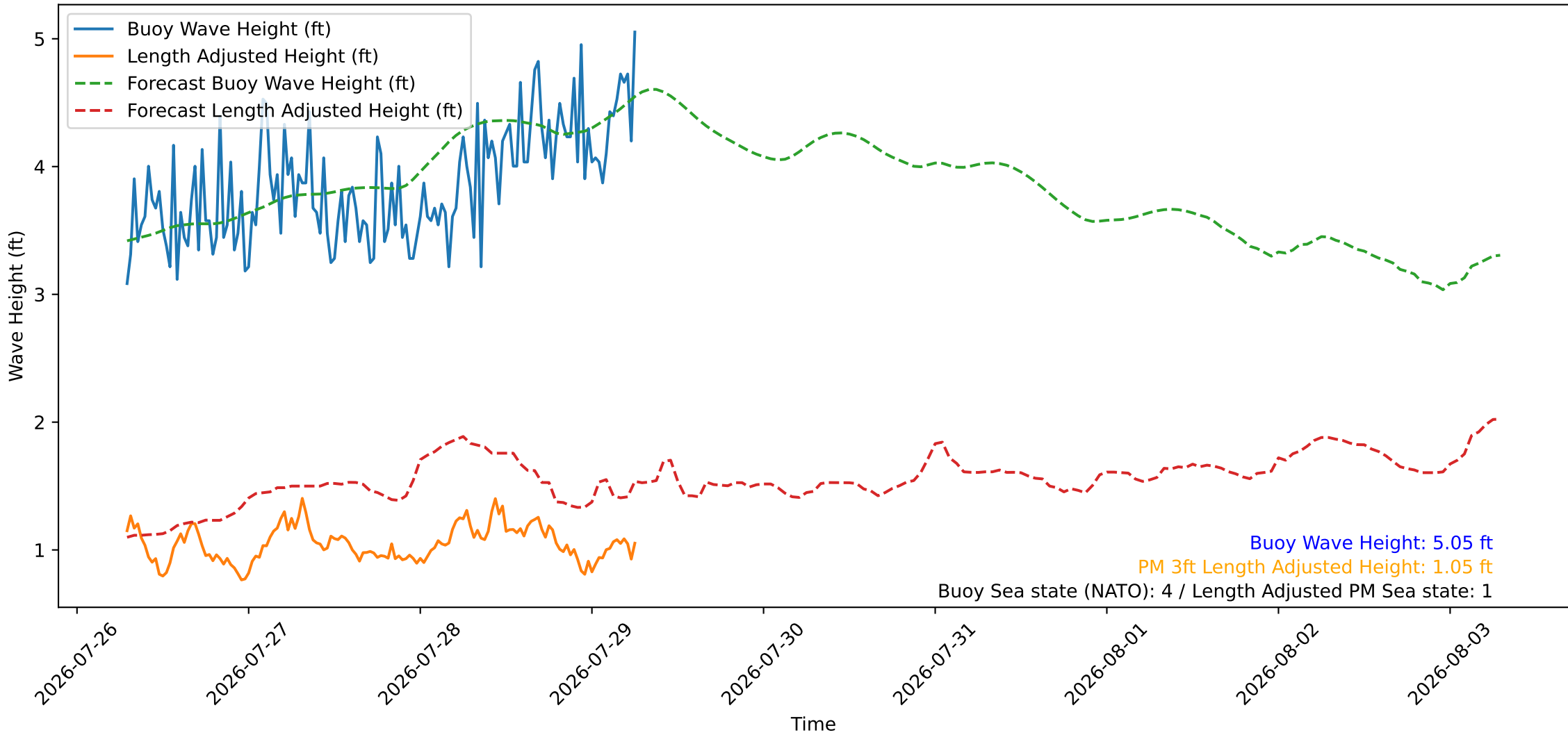
Wave Heights over Time for Red Beach at 2026-07-29 06:40:46
