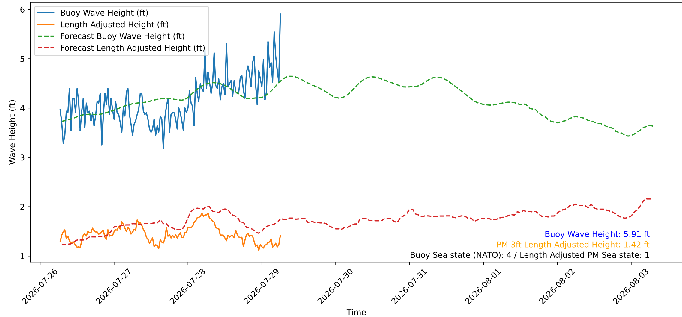
Wave Heights over Time for Oceanside Harbor at 2026-07-29 06:40:26
