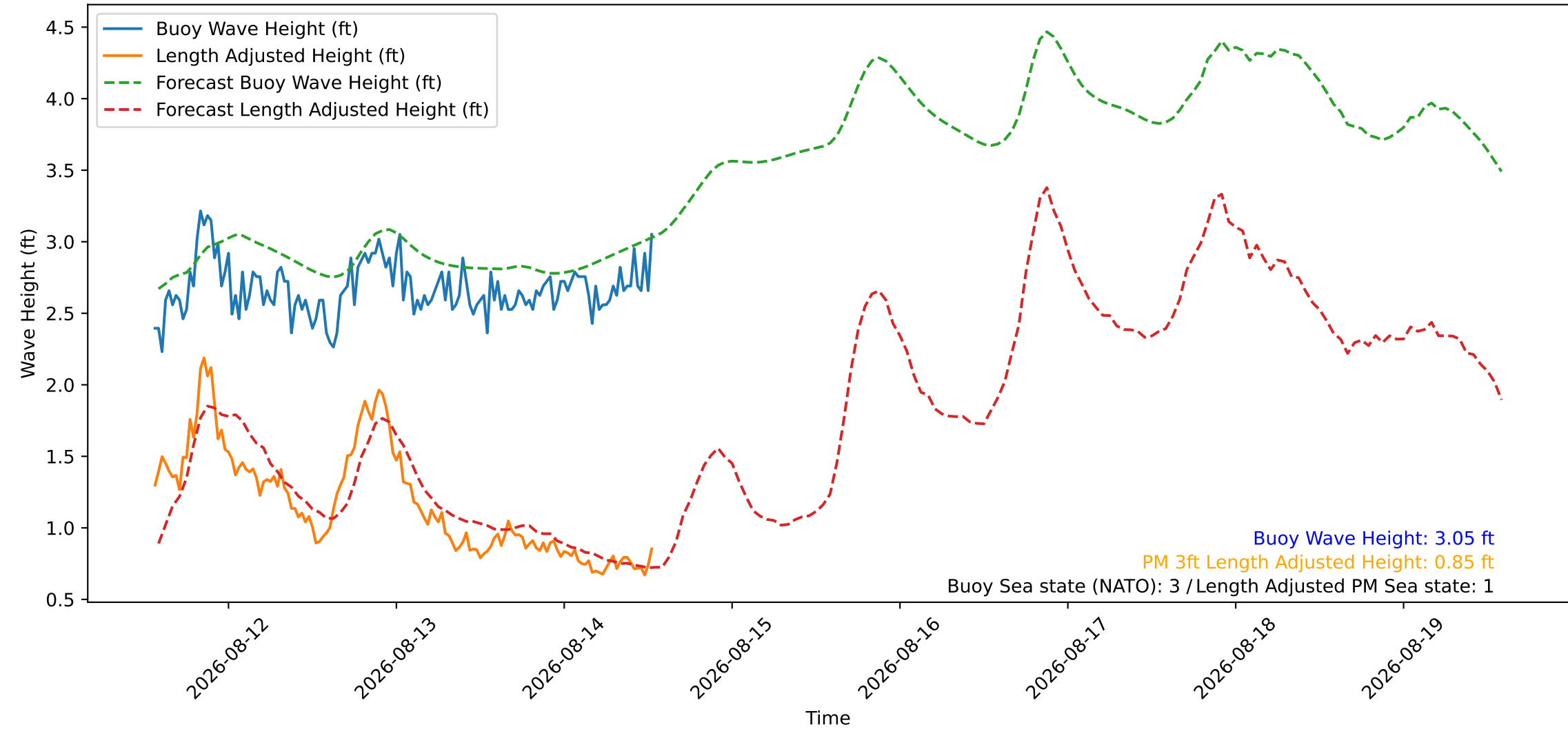
Wave Heights over Time for Green Beach at 2026-08-14 13:31:08
