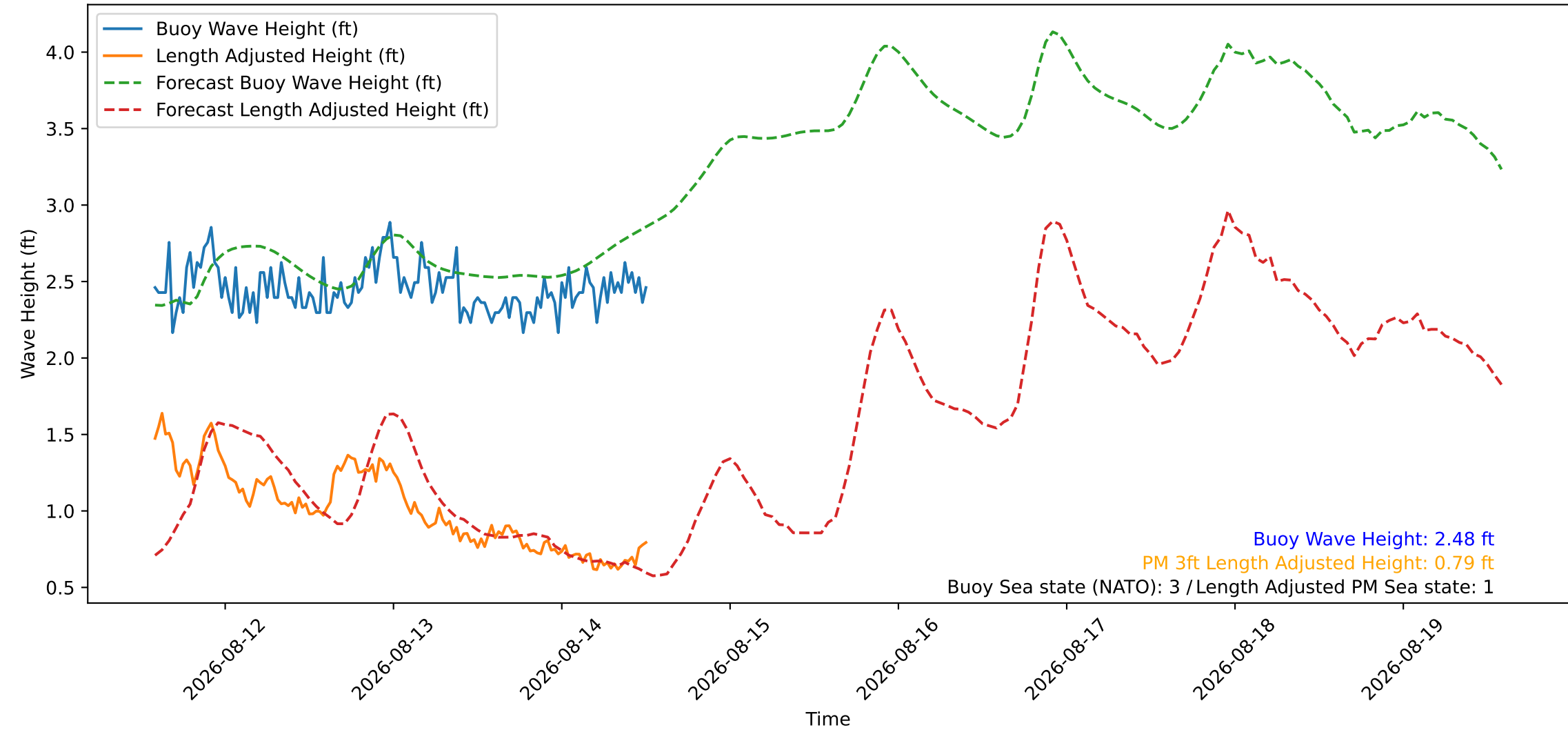
Wave Heights over Time for Red Beach at 2026-08-14 13:30:46
