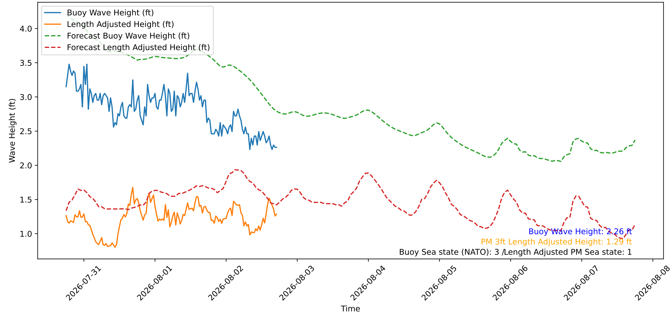
Wave Heights over Time for Red Beach at 2026-08-02 17:50:47
