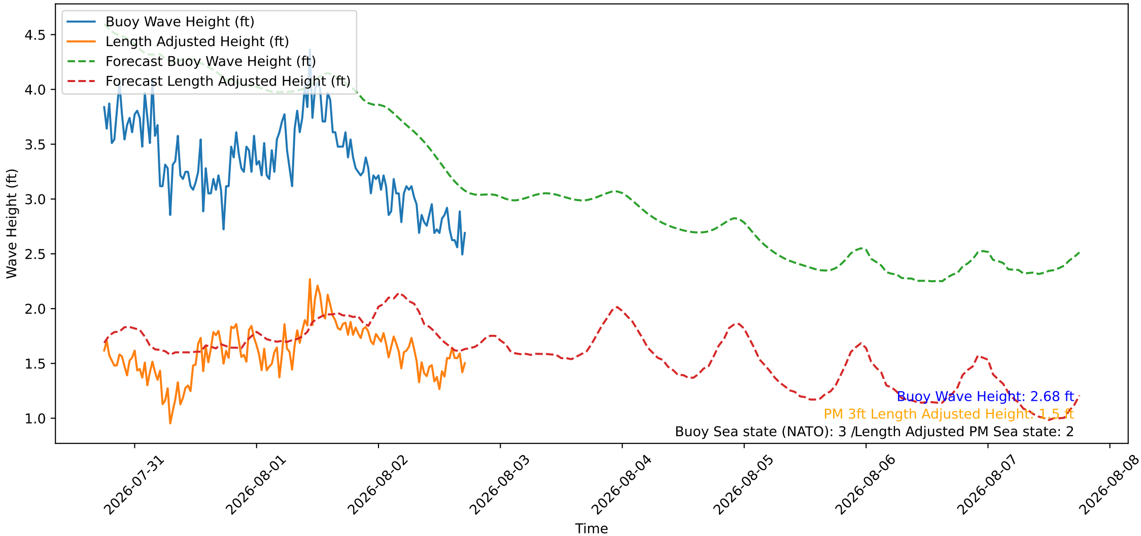
Wave Heights over Time for Oceanside Harbor at 2026-08-02 17:50:26
