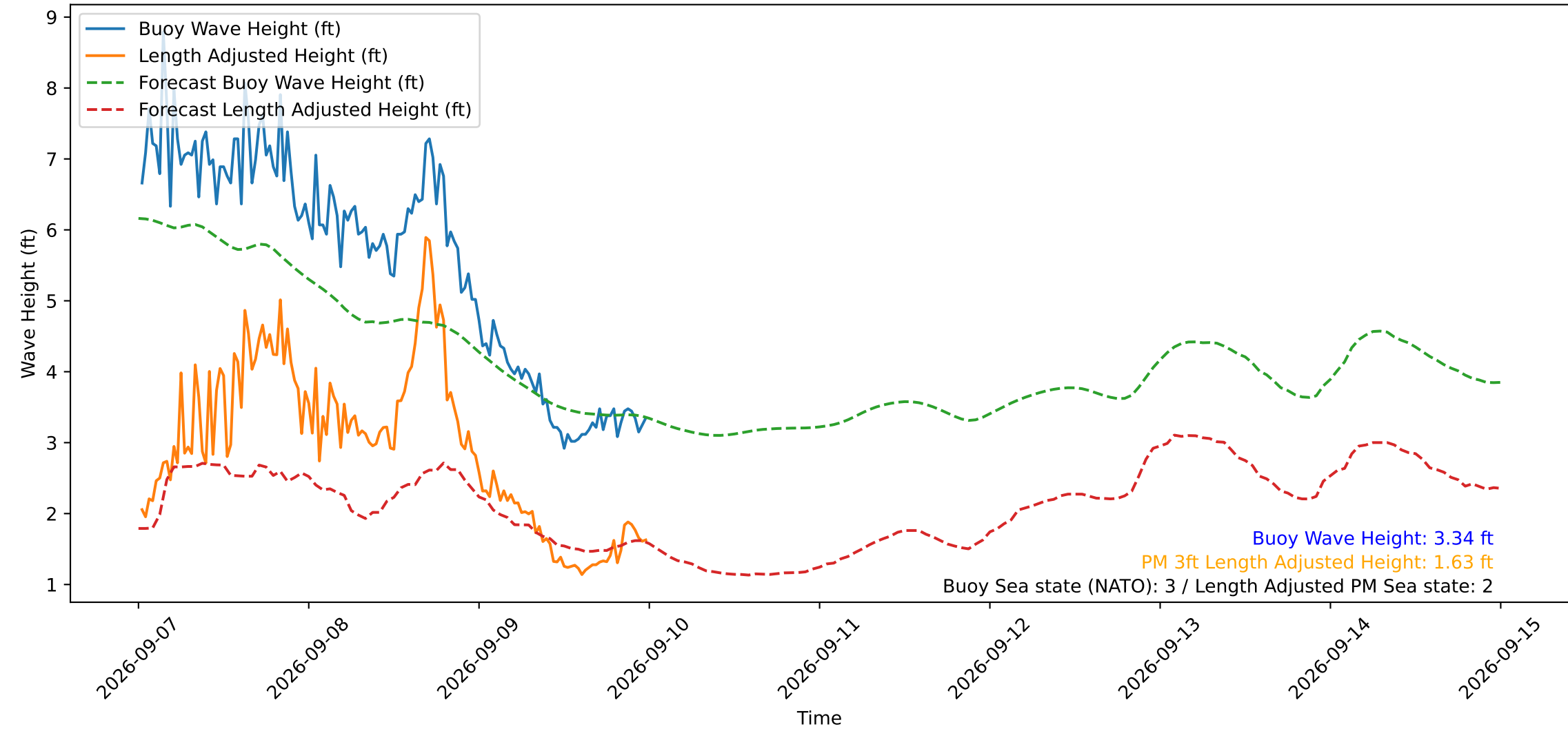
Wave Heights over Time for Green Beach at 2026-09-10 00:21:14
