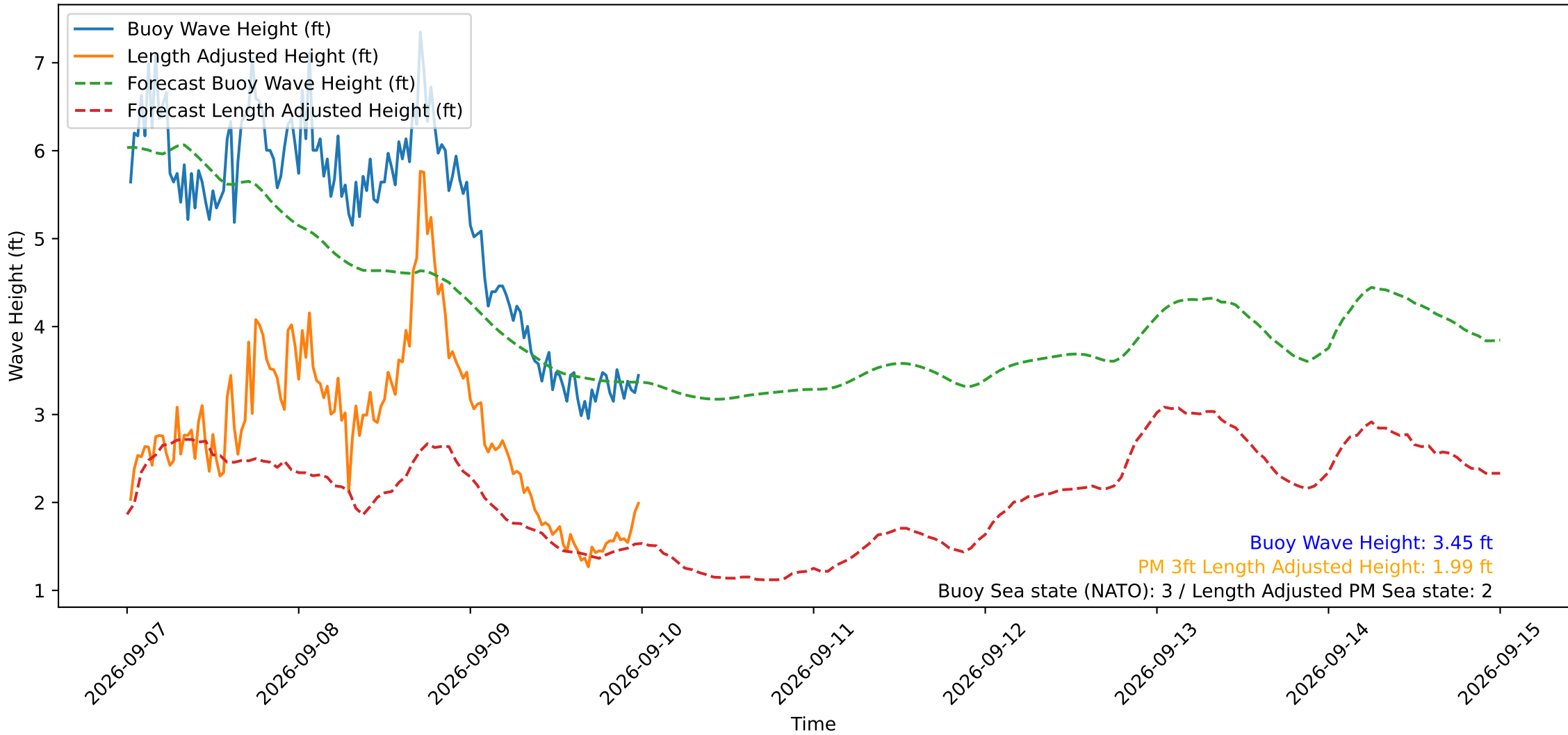
Wave Heights over Time for Oceanside Harbor at 2026-09-10 00:20:29
