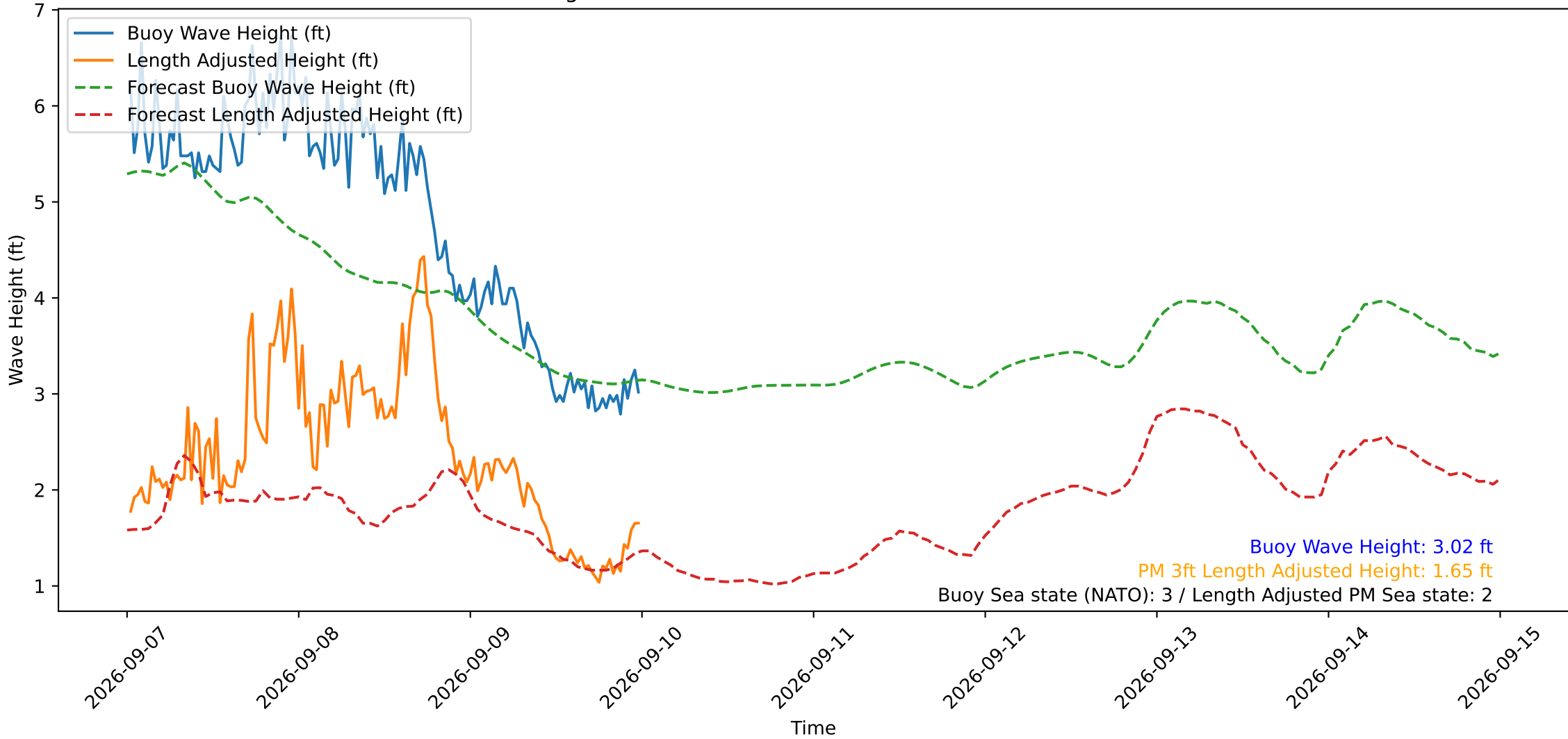
Wave Heights over Time for Red Beach at 2026-09-10 00:20:50
