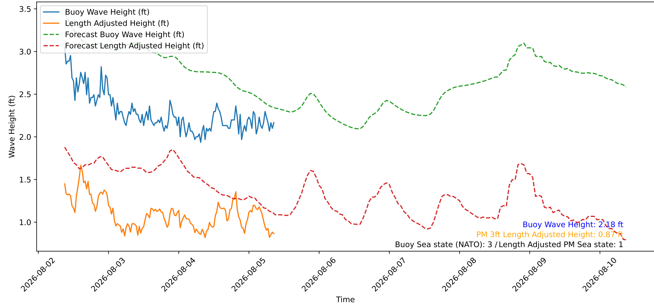
Wave Heights over Time for Green Beach at 2026-08-05 09:11:08
