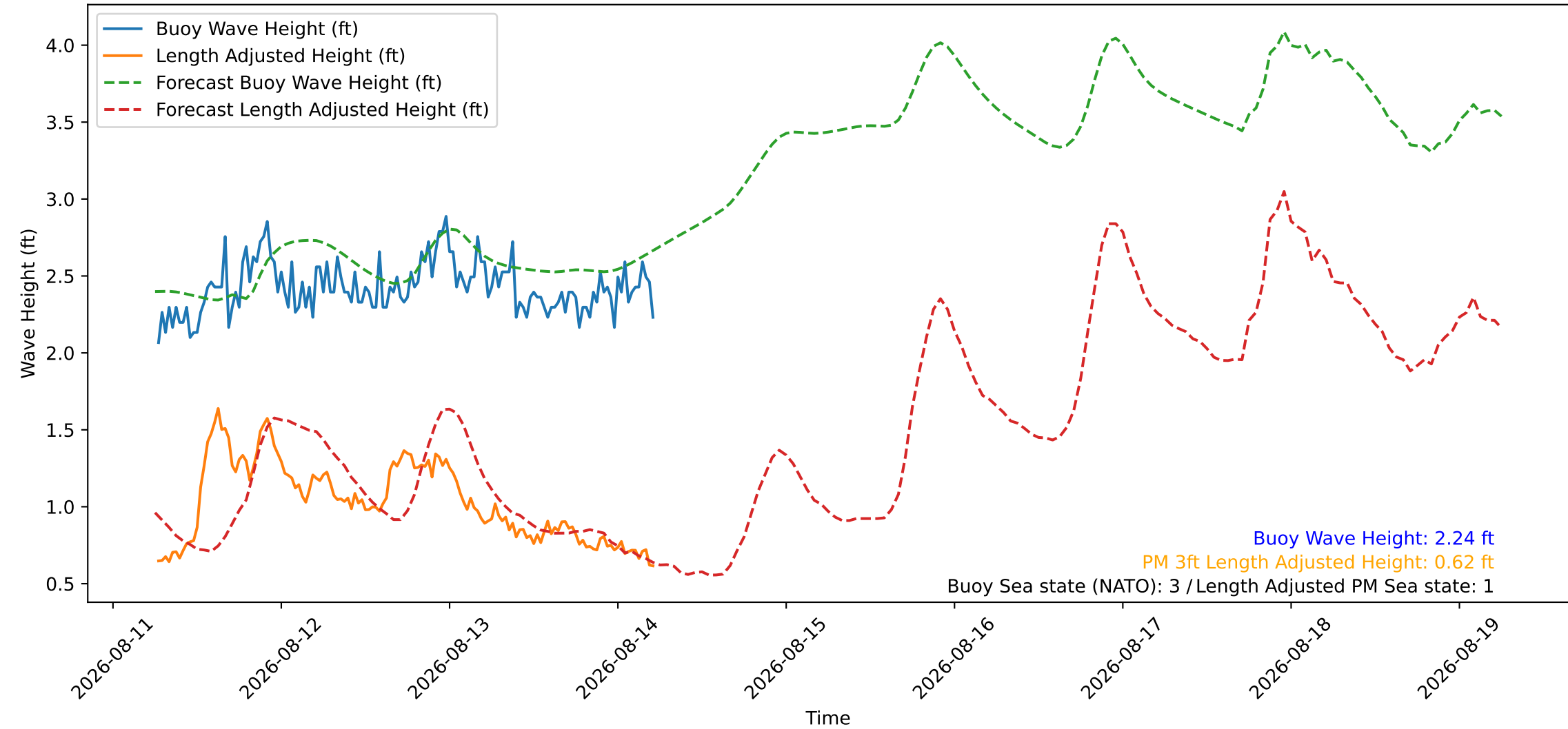
Wave Heights over Time for Red Beach at 2026-08-14 06:00:46
