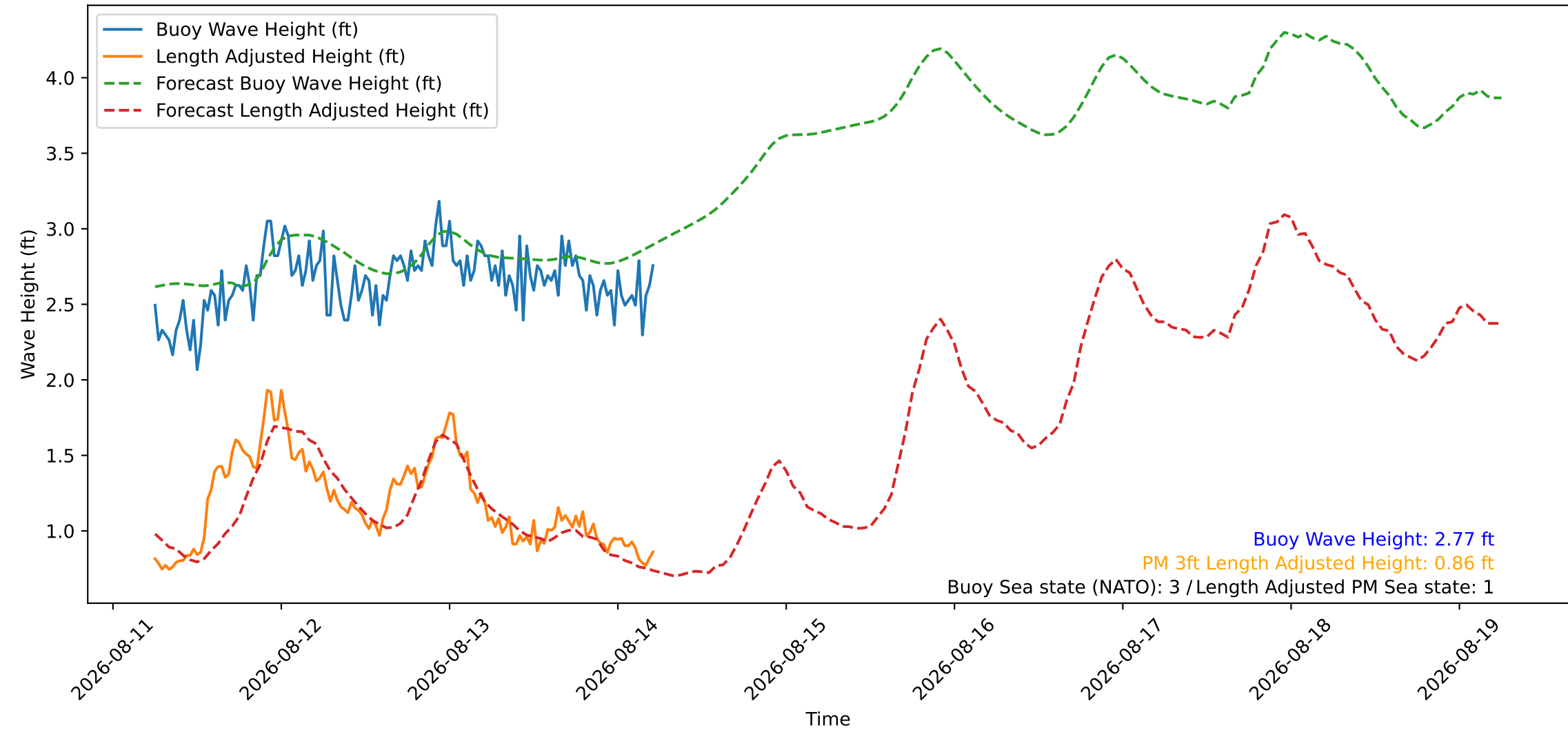
Wave Heights over Time for Oceanside Harbor at 2026-08-14 06:00:26
