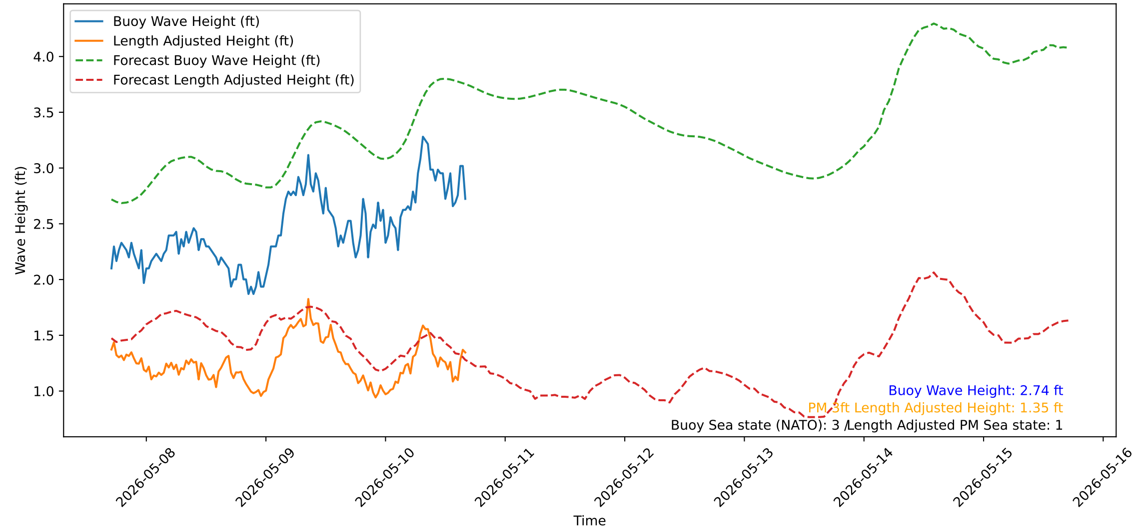
Wave Heights over Time for Oceanside Harbor at 2026-05-10 17:00:31
