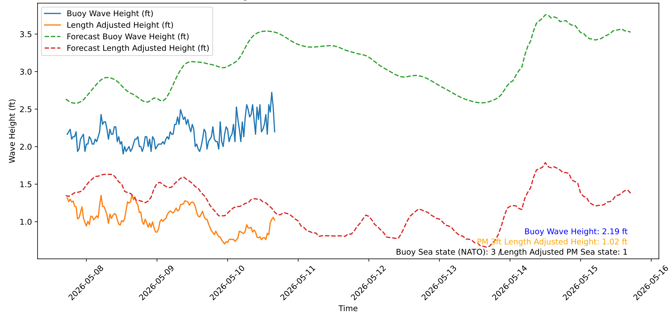
Wave Heights over Time for Red Beach at 2026-05-10 17:00:51
