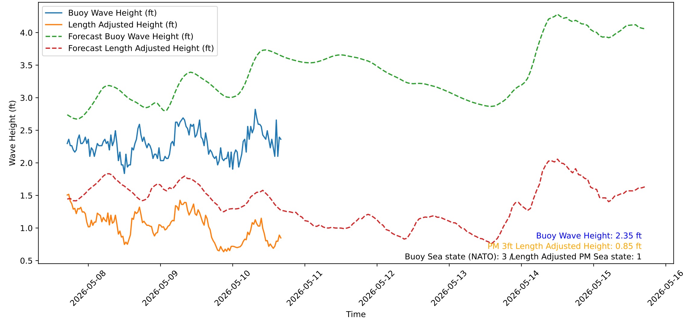
Wave Heights over Time for Green Beach at 2026-05-10 17:01:14
