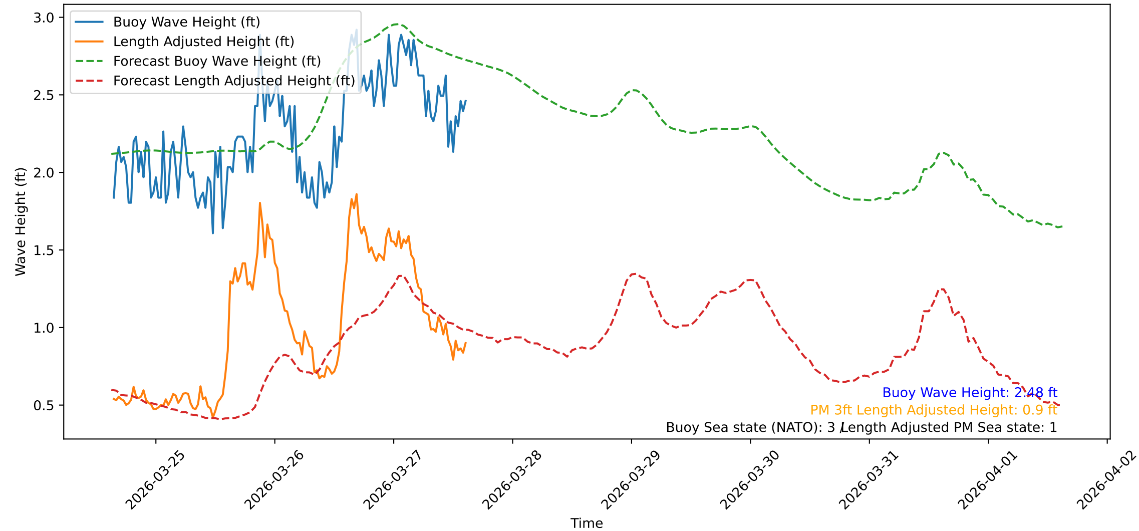
Wave Heights over Time for Oceanside Harbor at 2026-03-27 15:20:31
