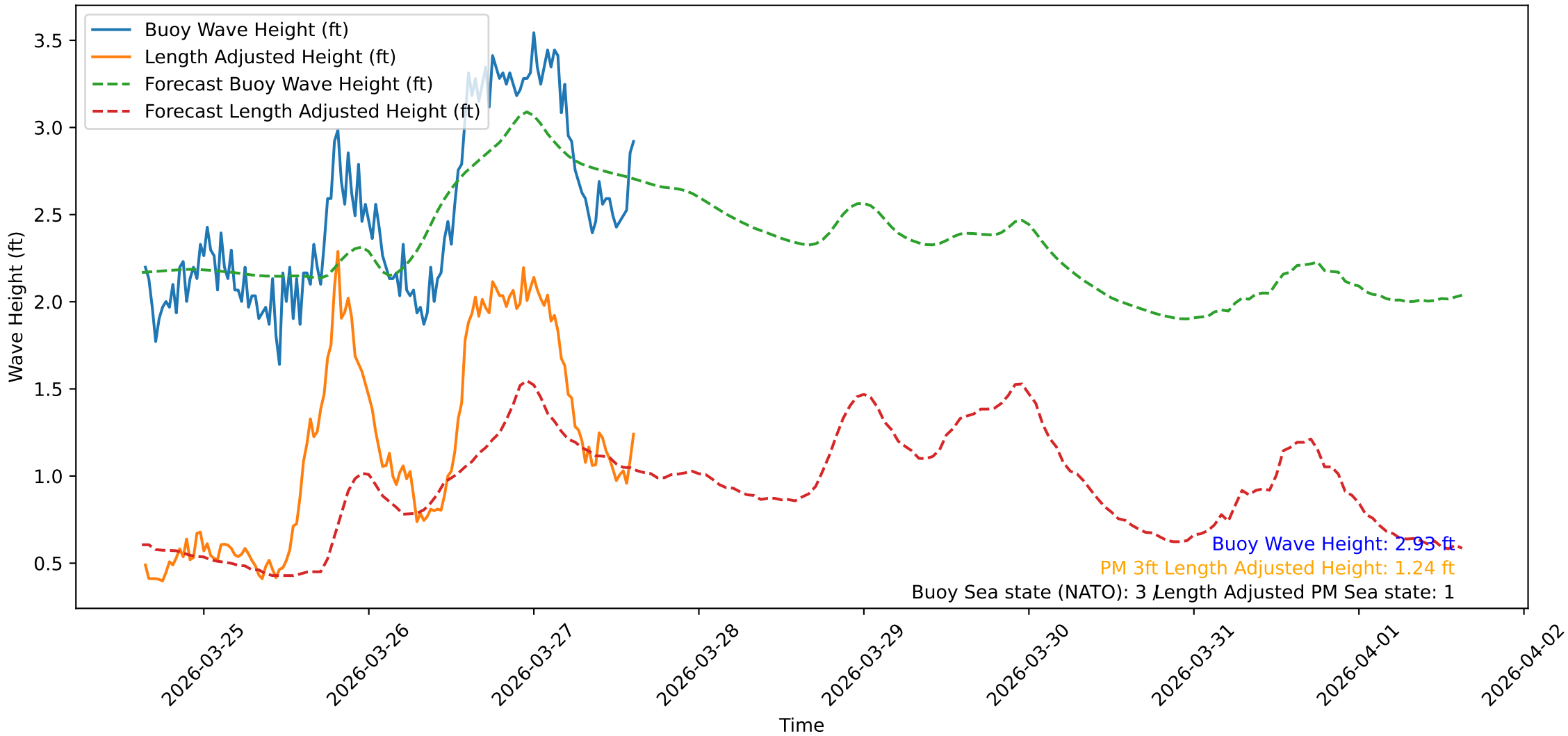
Wave Heights over Time for Green Beach at 2026-03-27 15:21:08
