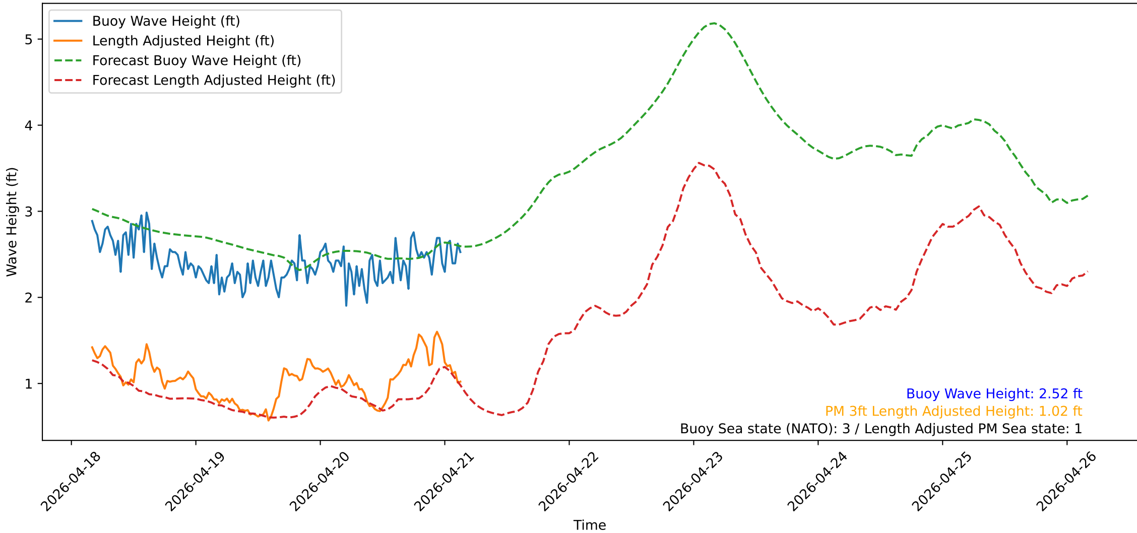
Wave Heights over Time for Oceanside Harbor at 2026-04-21 03:50:31
