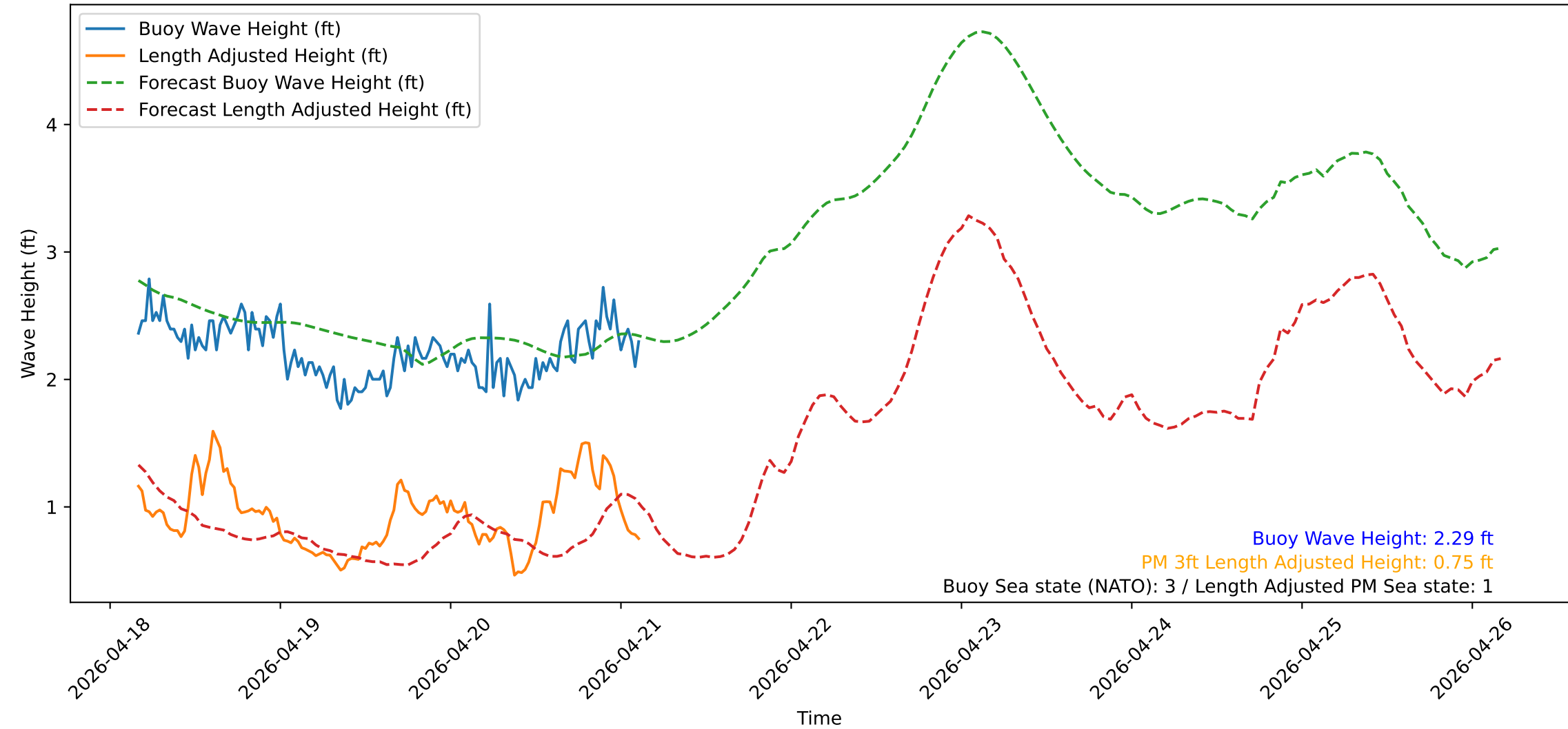
Wave Heights over Time for Red Beach at 2026-04-21 03:50:51
