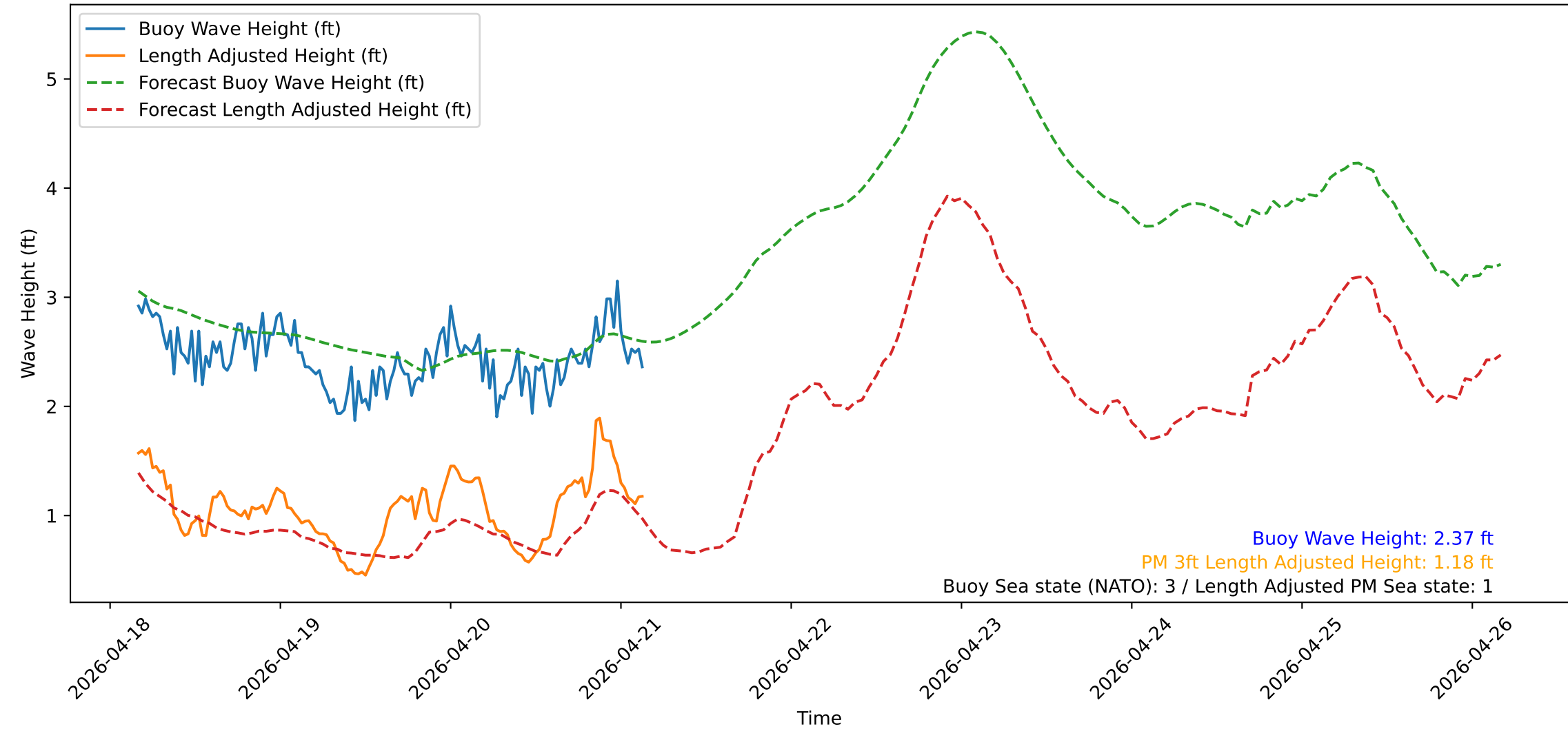
Wave Heights over Time for Green Beach at 2026-04-21 03:51:13
