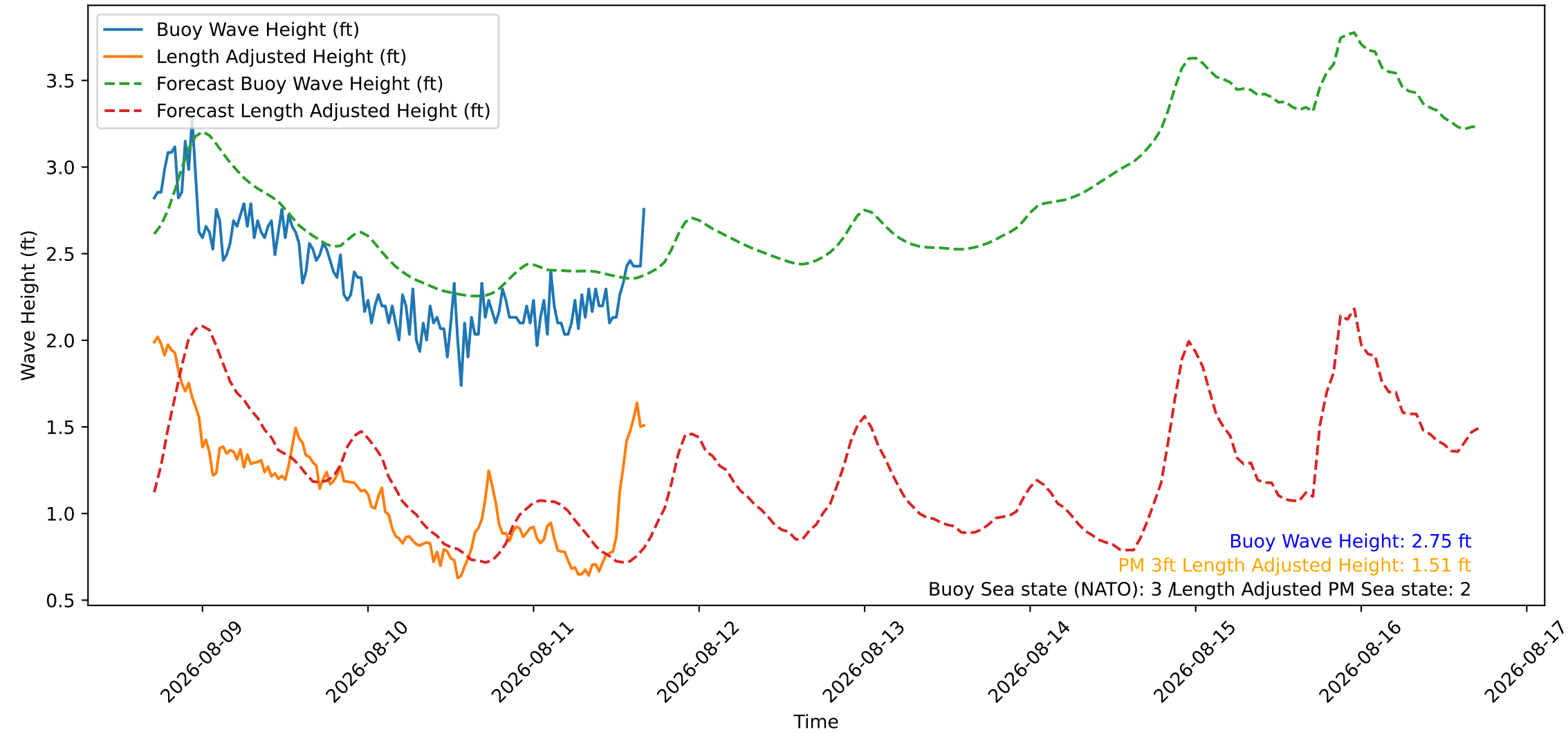
Wave Heights over Time for Red Beach at 2026-08-11 16:50:47
