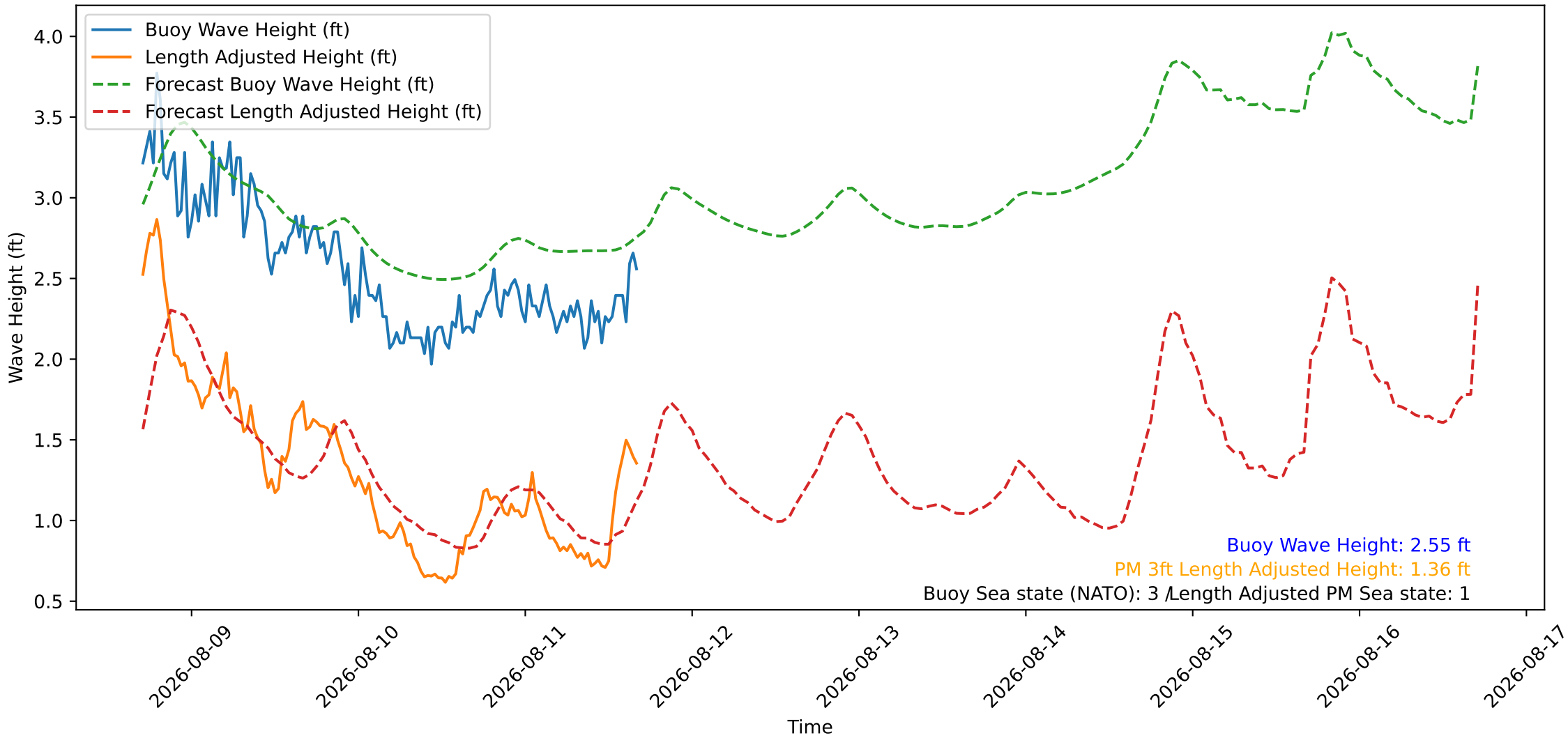
Wave Heights over Time for Green Beach at 2026-08-11 16:51:10
