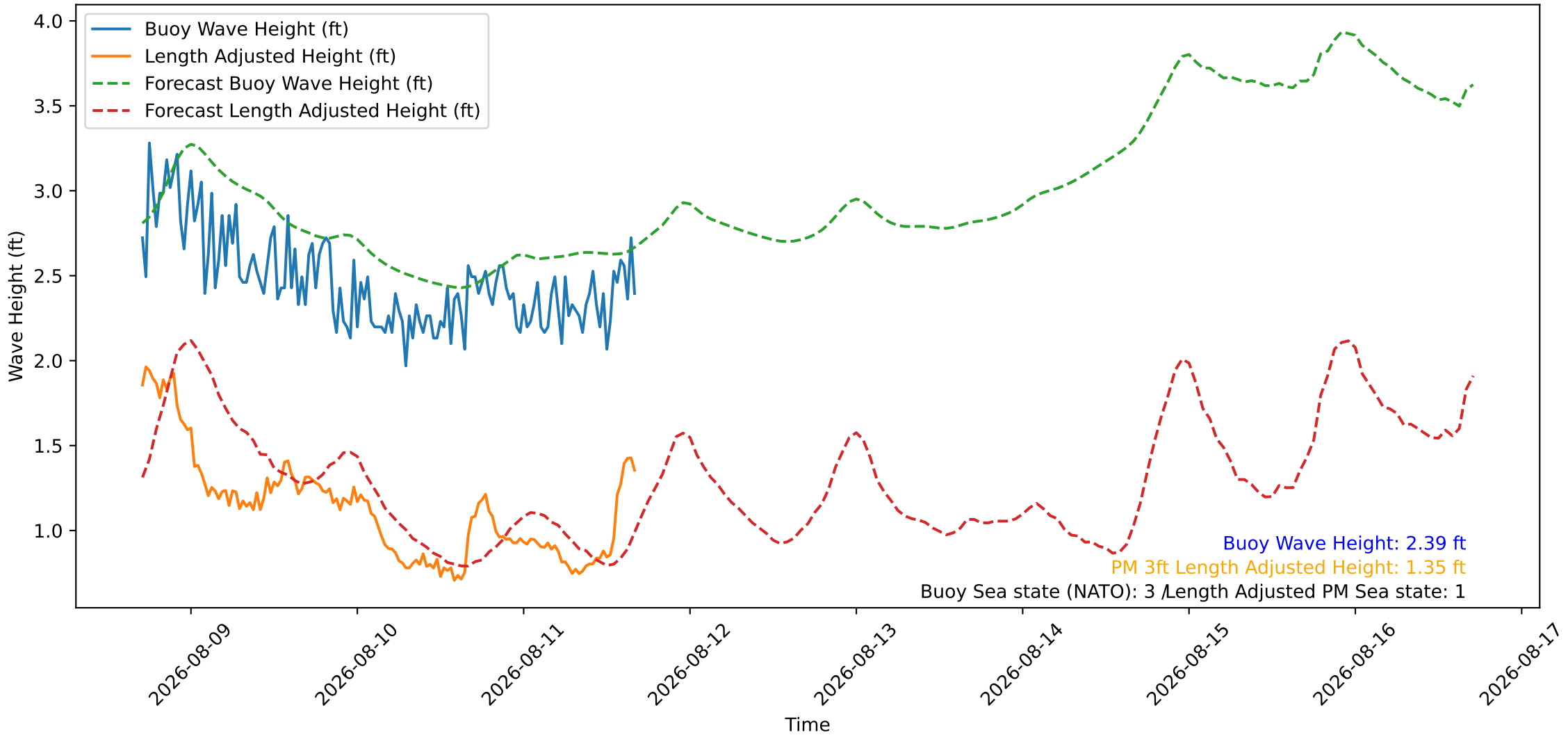
Wave Heights over Time for Oceanside Harbor at 2026-08-11 16:50:26
