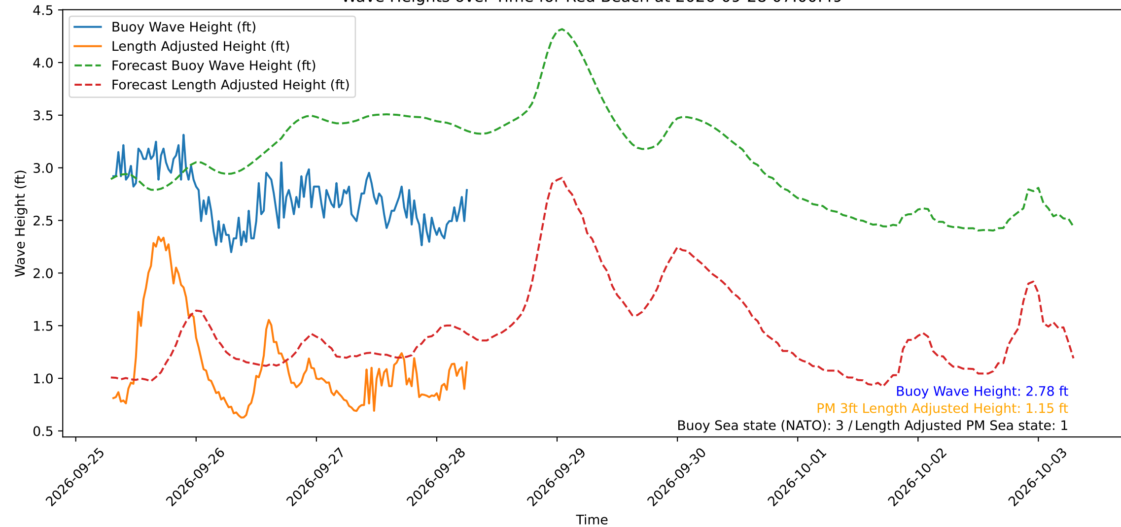
Wave Heights over Time for Red Beach at 2026-09-28 07:00:49
