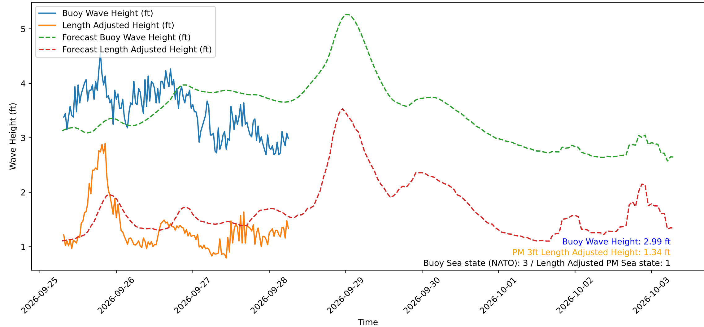
Wave Heights over Time for Green Beach at 2026-09-28 07:01:12
