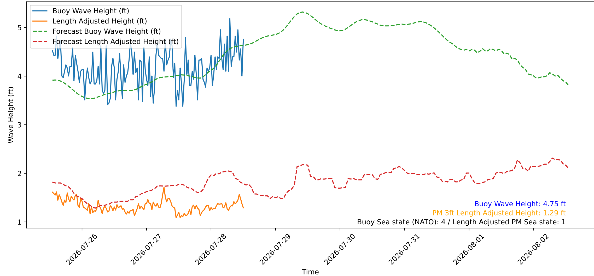
Wave Heights over Time for Green Beach at 2026-07-28 12:51:10
