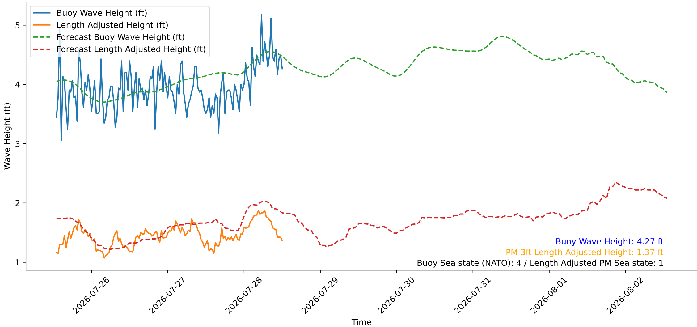
Wave Heights over Time for Oceanside Harbor at 2026-07-28 12:50:26
