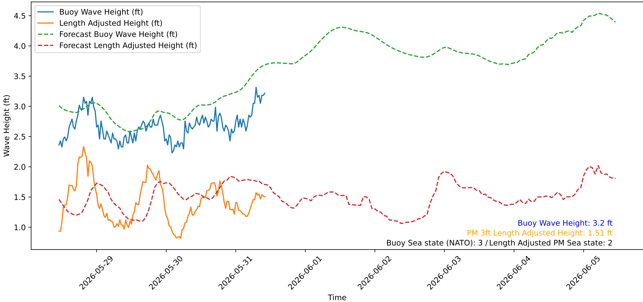
Wave Heights over Time for Red Beach at 2026-05-31 10:50:47
