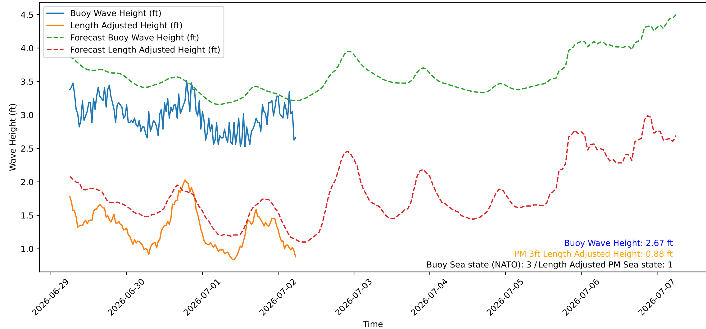
Wave Heights over Time for Green Beach at 2026-07-02 06:11:07
