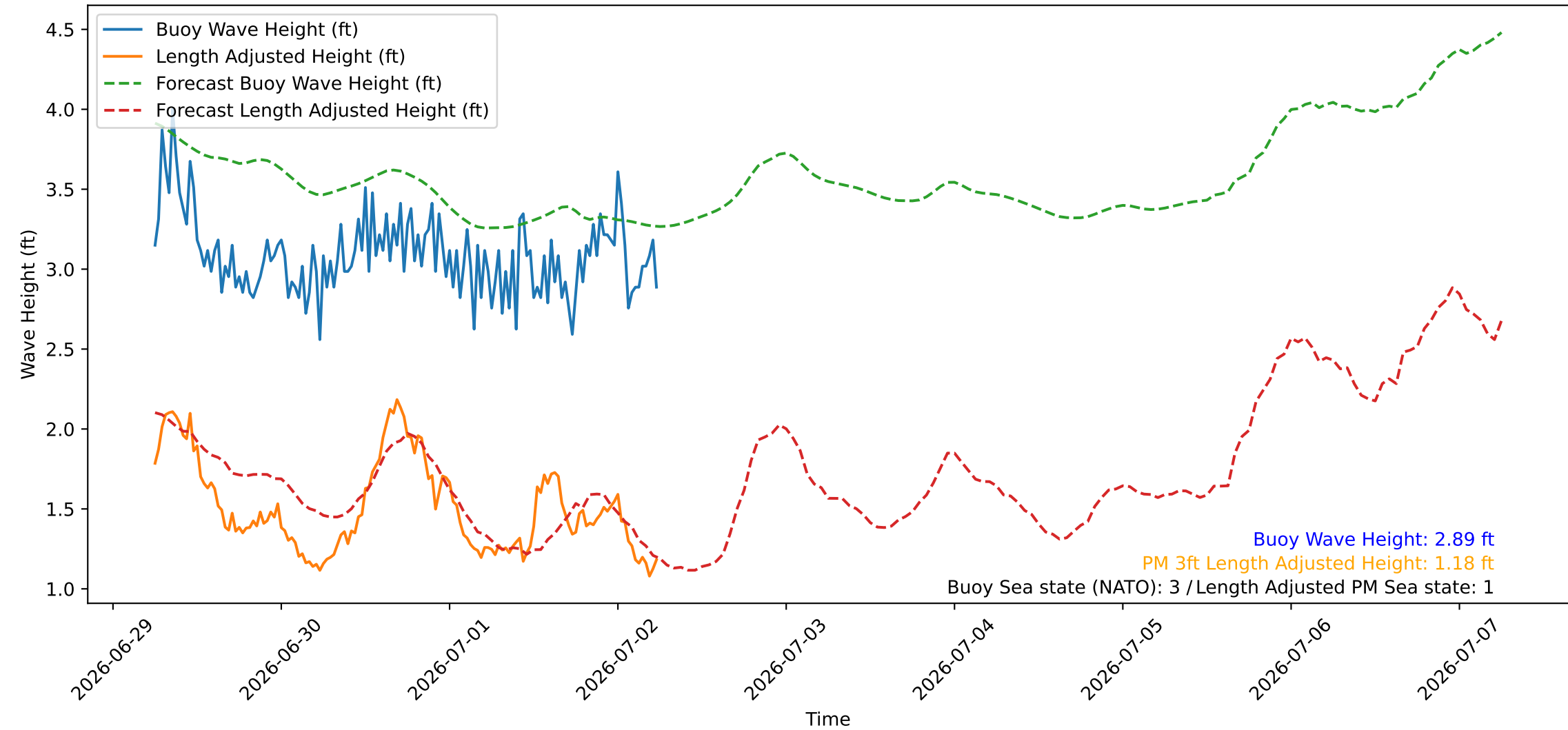
Wave Heights over Time for Oceanside Harbor at 2026-07-02 06:10:26
