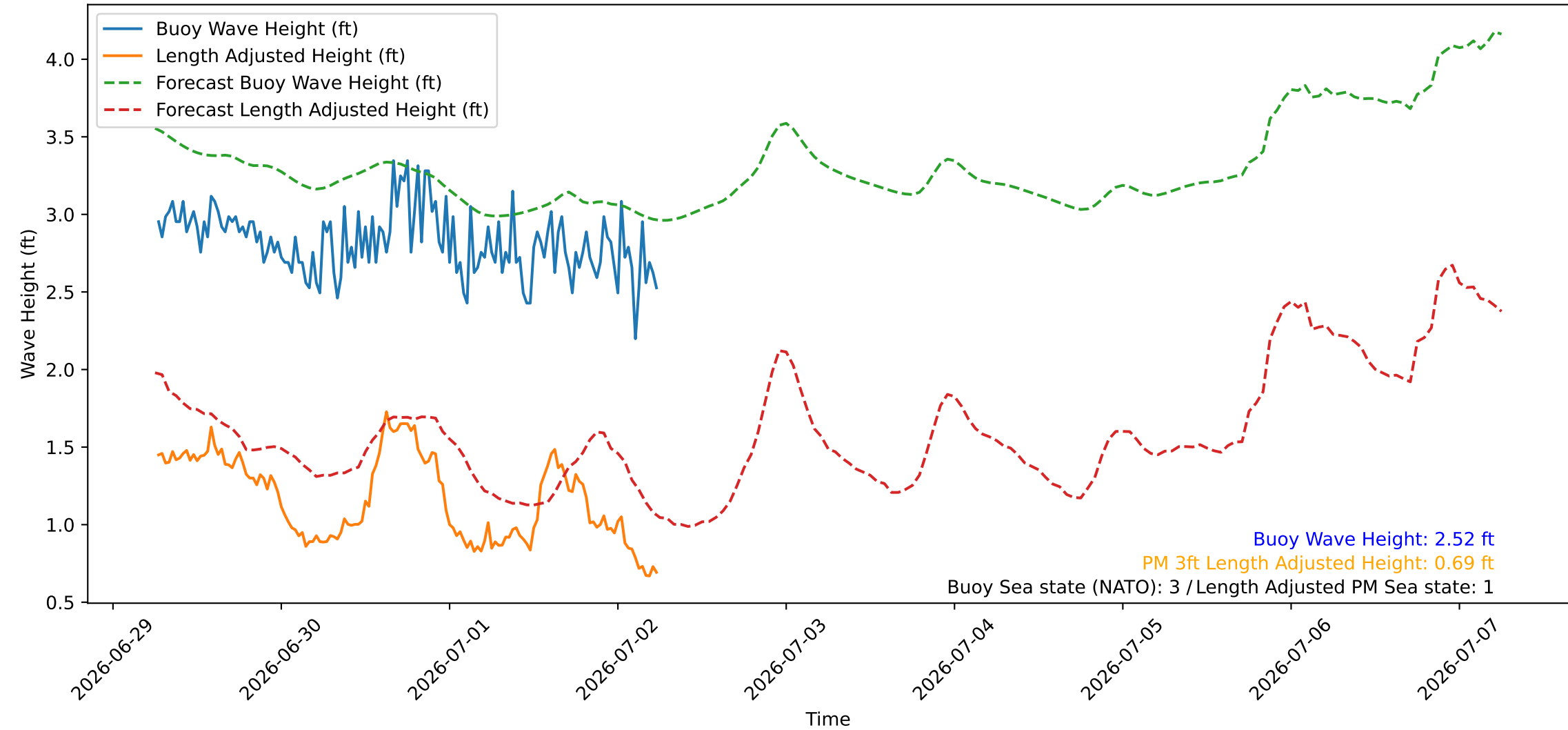
Wave Heights over Time for Red Beach at 2026-07-02 06:10:45
