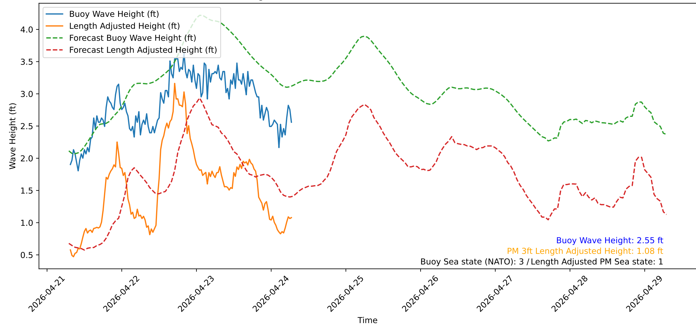
Wave Heights over Time for Red Beach at 2026-04-24 07:20:52
