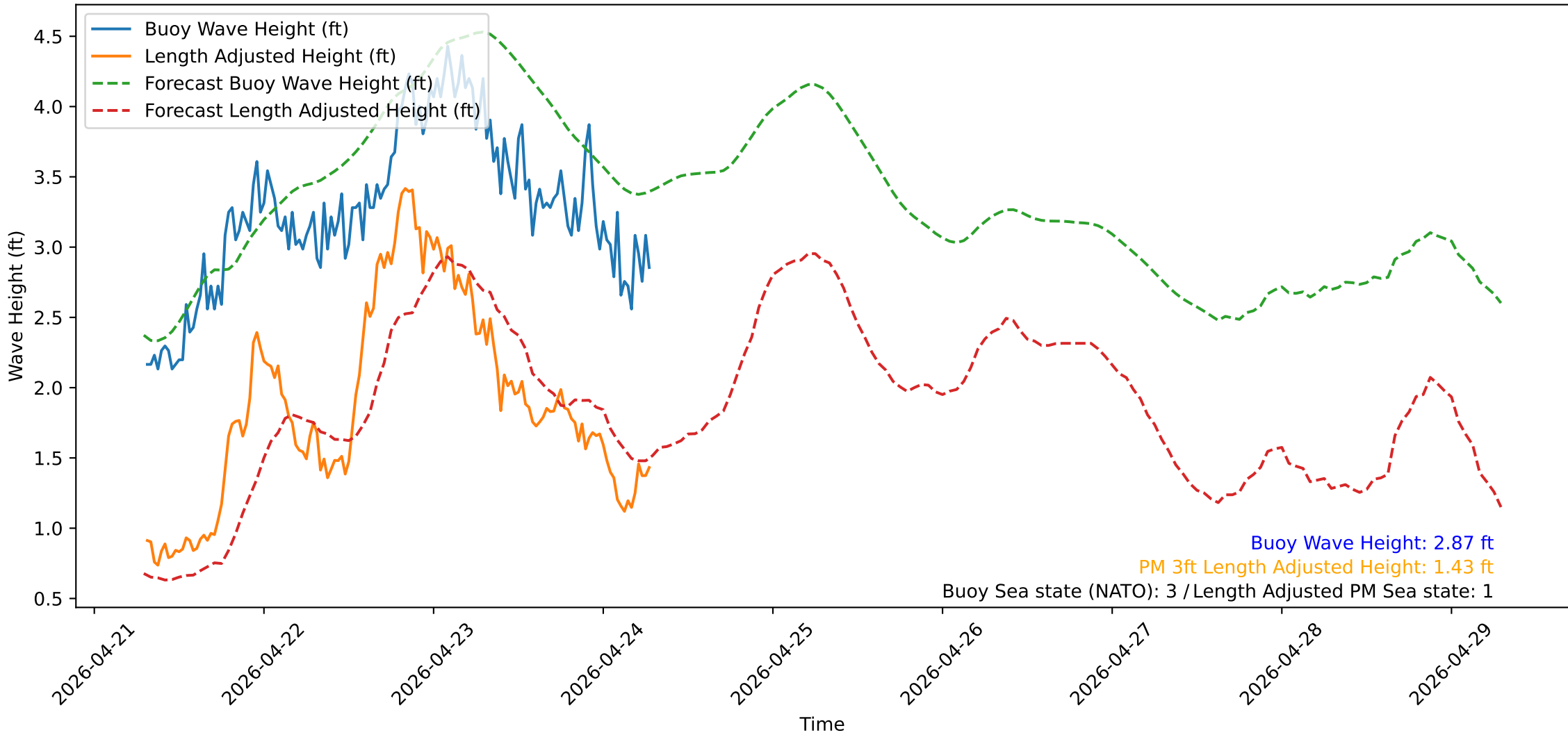
Wave Heights over Time for Oceanside Harbor at 2026-04-24 07:20:31
