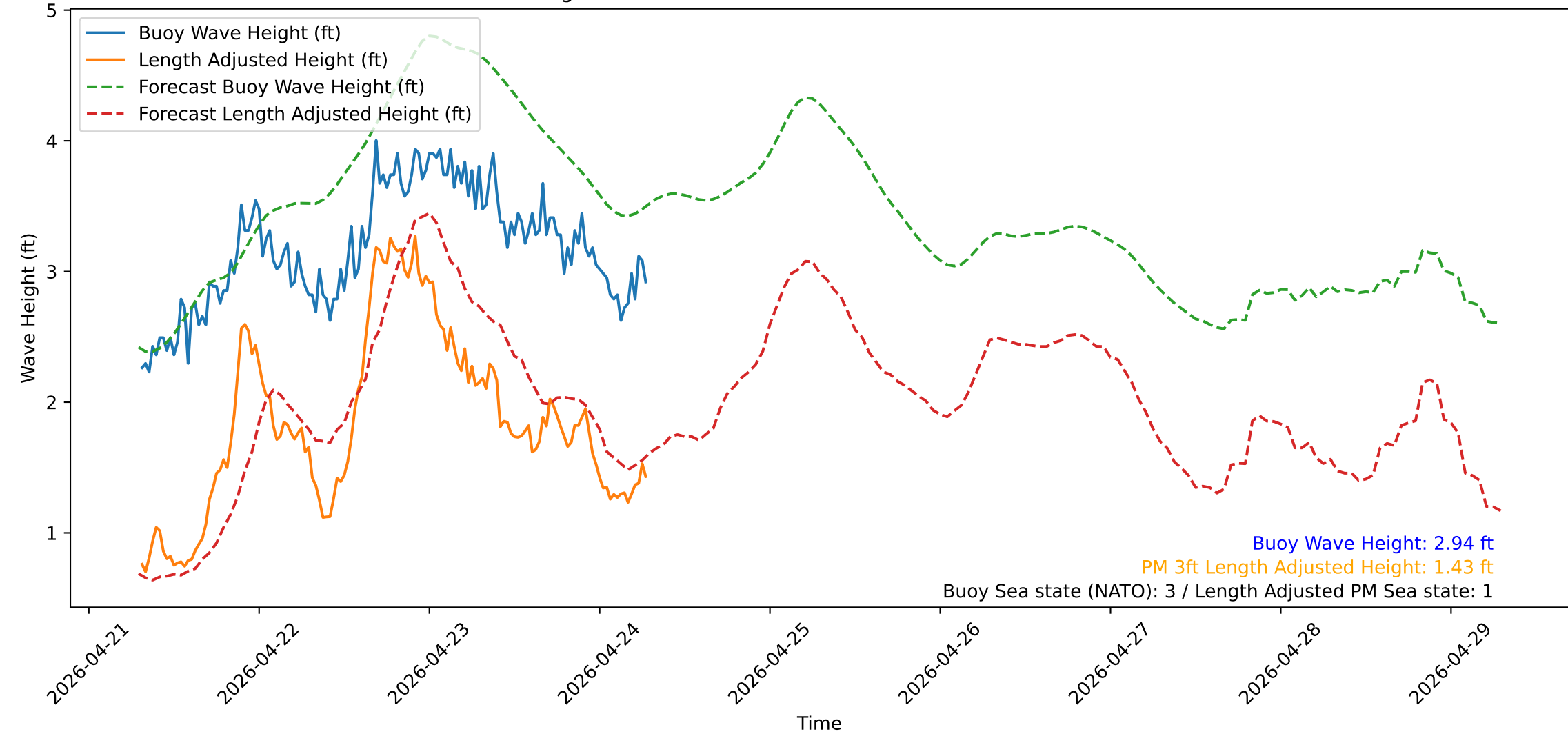
Wave Heights over Time for Green Beach at 2026-04-24 07:21:14
