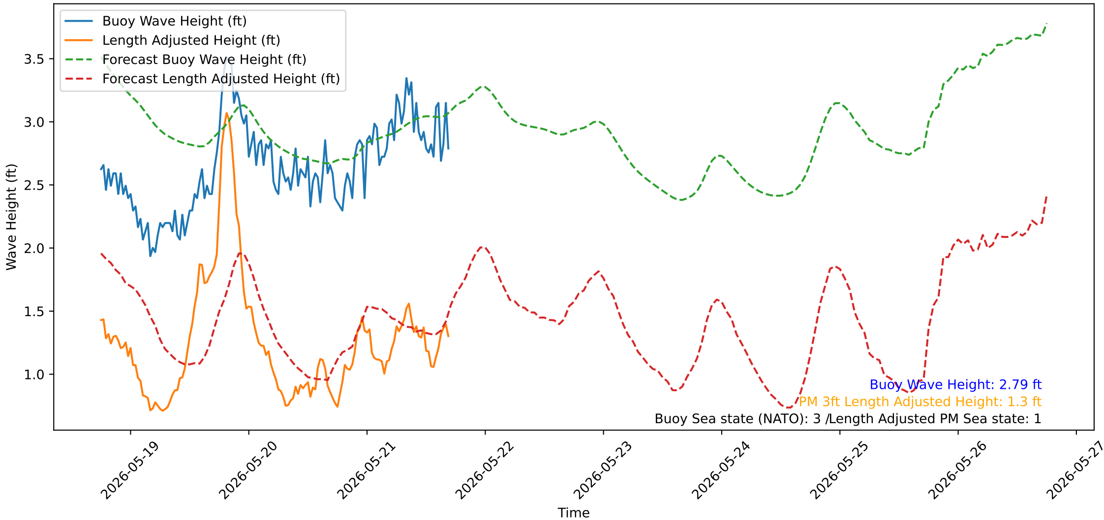
Wave Heights over Time for Red Beach at 2026-05-21 17:30:52
