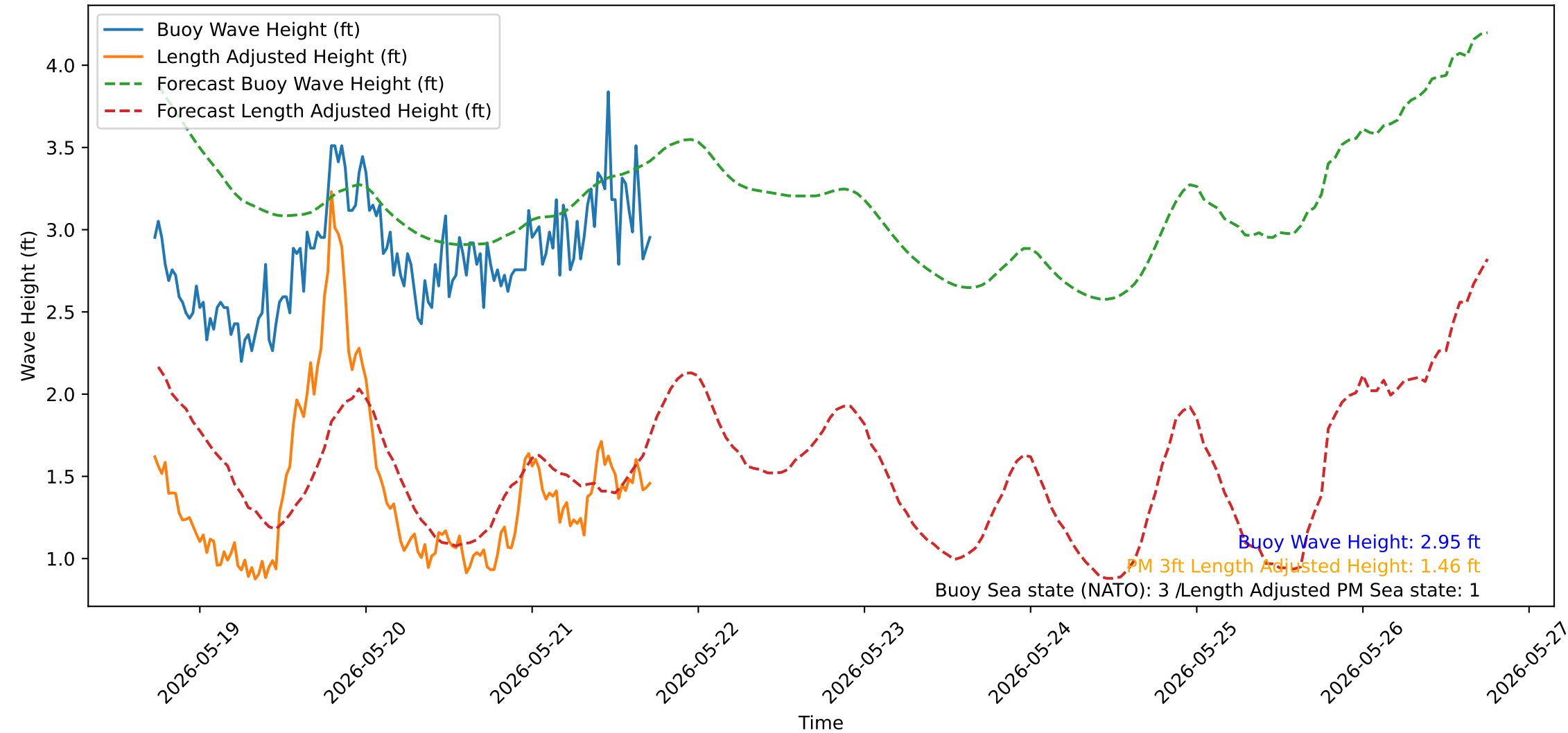
Wave Heights over Time for Oceanside Harbor at 2026-05-21 17:30:32
