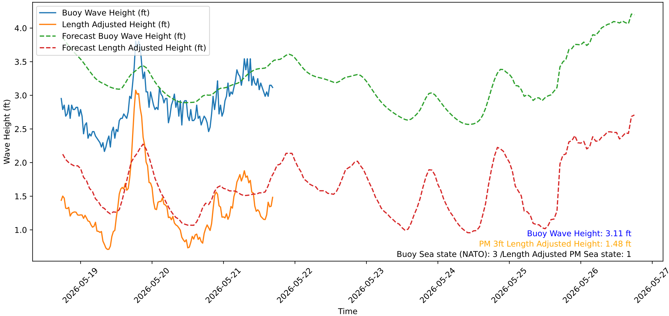
Wave Heights over Time for Green Beach at 2026-05-21 17:31:15
