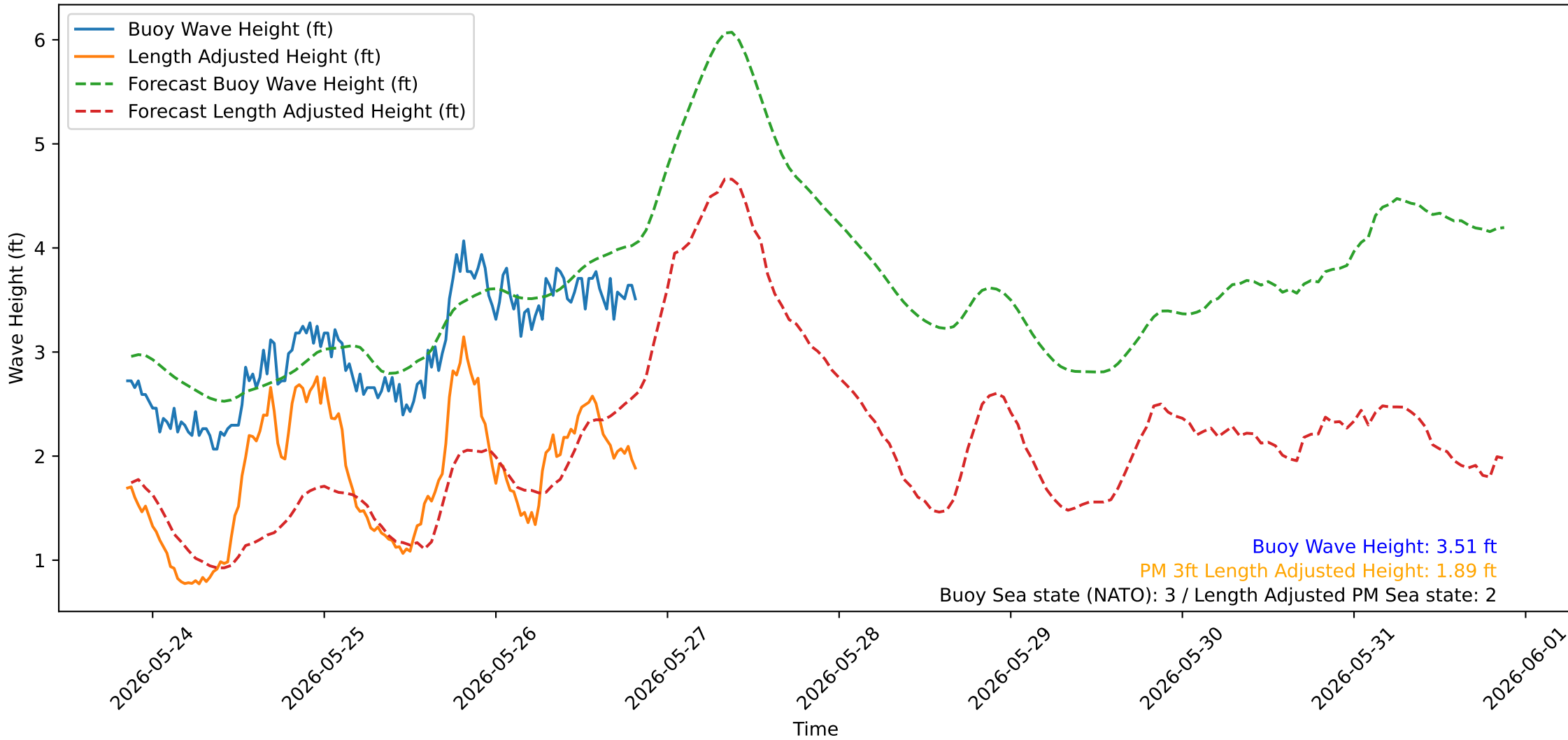
Wave Heights over Time for Green Beach at 2026-05-26 20:31:09
