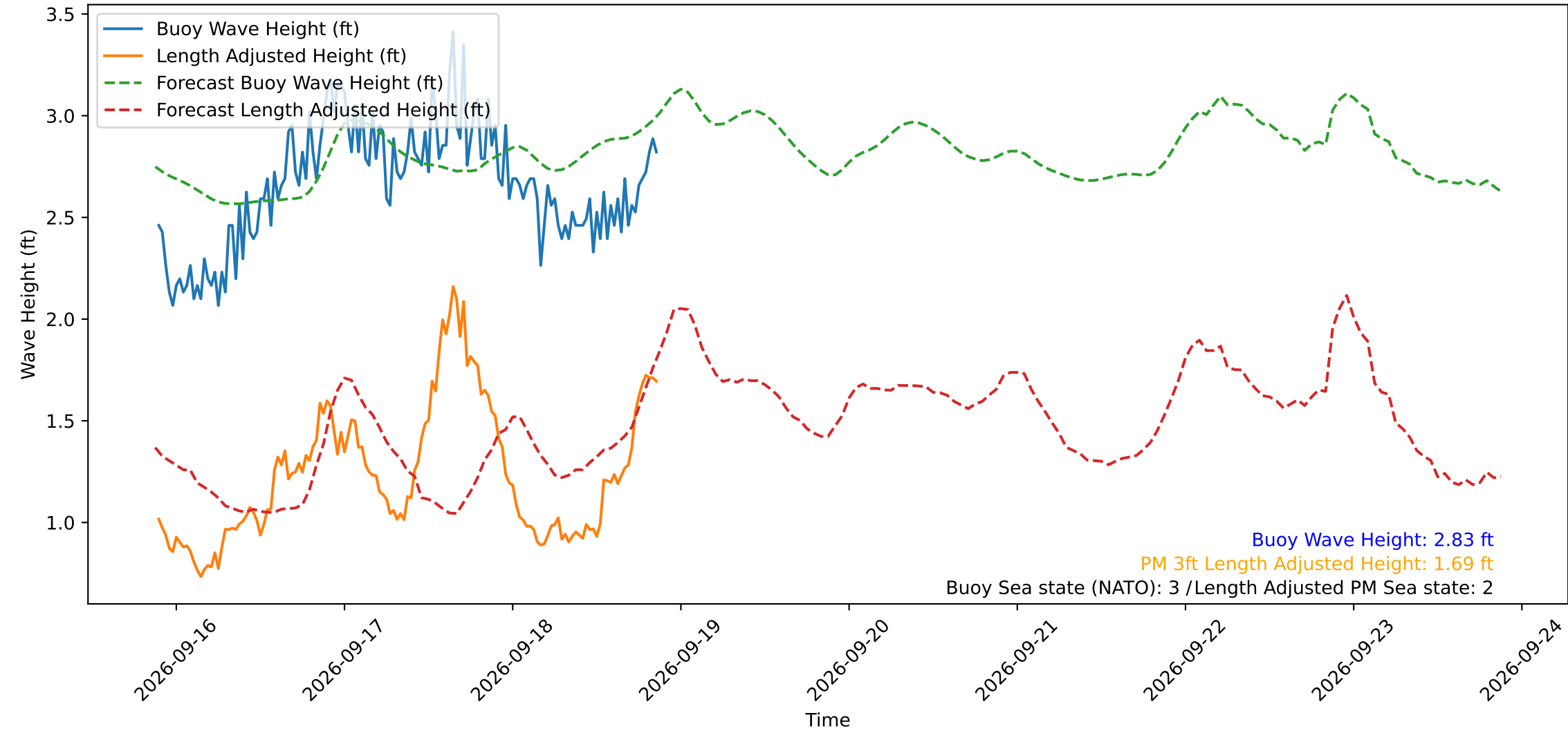
Wave Heights over Time for Red Beach at 2026-09-18 21:10:48
