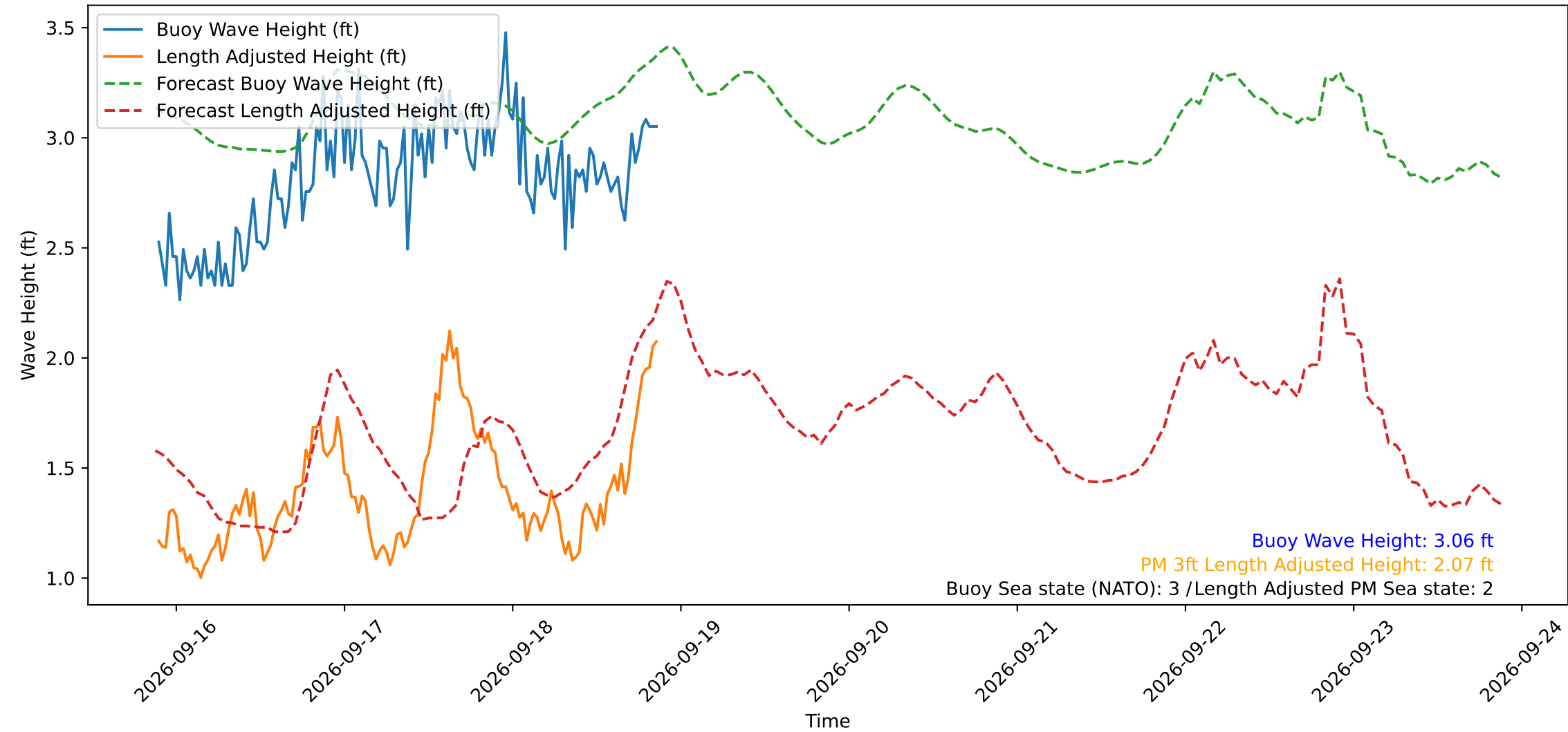
Wave Heights over Time for Green Beach at 2026-09-18 21:11:10
