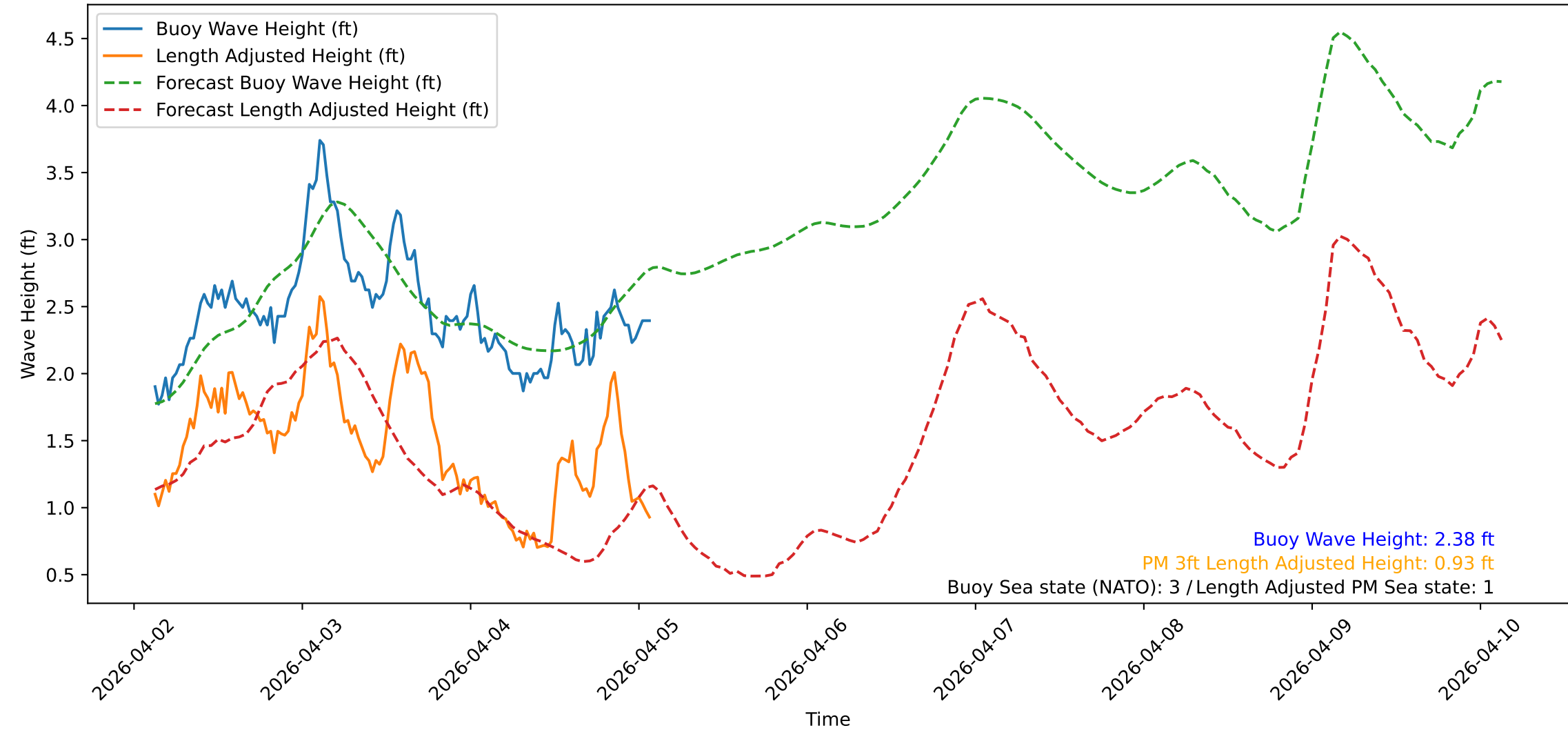
Wave Heights over Time for Red Beach at 2026-04-05 02:30:47
