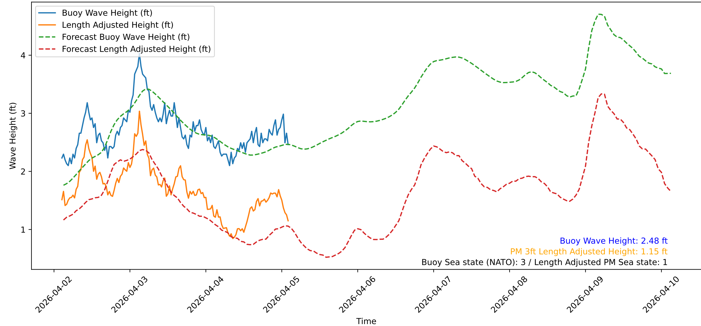
Wave Heights over Time for Oceanside Harbor at 2026-04-05 02:30:31
