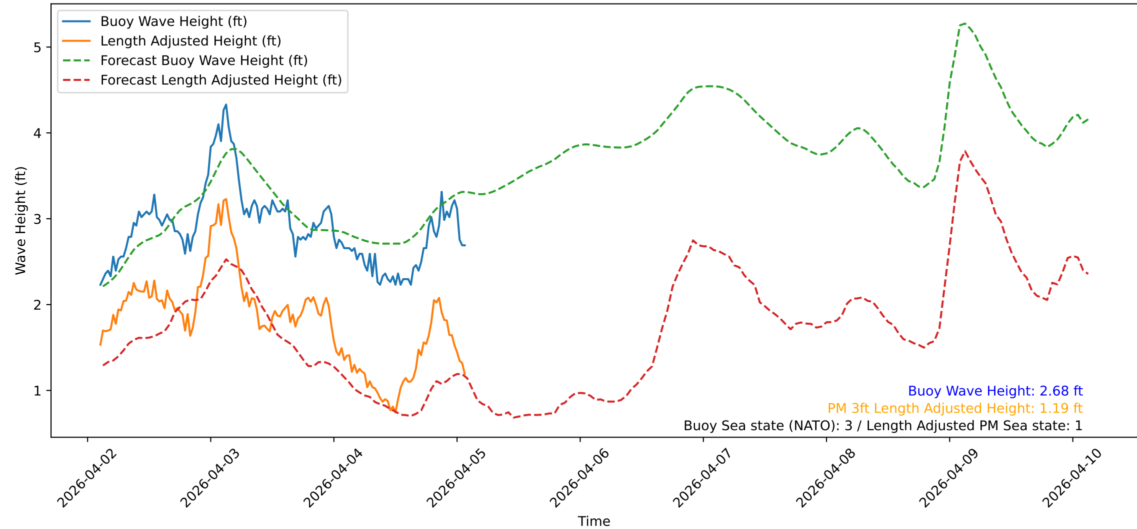
Wave Heights over Time for Green Beach at 2026-04-05 02:31:10
