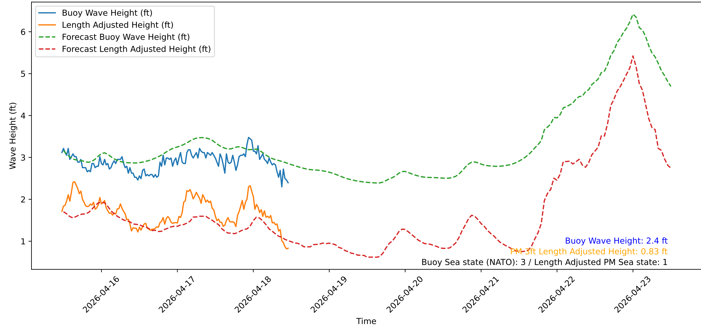
Wave Heights over Time for Green Beach at 2026-04-18 11:41:14
