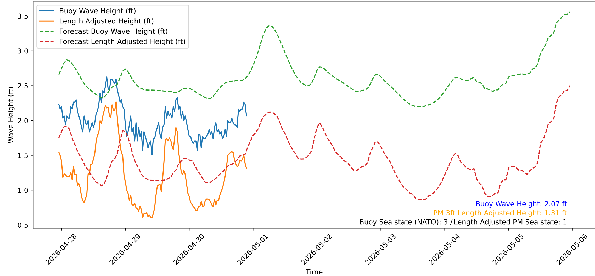
Wave Heights over Time for Red Beach at 2026-04-30 22:30:51
