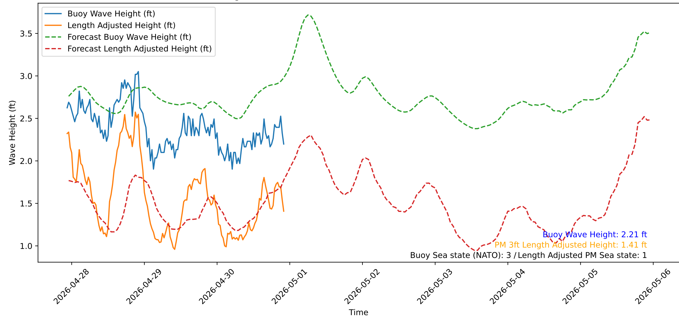
Wave Heights over Time for Oceanside Harbor at 2026-04-30 22:30:32
